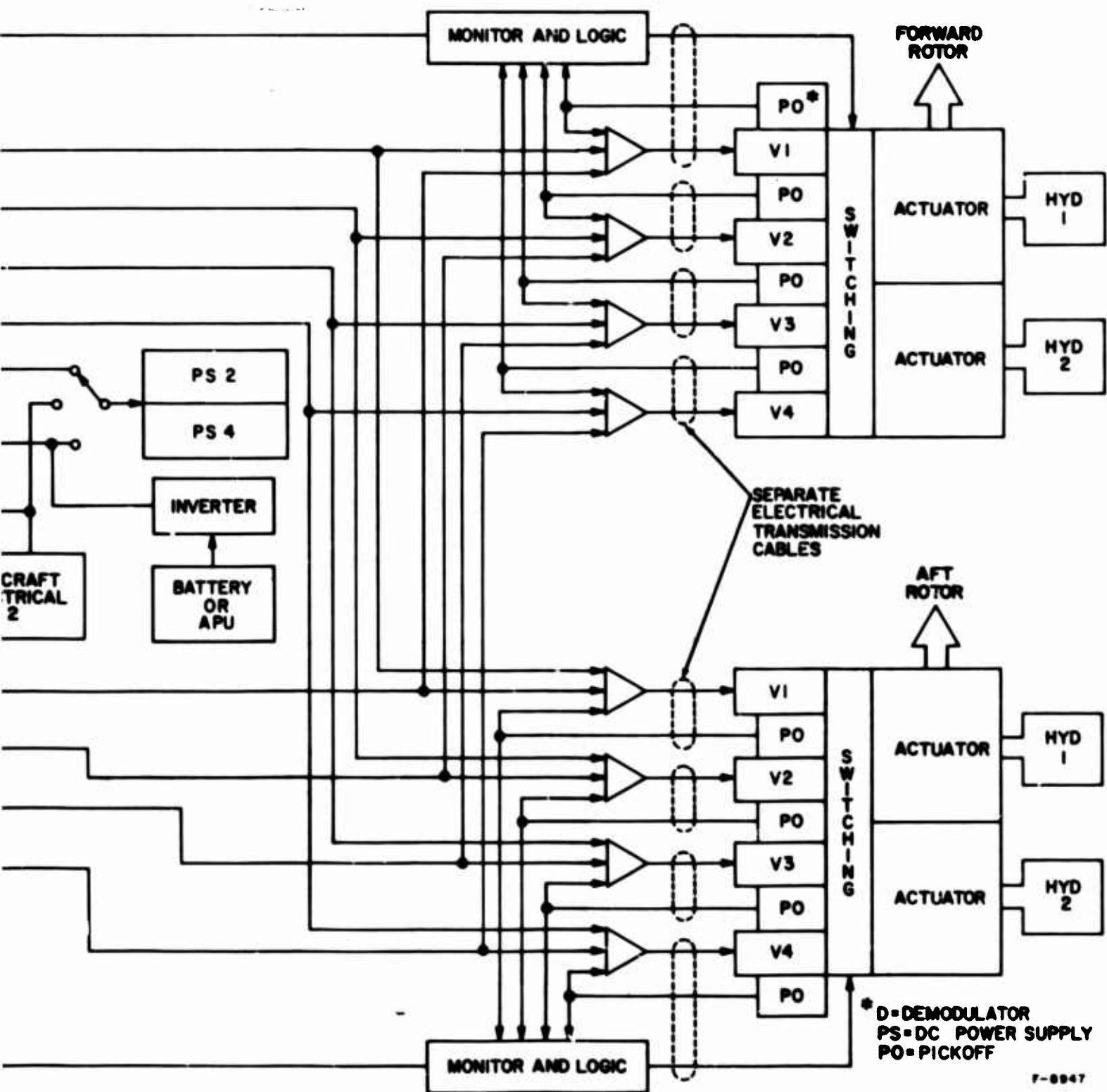
Figure 91 Fly-By-Wire Implementation Longitudinal Axis
