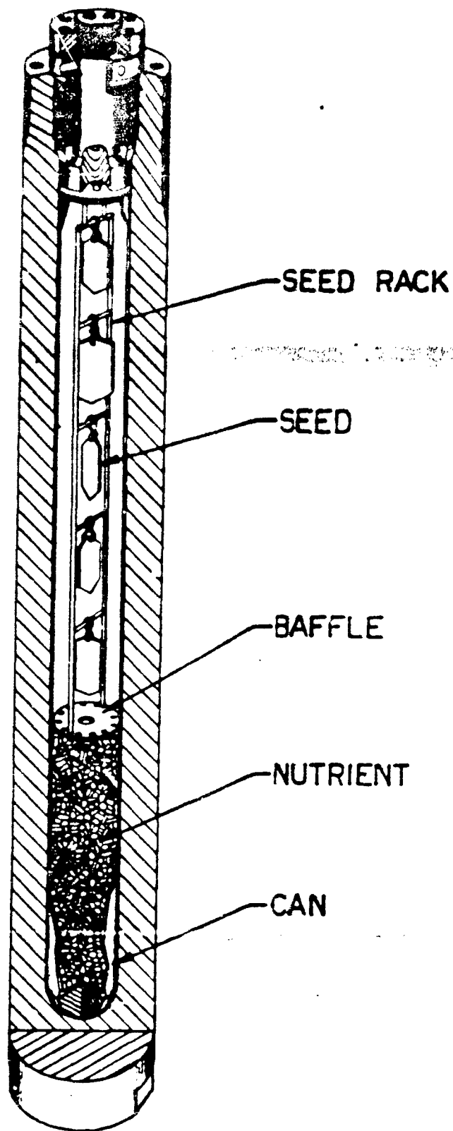
Figure 1 - Hydrothermal System
