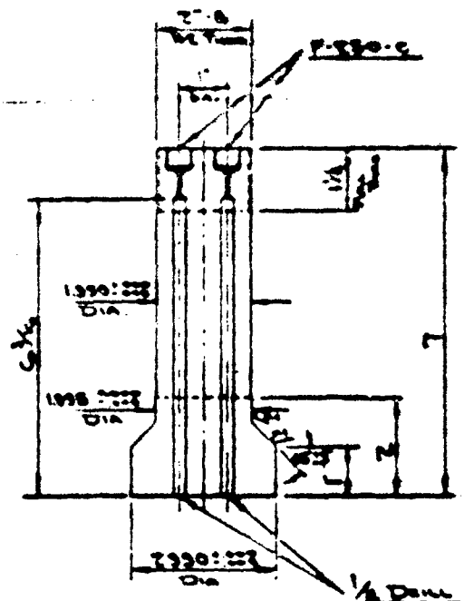
COVER - ITEM #2
