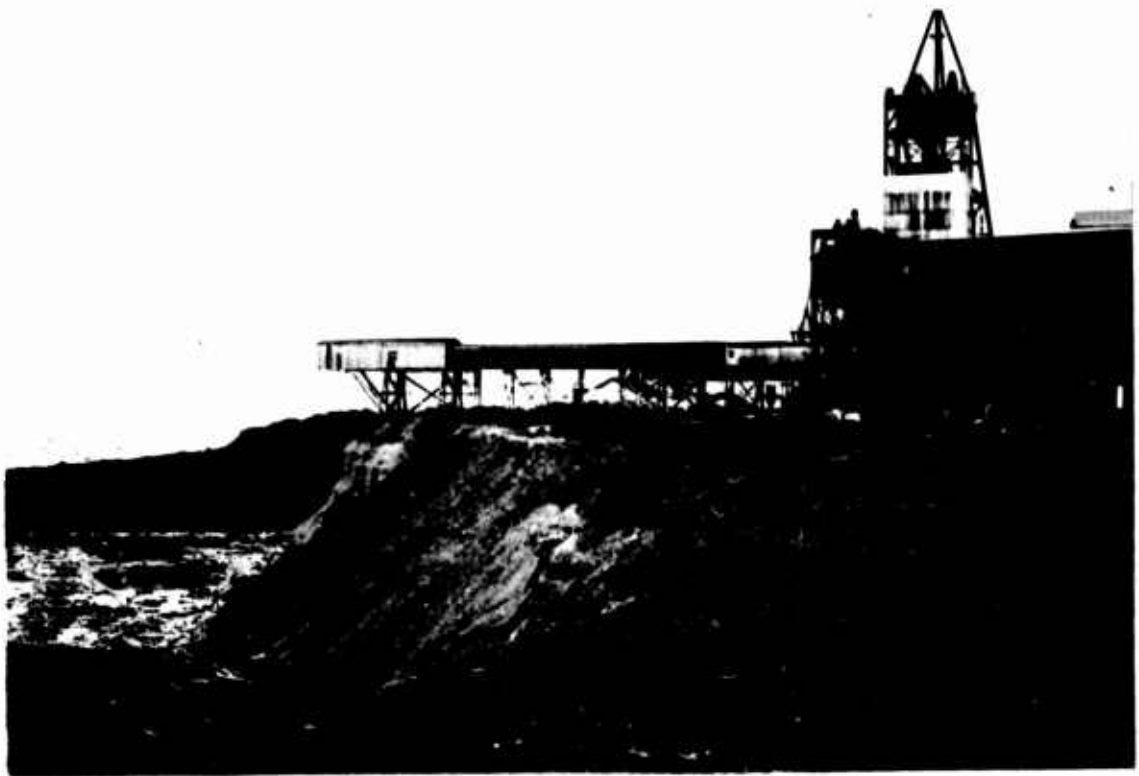
FIG. 12. Vertical Shaft at the Shore Line for Entry into Submarine Coal Mine Workings at Cape Breton.
