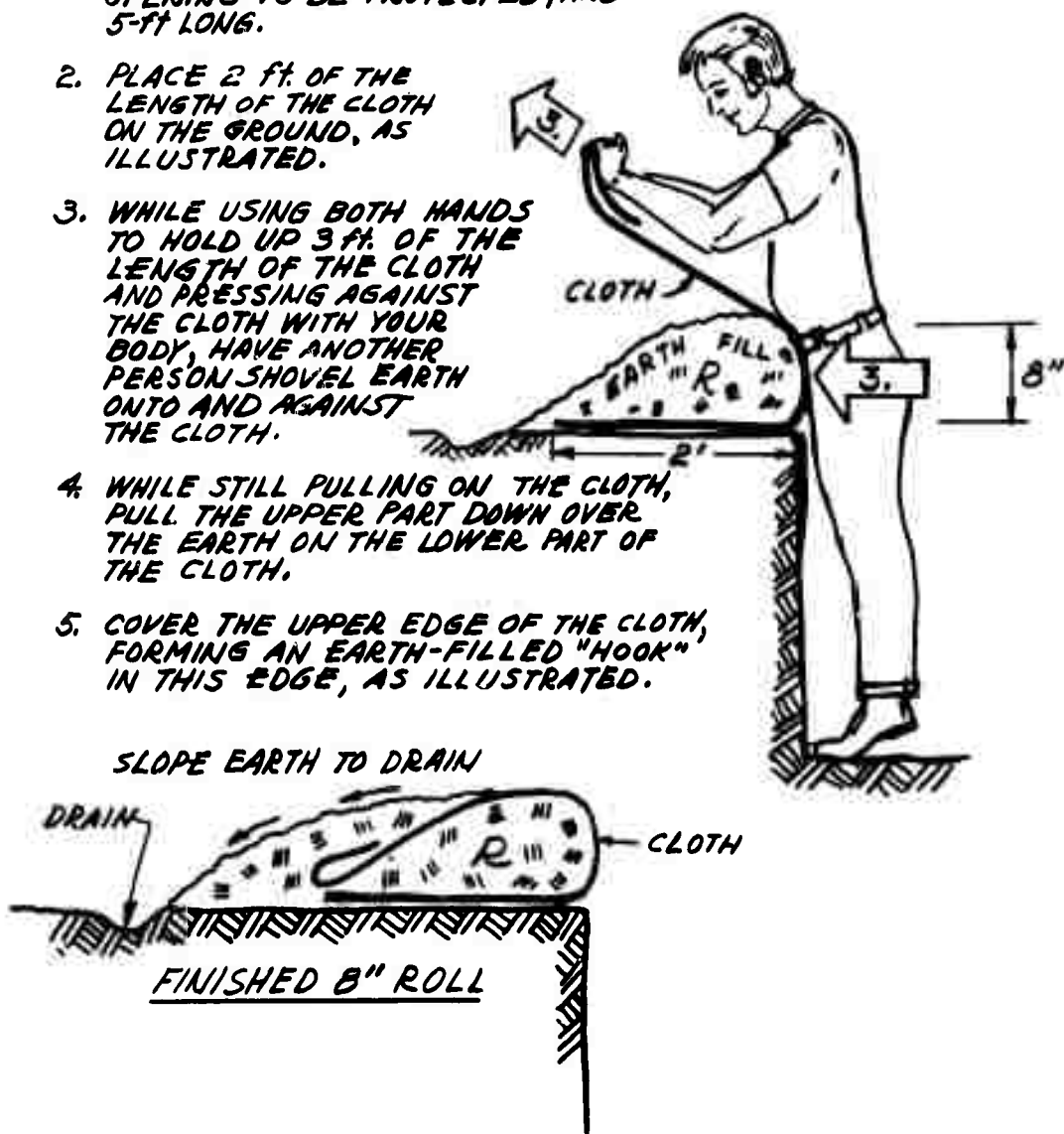
Fig. A-14.2. Door-Over-Trench Shelter, Making a "Roll."
