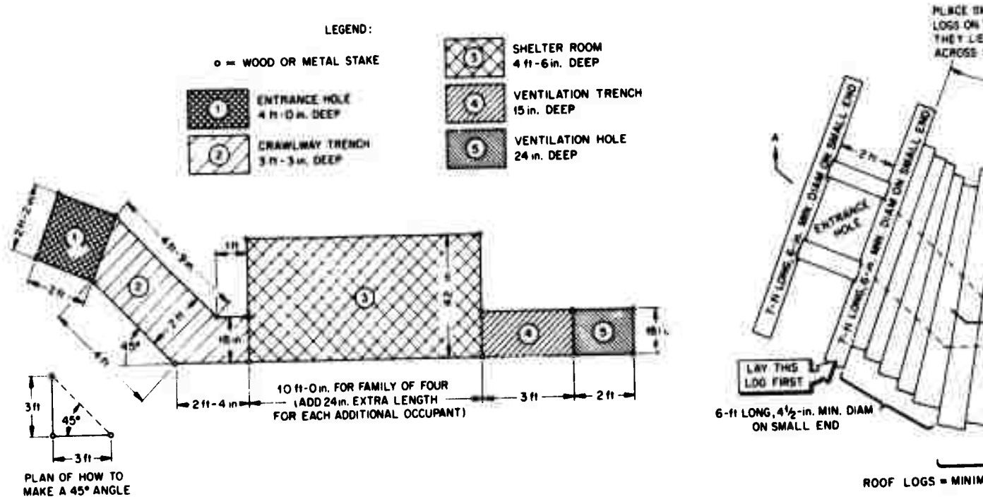
PLAN FOR STAKING OUT TRENCH ON TOP OF GROUND (SEE LEGEND FOR 5 DIFFERENT DEPTHS OF TRENCH)
