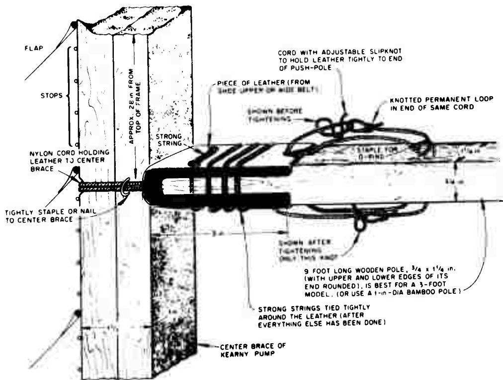
Fig. B-24. Push-pole flexible connection.
