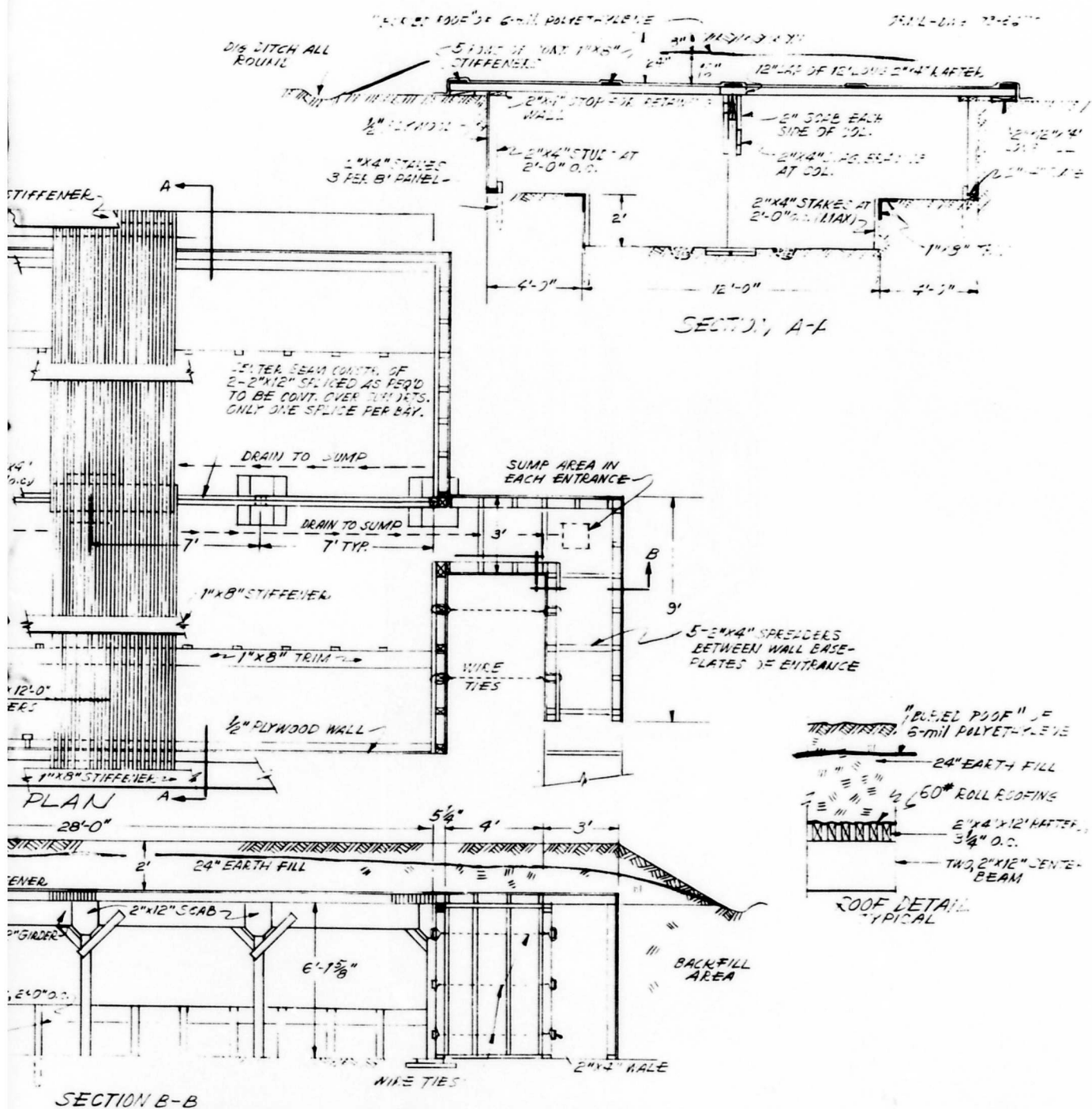
Fig. A-11.1. Wood Grate Roof Underground, Plans and Section.
