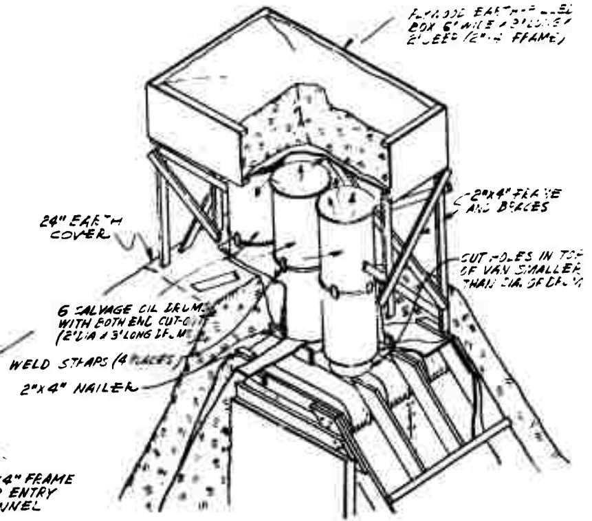
OIL DRUM VENT STACKS
