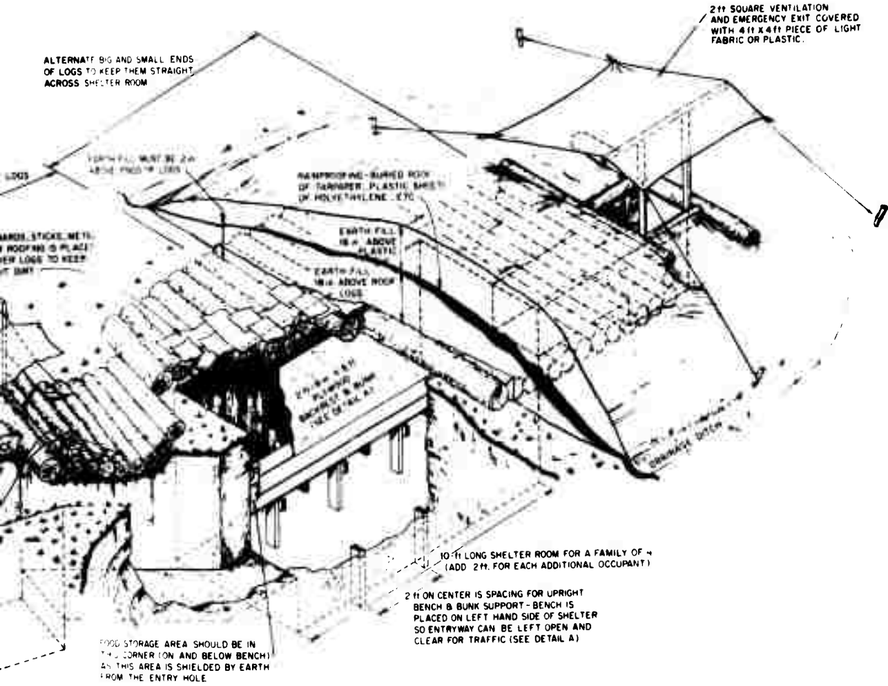
Trench Shelter, Pictorial View.
