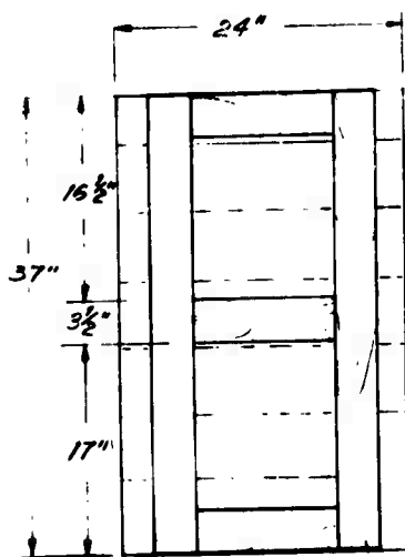
INSIDE FACE OF OUTER VERT. SECTION OF EXIT TUNNEL, MARK ④
