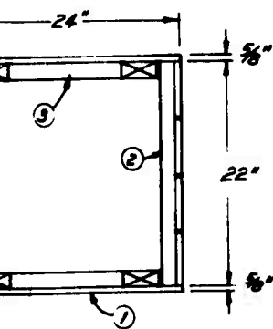
CROSS SECTION OF HORIZONTAL EXIT
