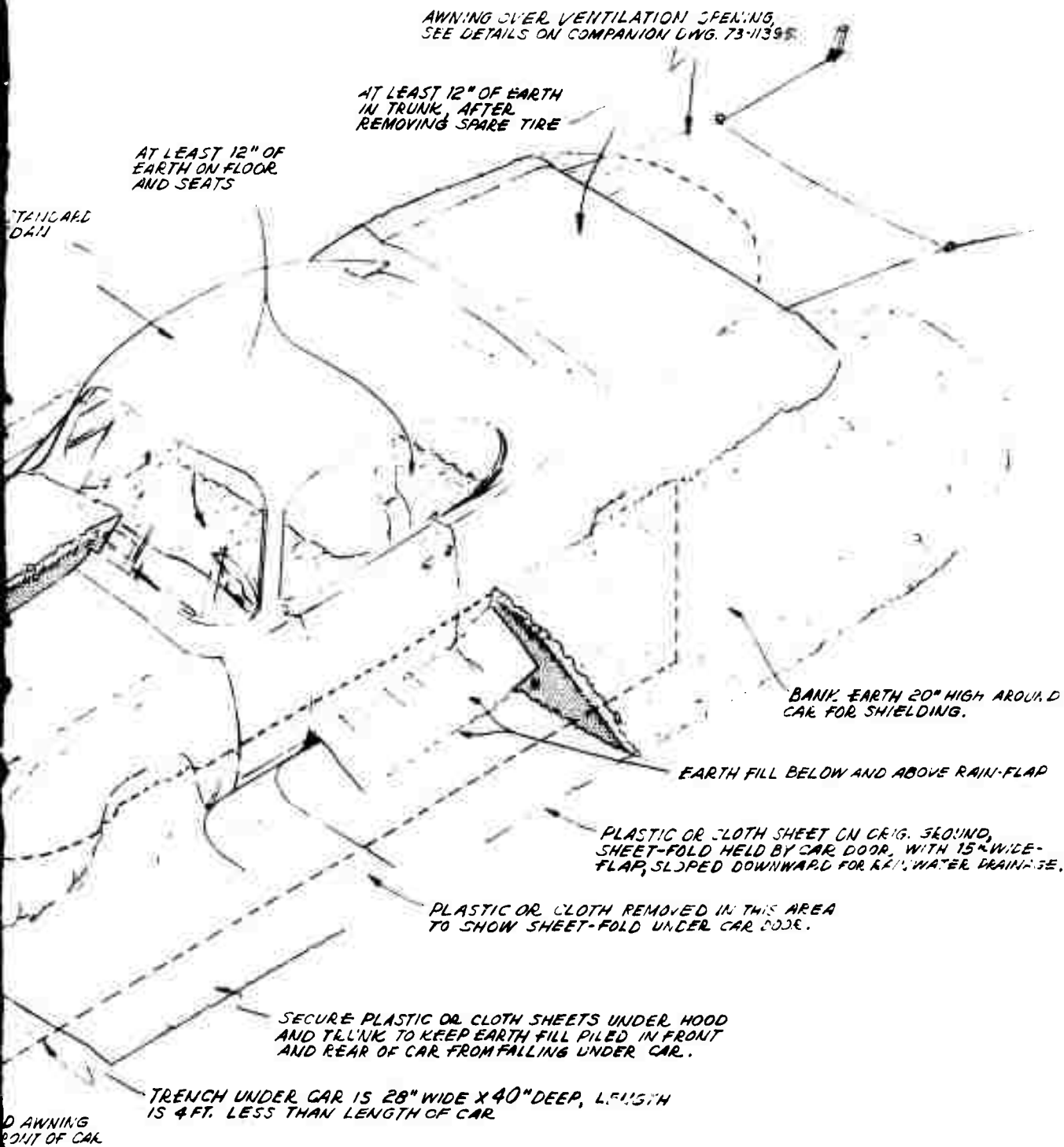
13.1. Car-Over-Trench Shelter, Pictorial View.
