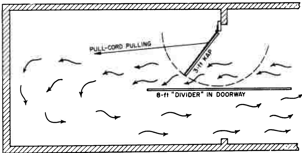
Fig. B-25. Use of "divider" to ventilate a shelter with only one opening.
