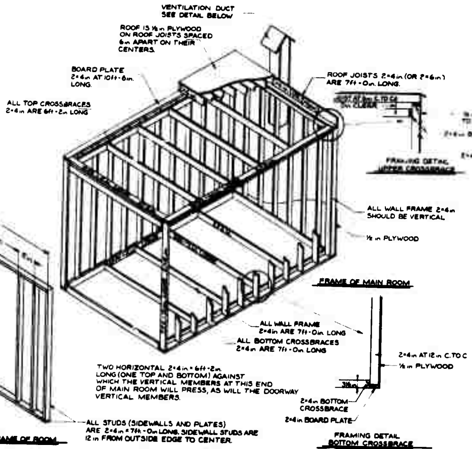
ALL SIDE WALLS NOT IN SUMP ARE 2x4in x 7ft-0in LONG
