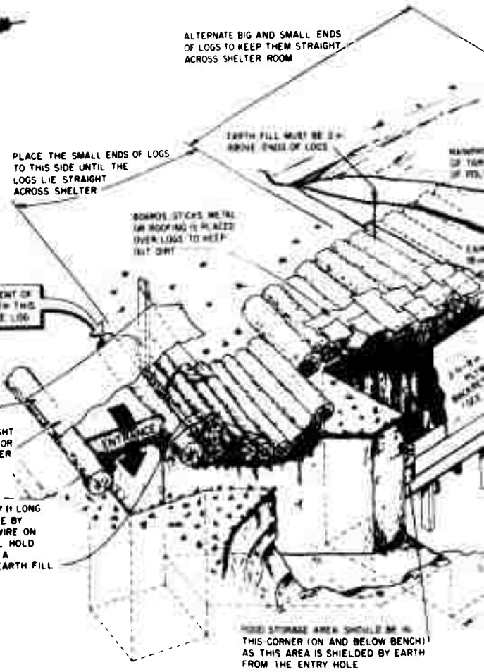
Fig. A-2.1. Log-Covered Trench Shelter, Pictorial View
