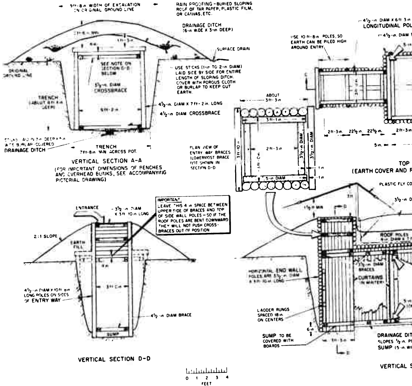
Fig. A-1.2. Small-Pole Shelter, Plan and
