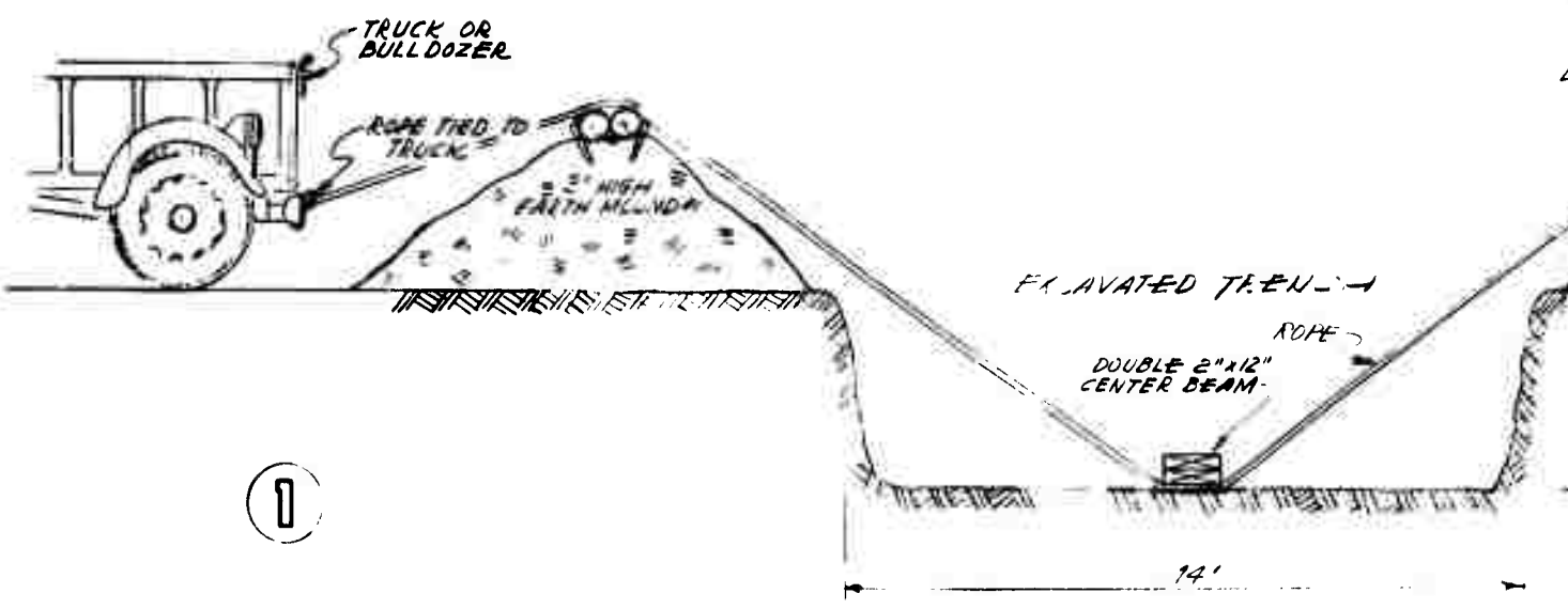
PICTORIAL VIEW SHOWING LIFTING MECHANISM FOR HEAVY CENTER BEAM
