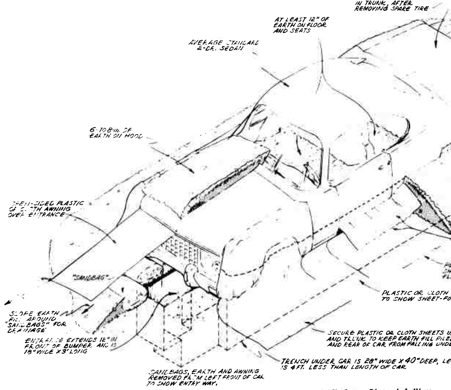
Fig. A-13.1. Car-Over-Trench Shelter, Pictorial View.
