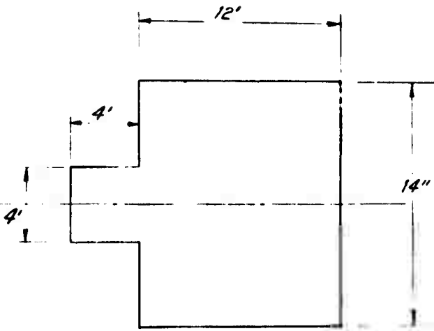
PLAN VIEW OF TRENCH - 4' DEEP
