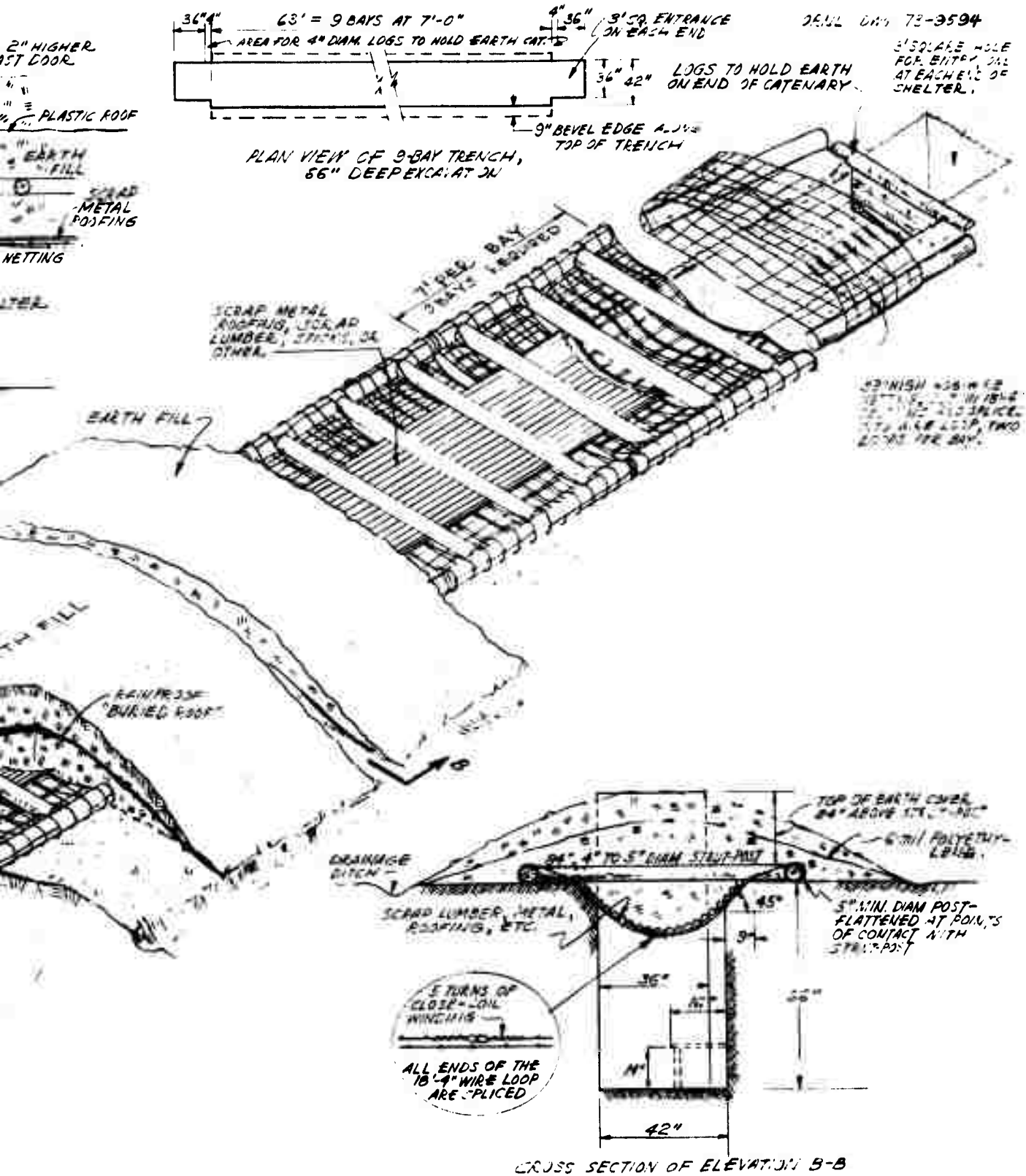
A-3.2. Catenary wire roofed shelter - alternate design.
