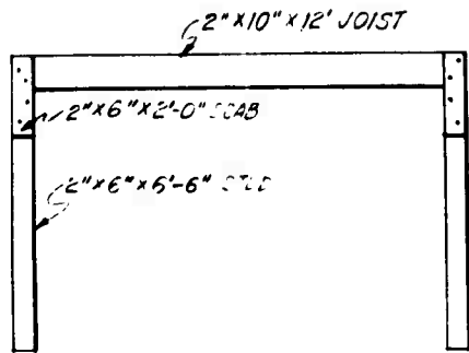
ELEV. VIEW - SUBASSEMBLY
