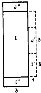
1.c TYPICAL LAYOUT FOR THREE SIDES OF ENTRY HATCH. TOTAL REQUIRED = 3 SHEETS USE PIECES I' AND J' IN POSITION I'' AND J'', FOURTH SIDE REQUIRES A PIECE 3 ft X 4 ft 2 in. WHICH MUST BE CUT FROM THE 17th PIECE OF PLYWOOD. SAVE THE SCRAP TO USE IN CONJUNCTION WITH THE K.A.P.
