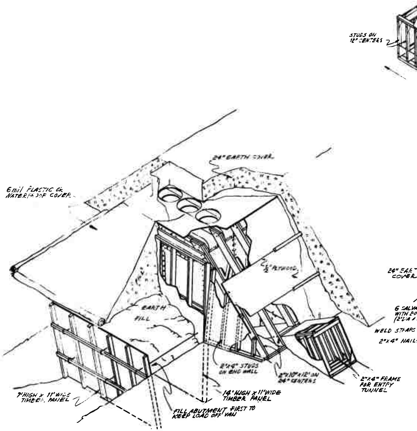
PICTORIAL VIEW OF FRAMING AT END OF VAN SHELTER
