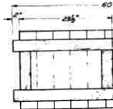
INSIDE FACE OF THE TOP SECTION, MARK ⑤
