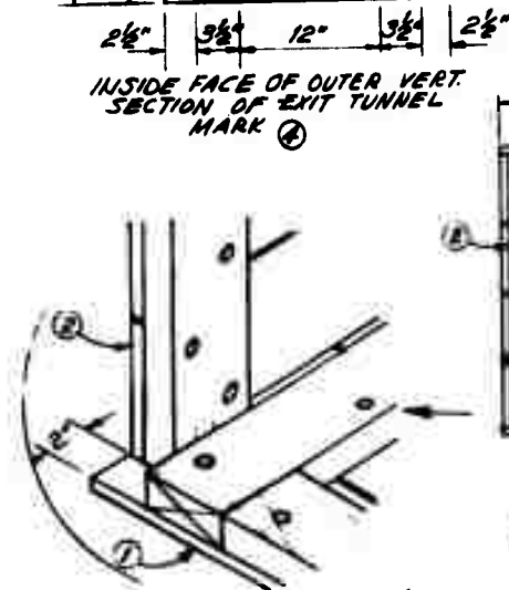
DETAIL A SHOWING 2" EXTENSION OF BOTTOM SECTION TO RECEIVE END VERT. SECTION MARKED ④
