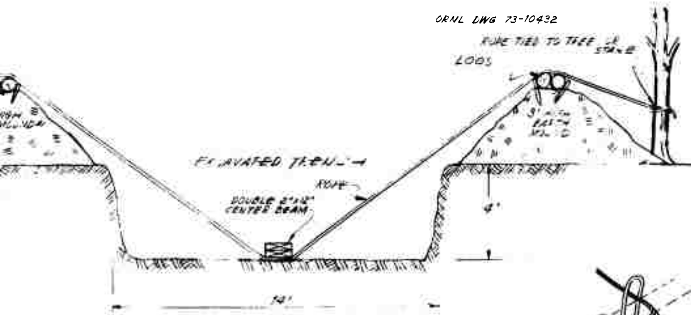
PICTORIAL VIEW SHOWING LIFTING MECHANISM FOR HEAVY CENTER BEAM
