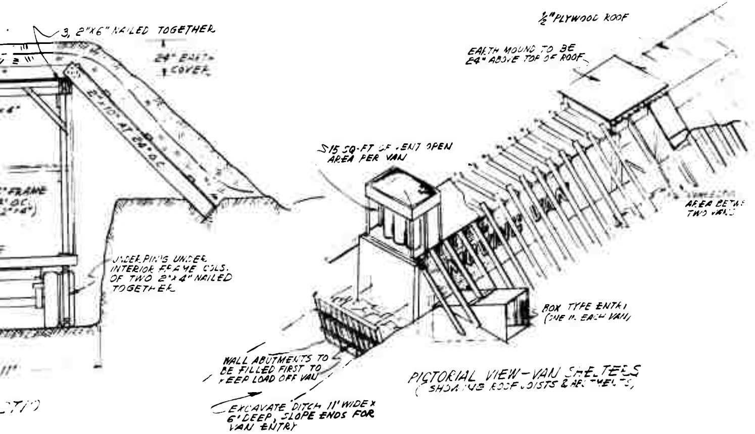
1. Trailer Van Shelter, Pictorial View and Sections.
