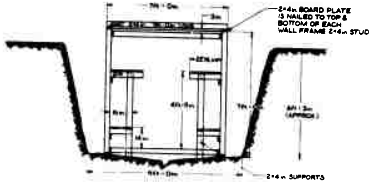
END VIEW OF MAIN ROOM SHOWING PLACEMENT OF BENCHES AND BOARD BUNKS - FROM REAR END OF MAIN ROOM THE 2x4 BUNK SUPPORTS ARE SPACED 3ft-0in APART.
