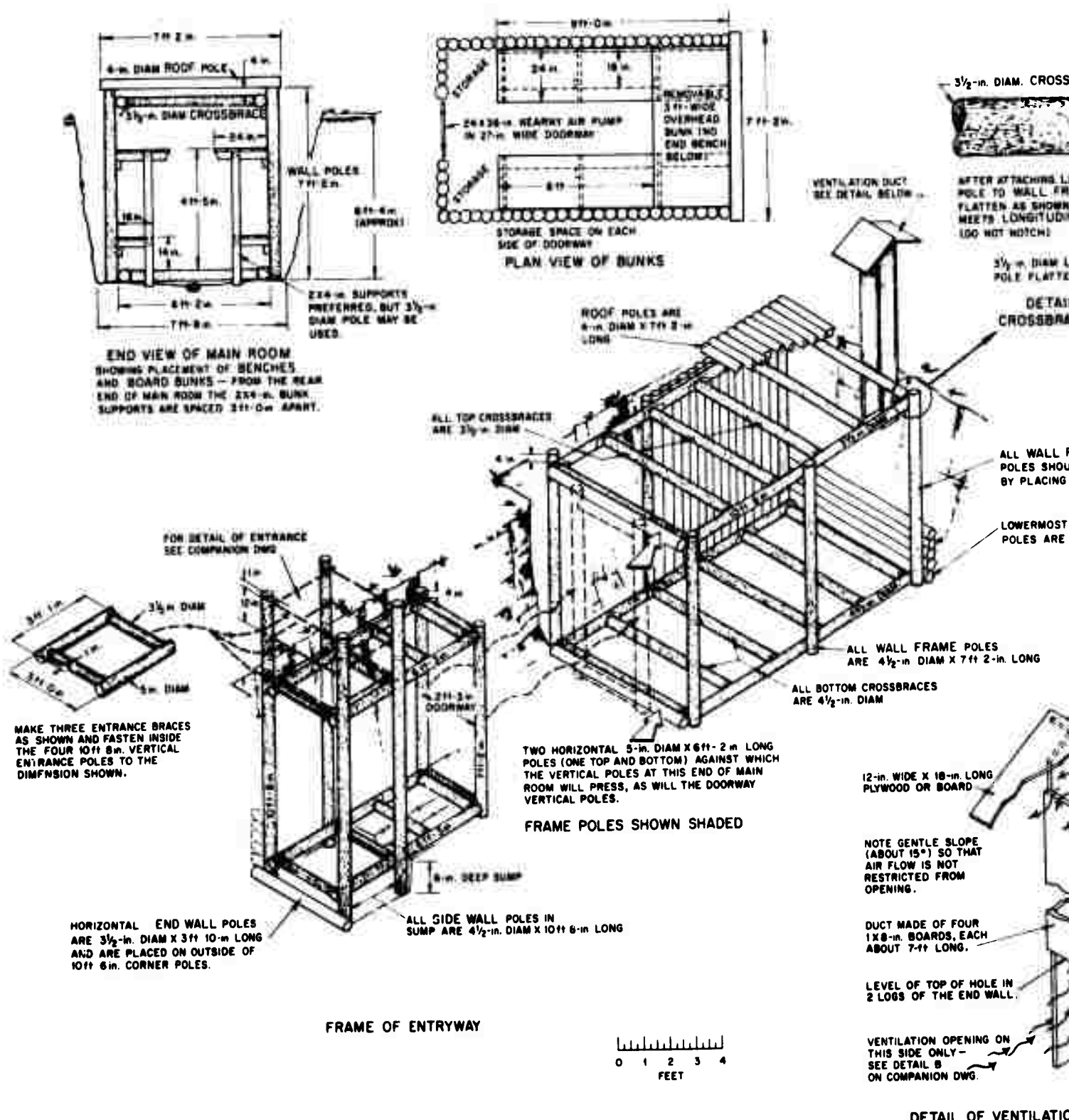
Fig. A-1.1. Small-Pole Shelter, Pictorial View.
