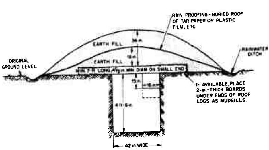
VIEW B-B', CROSS SECTION THROUGH WIDTH OF TRENCH SHELTER
