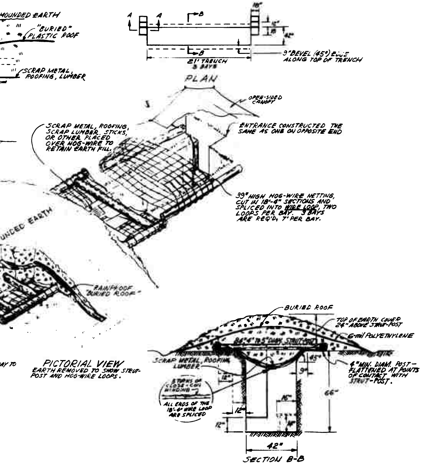
Fig. A-3.1. Catenary wire roofed shelter - basic design.
