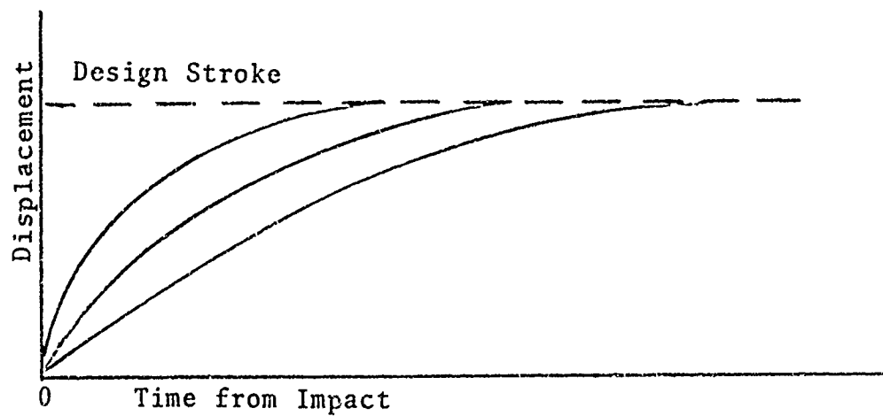
Figure 1. Motion-Time History for Different Deceleration Profiles Using a Fixed Stopping Distance
