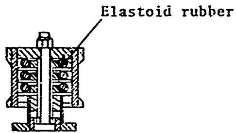
Rubber Snubber (Reference 9)
