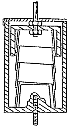
Reverse-Wound Coil Spring (Reference 6)
