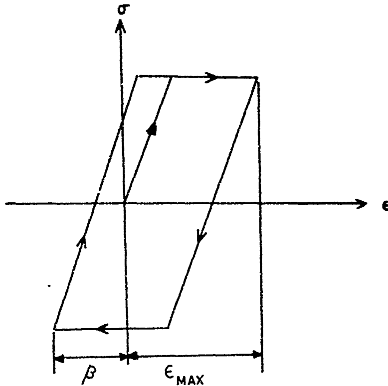
Figure I.1.3. Loading Path of Material
