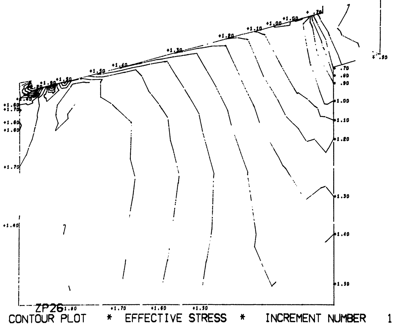
Figure B.10. Magnitude and distribution of stress in window-flange assembly Configuration B utilizing a titanium flange, fiber-reinforced-epoxy gasket, and glass ceramic window (problem 202). (sheet 8 of 8)
