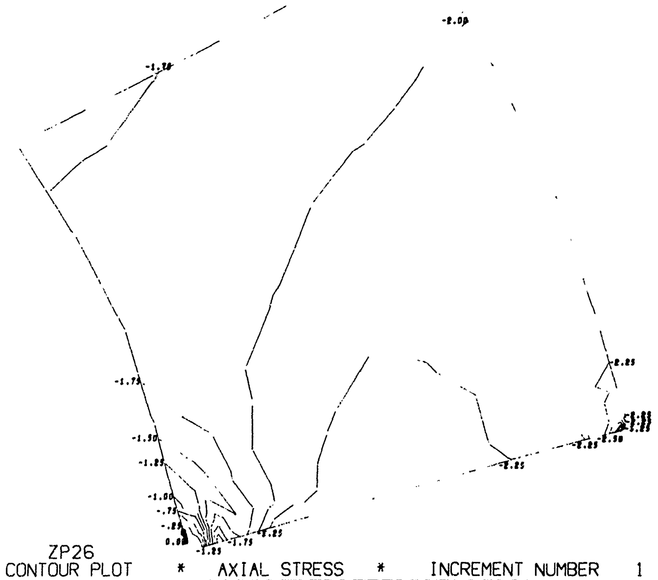
Figure B.6. Magnitude and distribution of stresses in window-flange assembly Configuration A utilizing a titanium flange, fiber-reinforced-epoxy laminate gasket and glass ceramic window (problem 106). (sheet 8 of 8)
