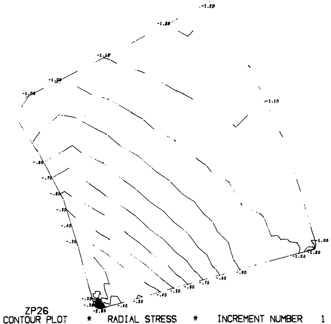
Figure B.10. Magnitude and distribution of stress in window-flange assembly Configuration B utilizing a titanium flange, fiber-reinforced-epoxy gasket, and glass ceramic window (problem 202). (sheet 3 of 8)
