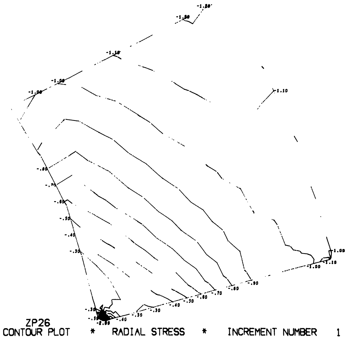
Figure B.9. Magnitude and distribution of stress in window-flange assembly Configuration B utilizing an aluminum flange, fiber-reinforced-epoxy gasket, and glass ceramic window (problem 203). (sheet 3 of 8)
