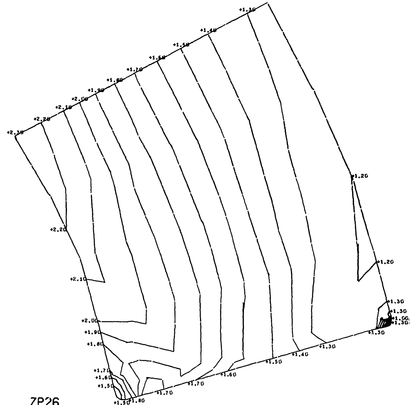
Figure E.8. Calculated effective stresses in Cer-Vit C-101 window and Monel K-500 flange. (sheet 2 of 2)
