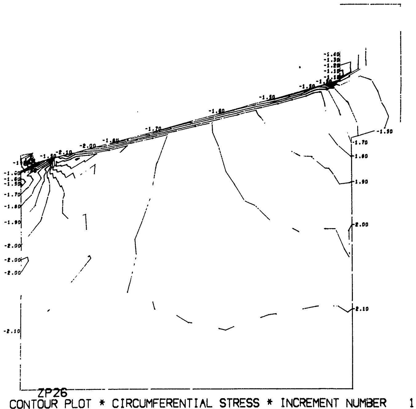
Figure B.10. Magnitude and distribution of stress in window-flange assembly Configuration B utilizing a titanium flange, fiber-reinforced-epoxy gasket, and glass ceramic window (problem 202). (sheet 6 of 8)
