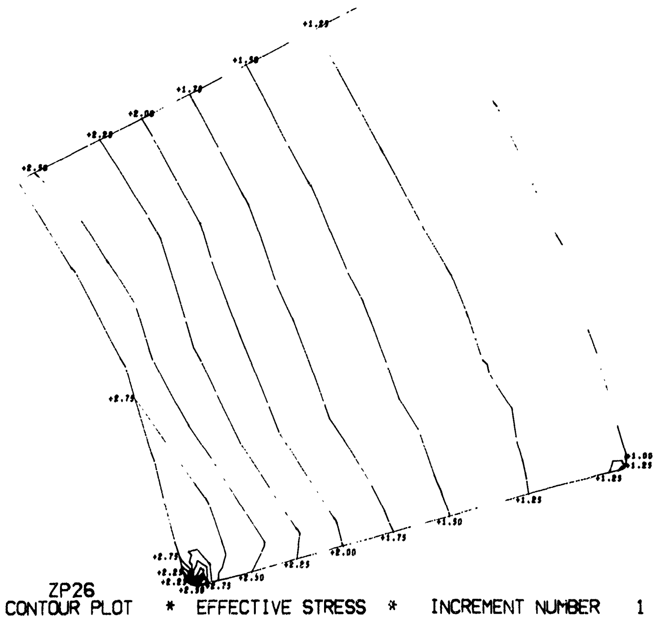
Figure B.9. Magnitude and distribution of stress in window-flange assembly Configuration B utilizing an aluminum flange, fiber-reinforced-epoxy gasket, and glass ceramic window (problem 203). (sheet 7 of 8)
