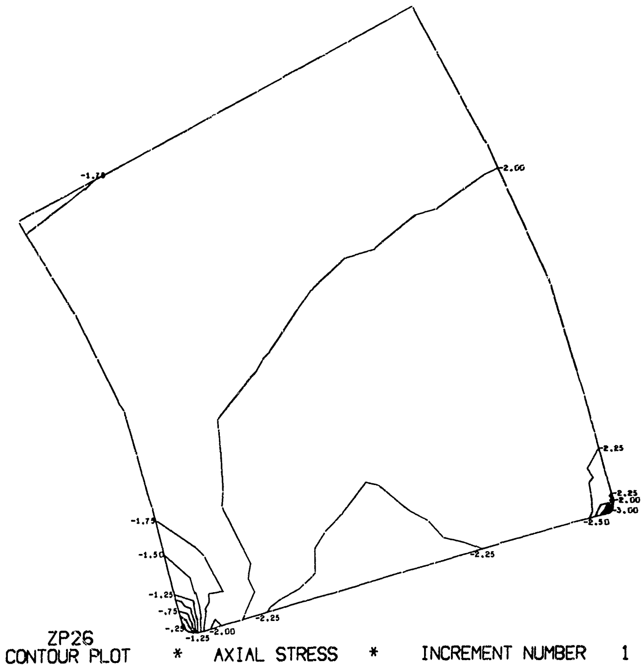
Figure 2. Finite element stress analysis of the NUC window-flange assembly subjected to external hydrostatic pressure; a glass window was supported by a Monel K-509 flange on an epoxy-coated PRD-49 cloth gasket. (sheet 8 of 10)
