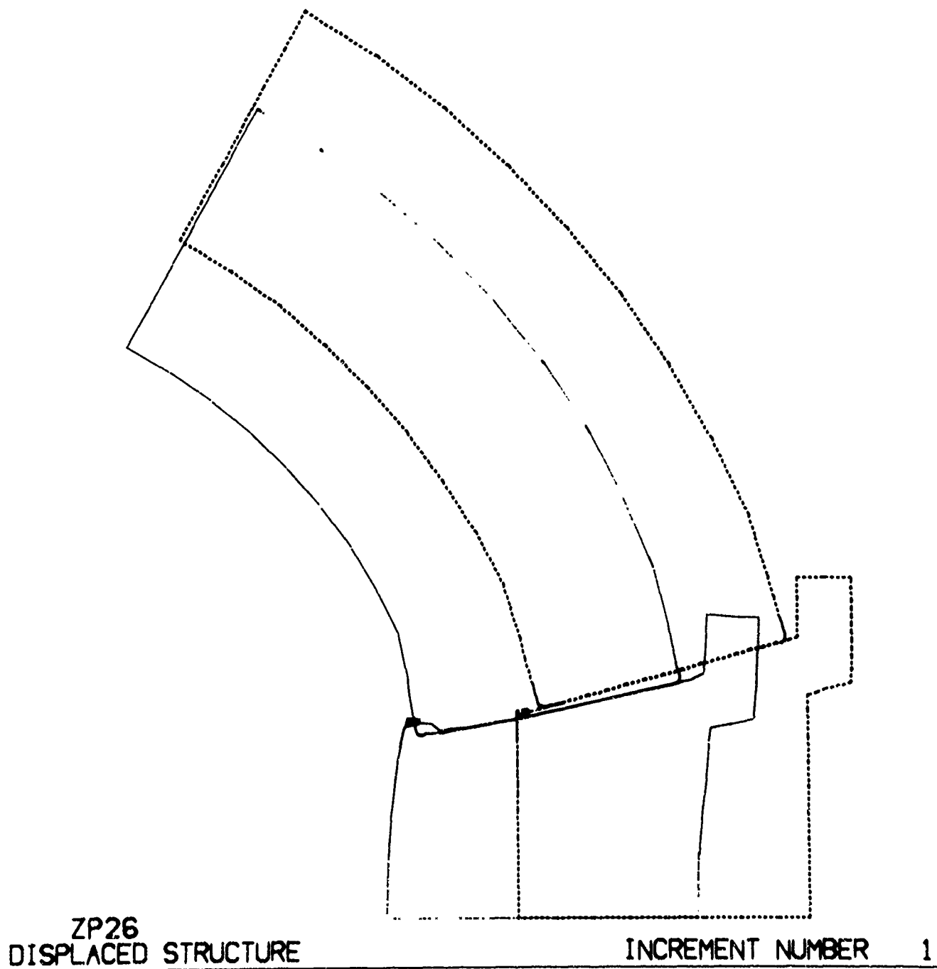
Figure B.11. Radial displacements of window and flange in Configuration B under external hydrostatic loading: problem 203, ceramic on aluminum.
