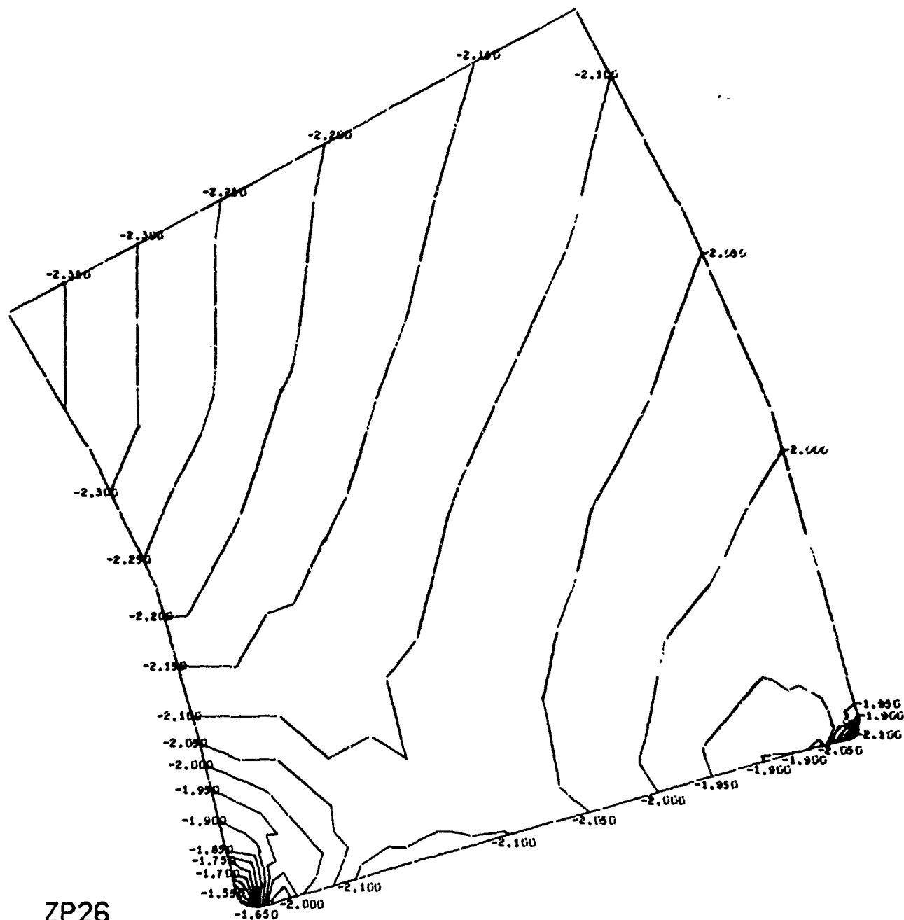
Figure E.5. Calculated circumferential stresses in Cer-Vit C-101 window and Monel K-500 flange. (sheet 2 of 2)
