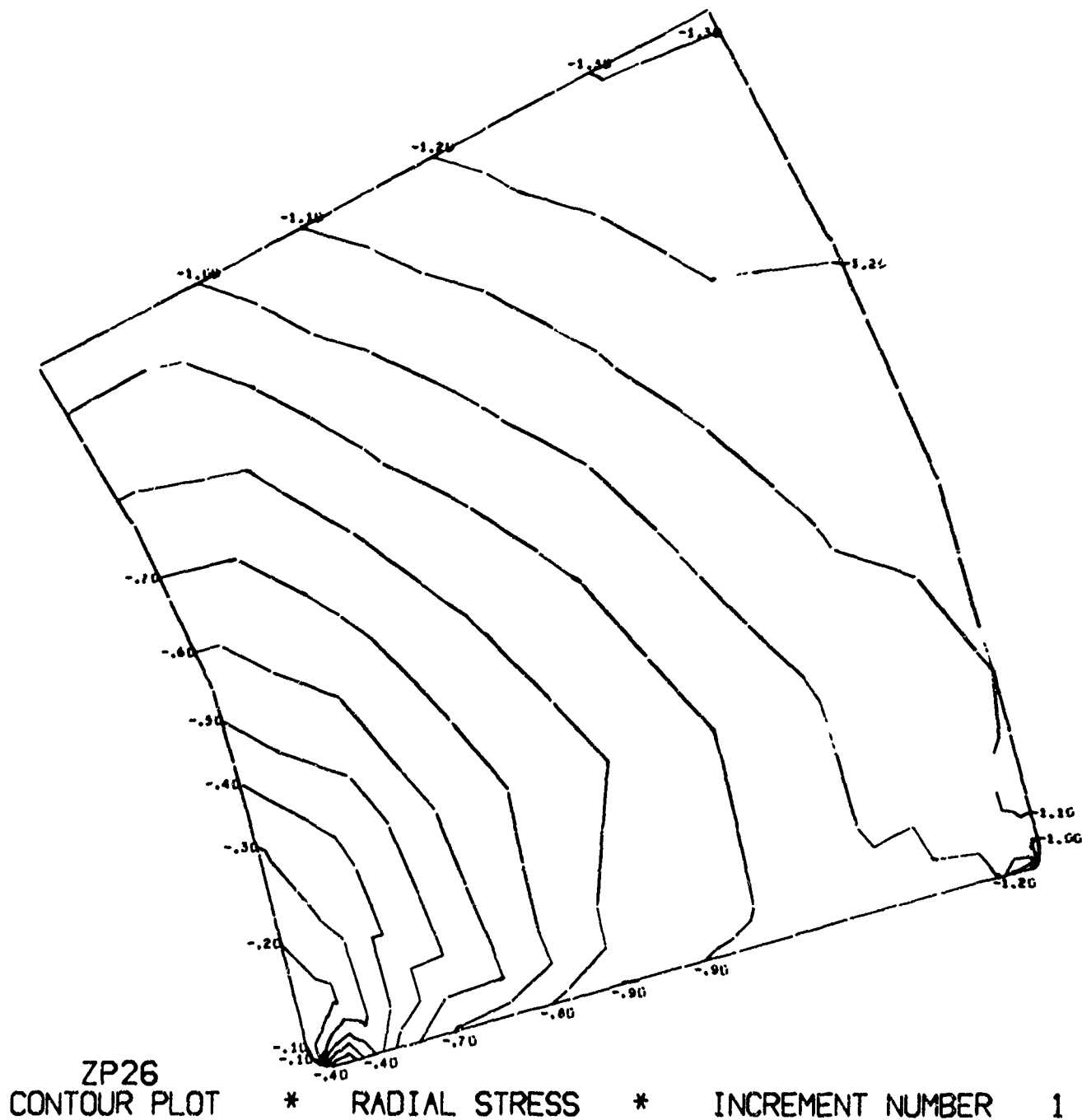
Figure E.7. Calculated radial stresses in Cer-Vit C-101 window and Monel K-500 flange. (sheet 2 of 2)
