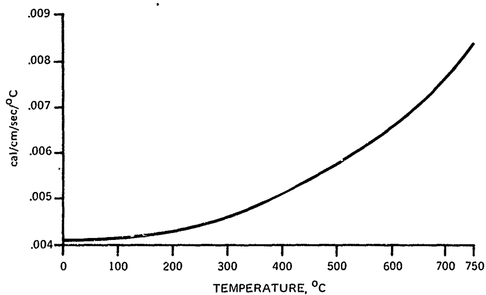
Figure C.12. Thermal conductivity for Cer-Vit C-101.
