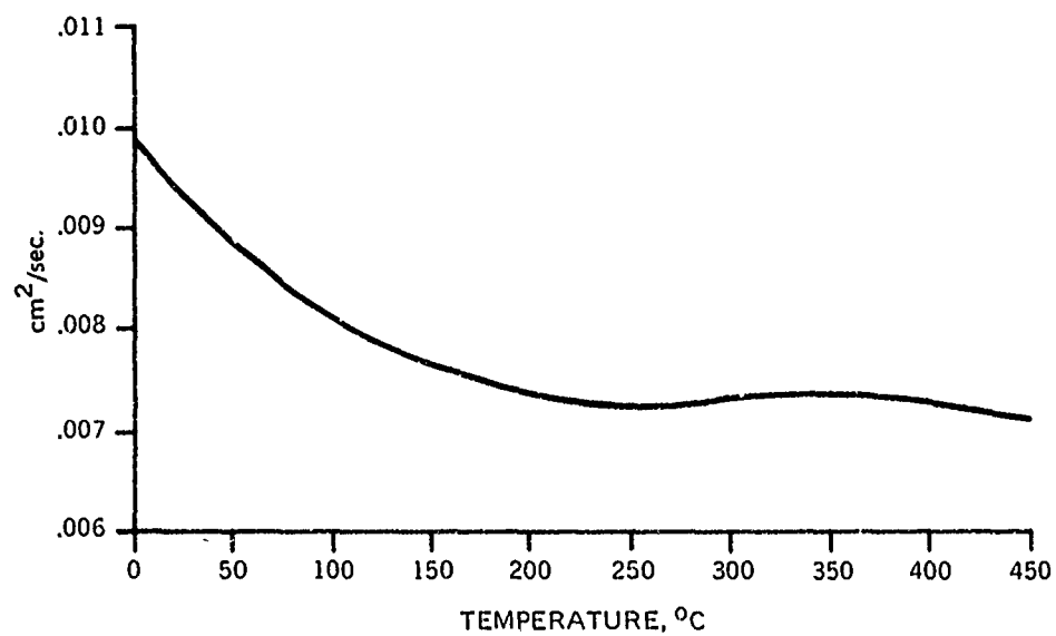
Figure C.11. Thermal diffusivity for Cer-Vit C-101.
