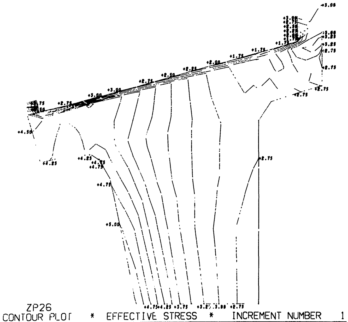
Figure B.5. Magnitude and distribution of stresses in window-flange assembly Configuration A utilizing a steel flange, fiber-reinforced-epoxy gasket, and glass ceramic window (problem 102). (sheet 1 of 7)
