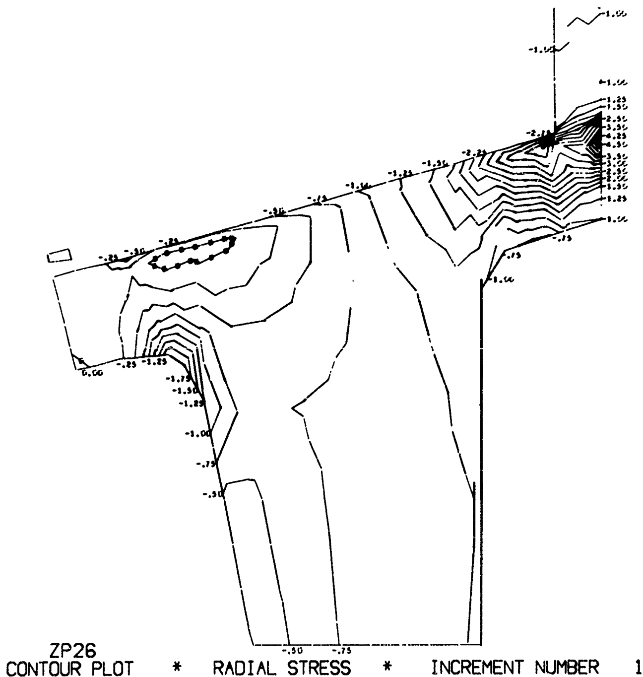
Figure E.7. Calculated radial stresses in Cer-Vit C-101 window and Monel K-500 flange. (sheet 1 of 2)
