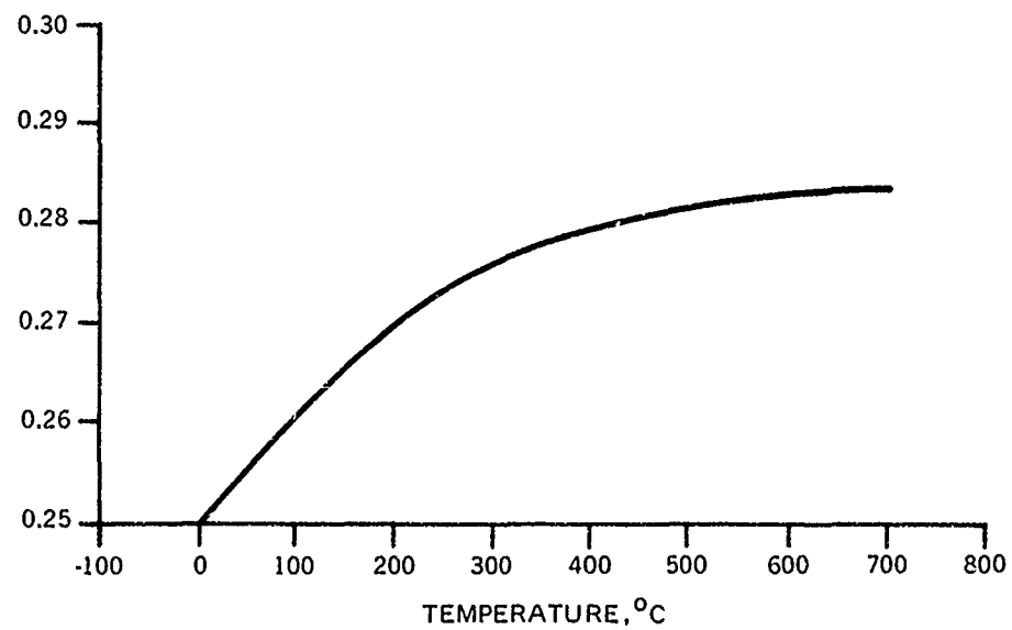
Figure C.9. Poisson's ratio for Cer-Vit C-101.
