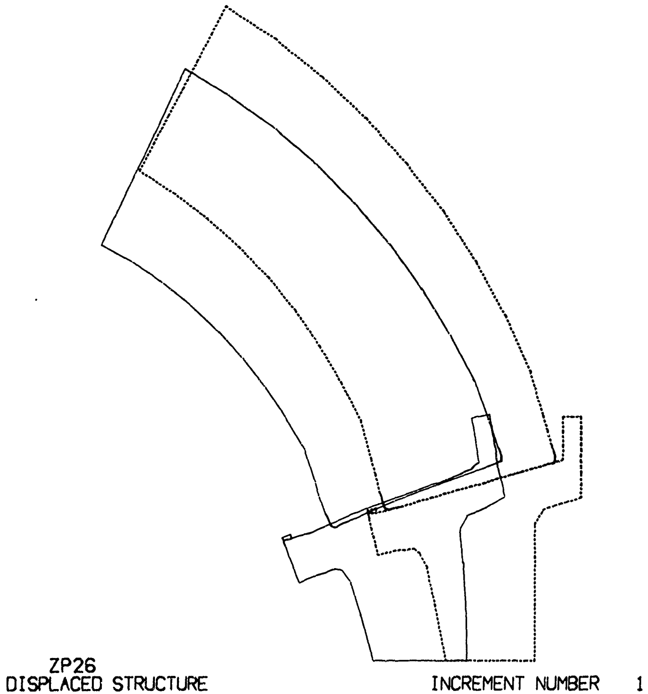
Figure E.9. Calculated displacements of Cer-Vit C-101 window and Monel K-500 flange.
