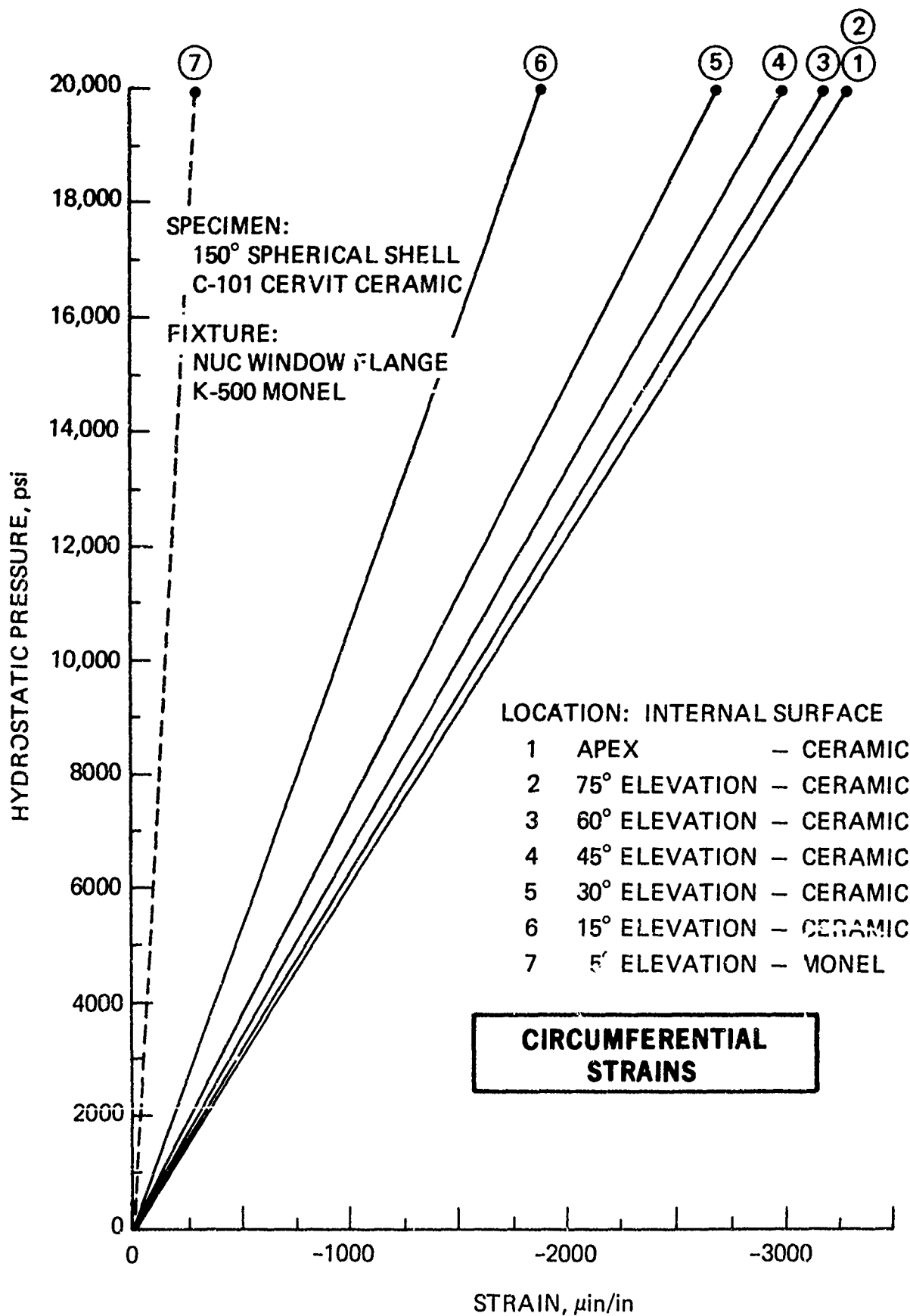
Figure E.1. Comparison of circumferential strains in Cer-Vit C-101 window and Monel K-500 flange.
