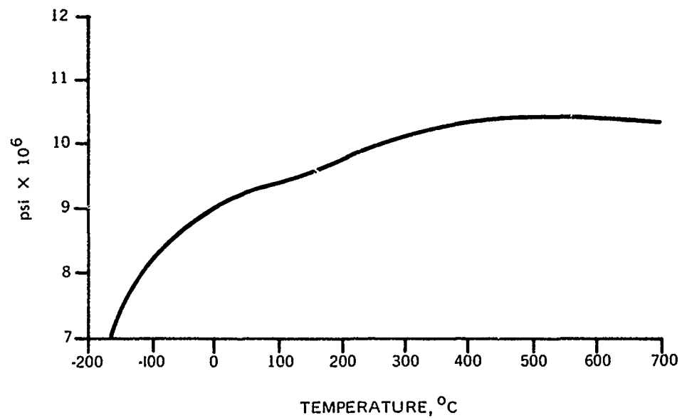
Figure C.8. Bulk modulus (B) for Cer-Vit C-101.
