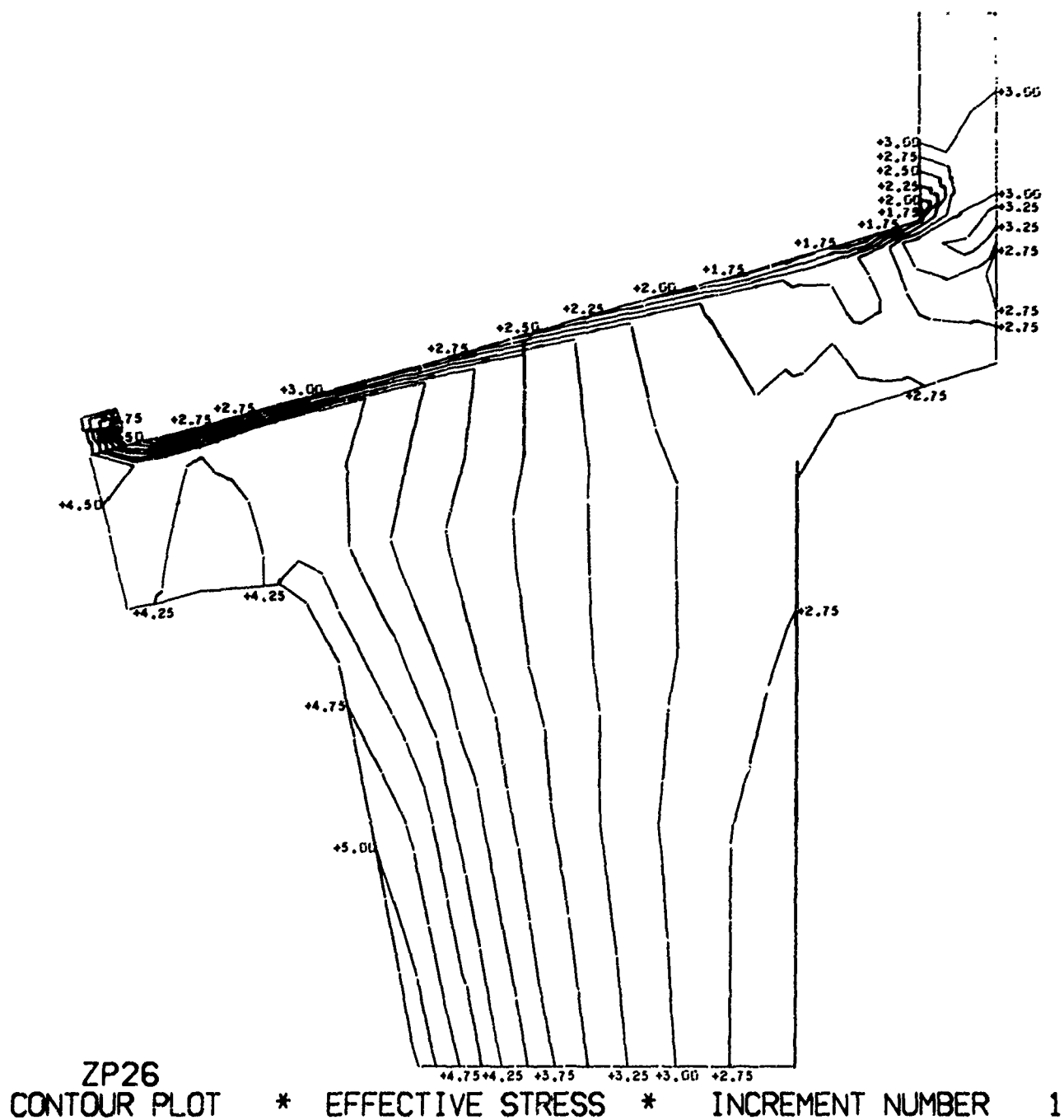
Figure E.8. Calculated effective stresses in Cer-Vit C-101 window and Monel K-500 flange. (sheet 1 of 2)
