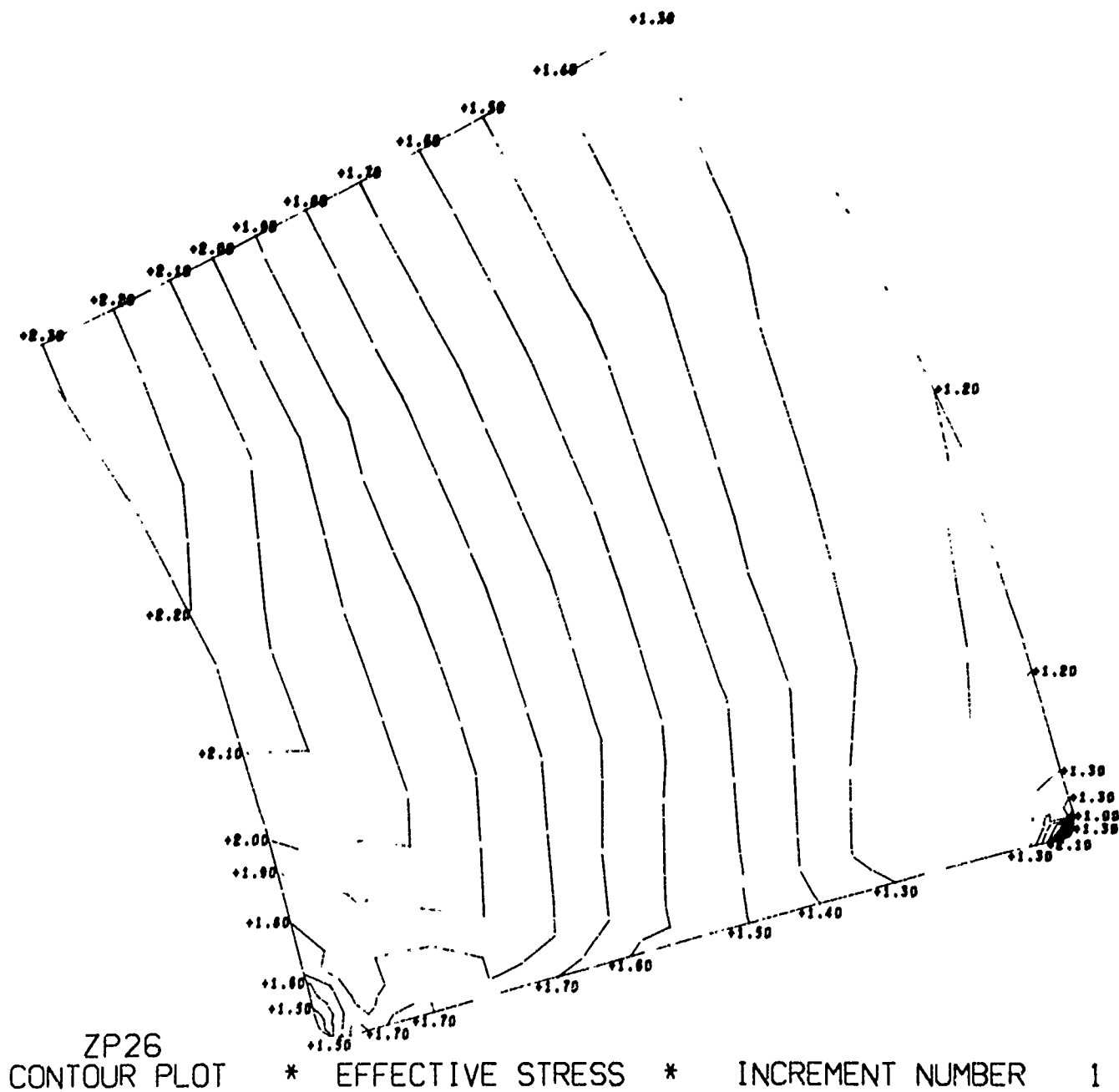
Figure B.5. Magnitude and distribution of stresses in window-flange assembly Configuration A utilizing a steel flange, fiber-reinforced-epoxy gasket, and glass ceramic window (problem 102). (sheet 2 of 7)
