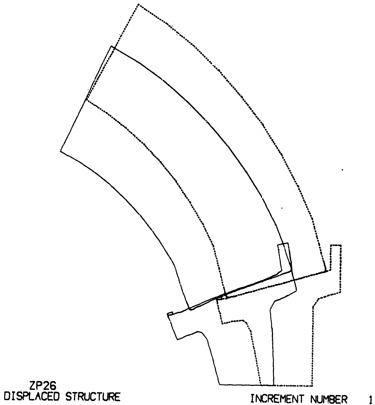
Figure 2. Finite element stress analysis of the NUC window-flange assembly subjected to external hydrostatic pressure; a glass window was supported by a Monel K-500 flange on an epoxy-coated PRD-49 cloth gasket. (sheet 2 of 10)
