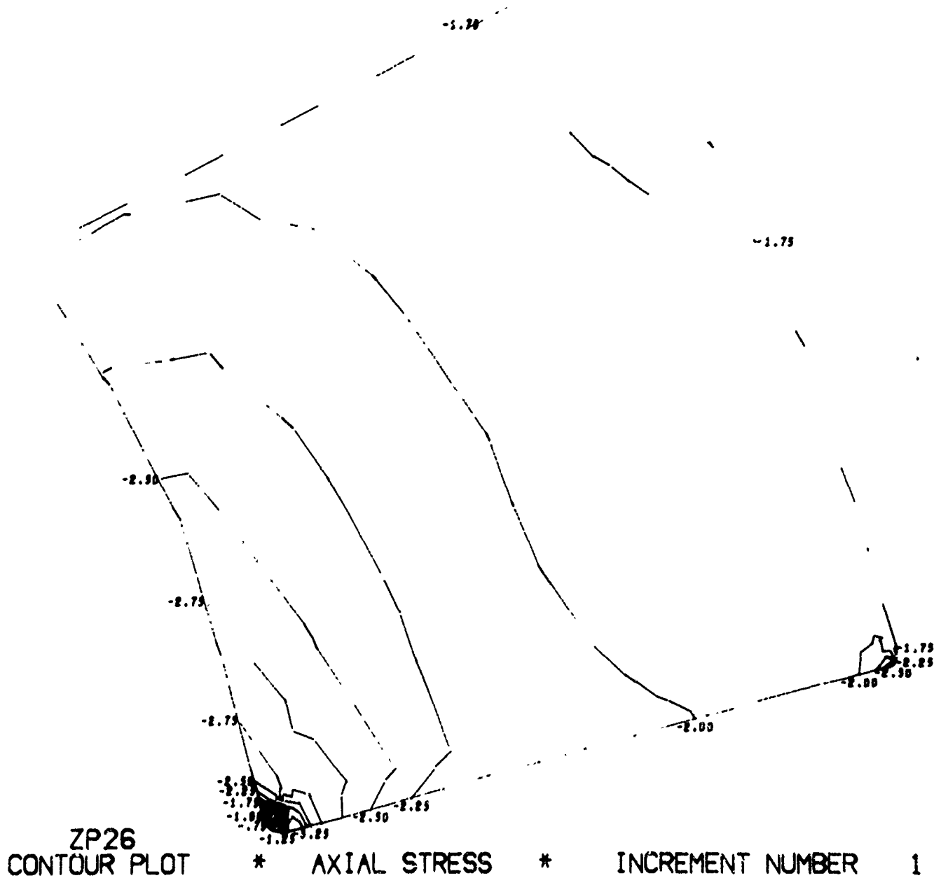
Figure B.9. Magnitude and distribution of stress in window-flange assembly Configuration B utilizing an aluminum flange, fiber-reinforced-epoxy gasket, and glass ceramic window (problem 203). (sheet 1 of 8)
