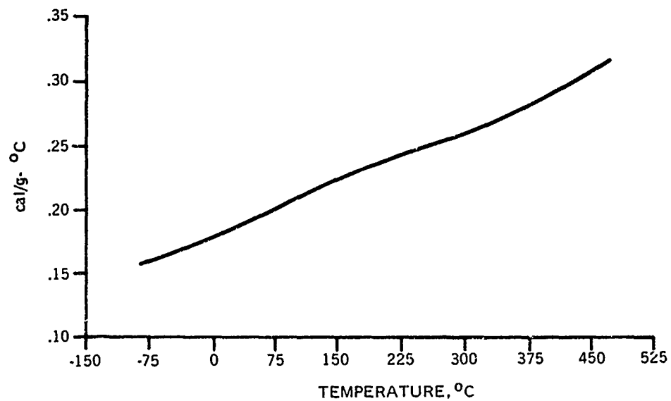
Figure C.10. Specific heat (C) for Cer-Vit C-101.
