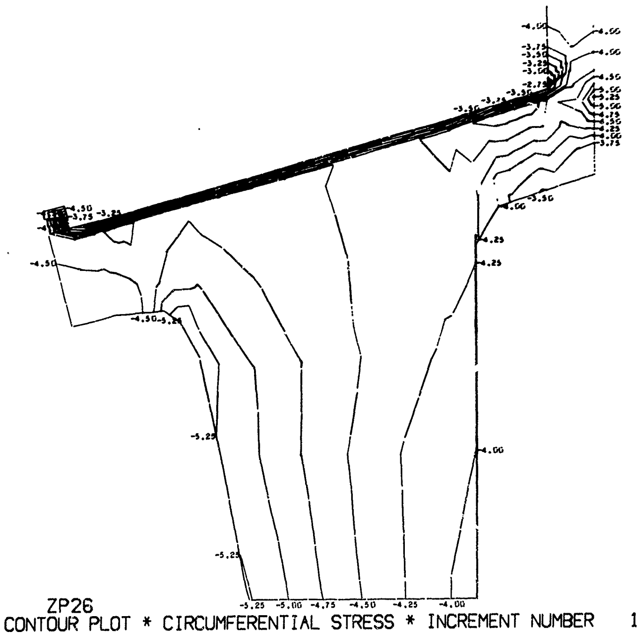
Figure E.5. Calculated circumferential stresses in Cer-Vit C-101 window and Monel K-500 flange. (sheet 1 of 2)
