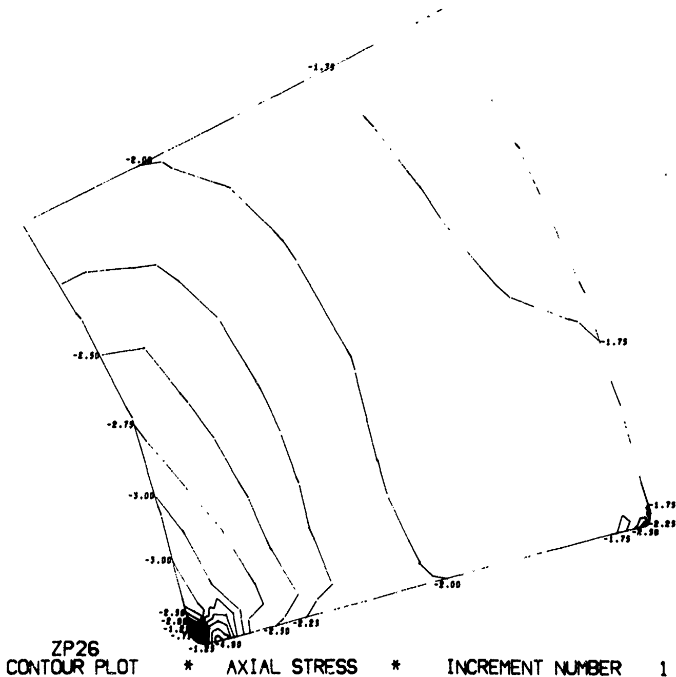
Figure B.8. Magnitude and distribution of stresses in window-flange assembly Configuration B, utilizing a glass-reinforced-plastic flange and glass ceramic window (problem 204). (sheet 8 of 8)
