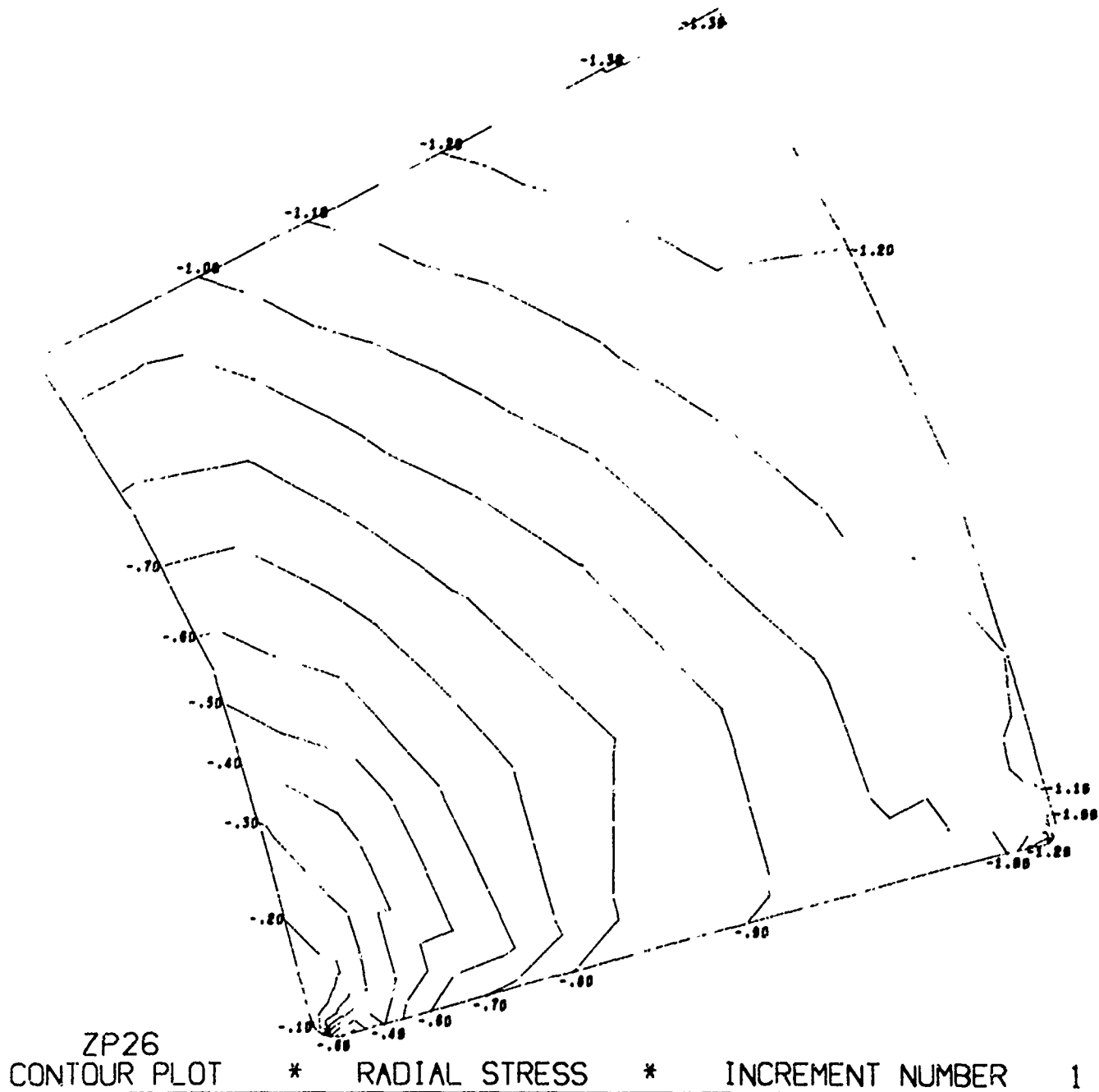
Figure B.5. Magnitude and distribution of stresses in window-flange assembly Configuration A utilizing a steel flange, fiber-reinforced-epoxy gasket, and glass ceramic window (problem 102). (sheet 6 of 7)
