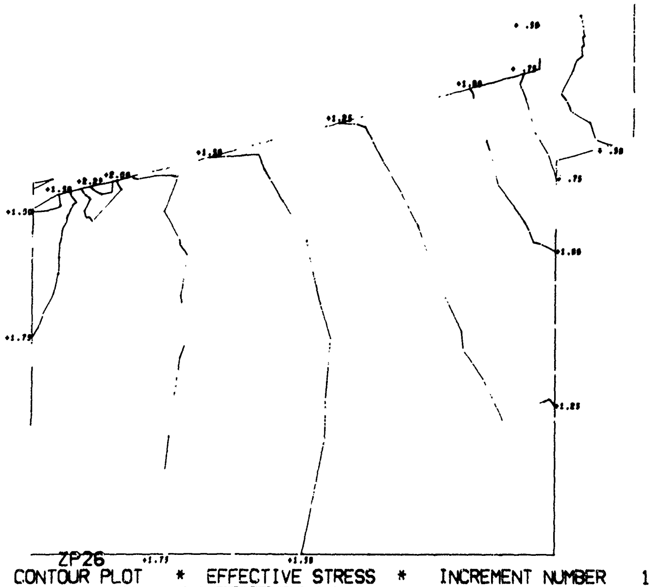
Figure B.8. Magnitude and distribution of stresses in window-flange assembly Configuration B, utilizing a glass-reinforced-plastic flange and glass ceramic window (problem 204). (sheet 1 of 8)
