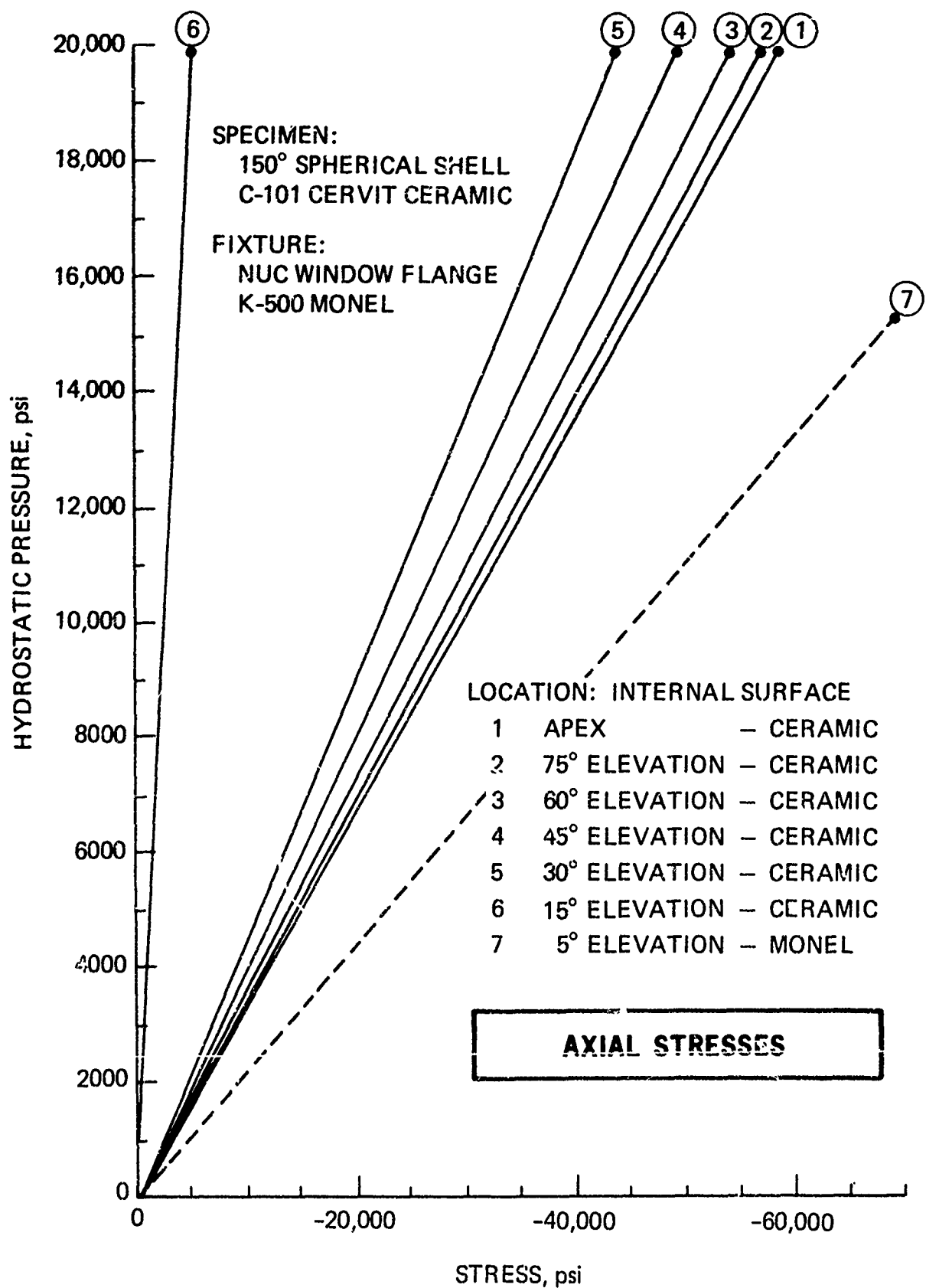
Figure E.4. Experimentally generated axial stresses in Cer-Vit C-101 window and Monel K-500 flange.
