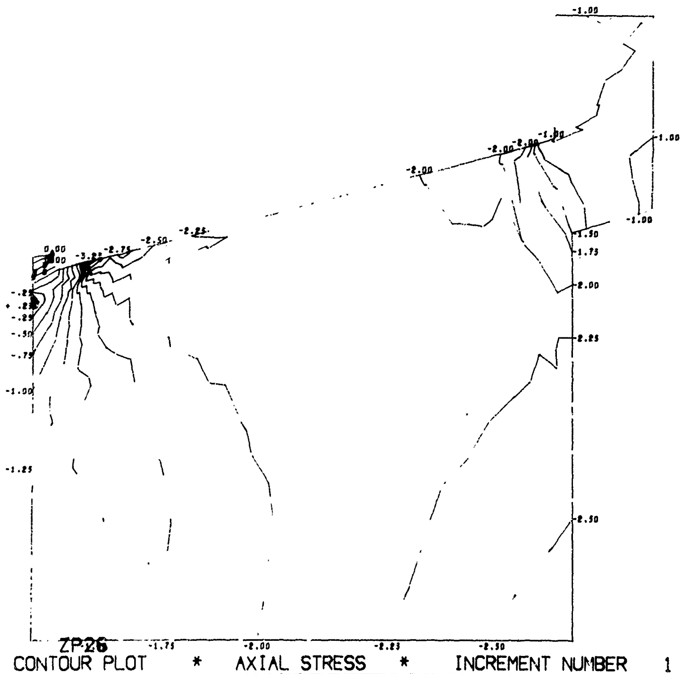
Figure B.10. Magnitude and distribution of stress in window-flange assembly Configuration B utilizing a titanium flange, fiber-reinforced-epoxy gasket, and glass ceramic window (problem 202). (sheet 2 of 8)
