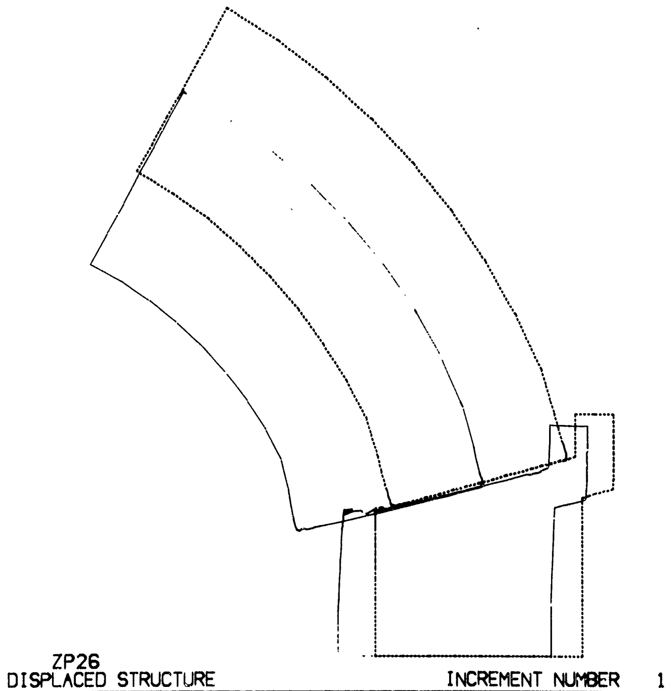
Figure B.11. Radial displacements of window and flange in Configuration B under external hydrostatic loading: problem 201, ceramic on steel.
