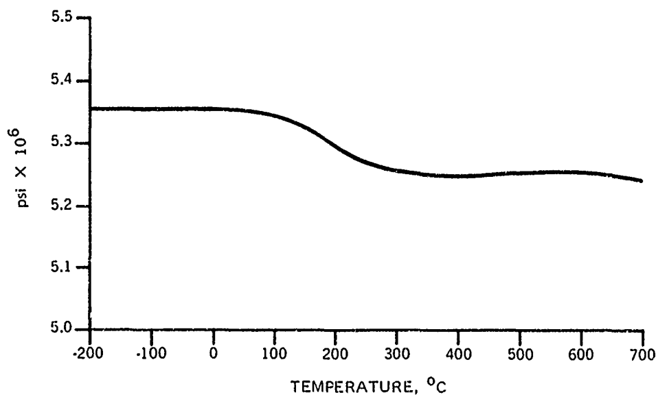
Figure C.7. Shear modulus for Cer-Vit C-101.
