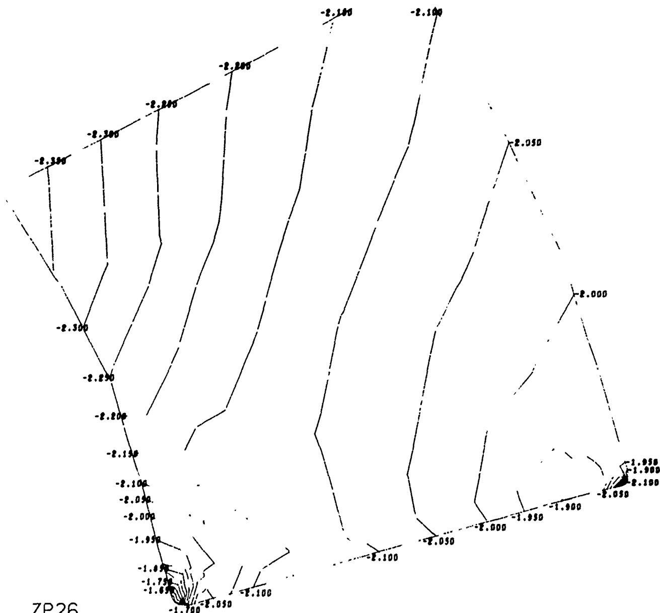
Figure B.5. Magnitude and distribution of stresses in window-flange assembly Configuration A utilizing a steel flange, fiber-reinforced-epoxy gasket, and glass ceramic window (problem 102). (sheet 4 of 7)
