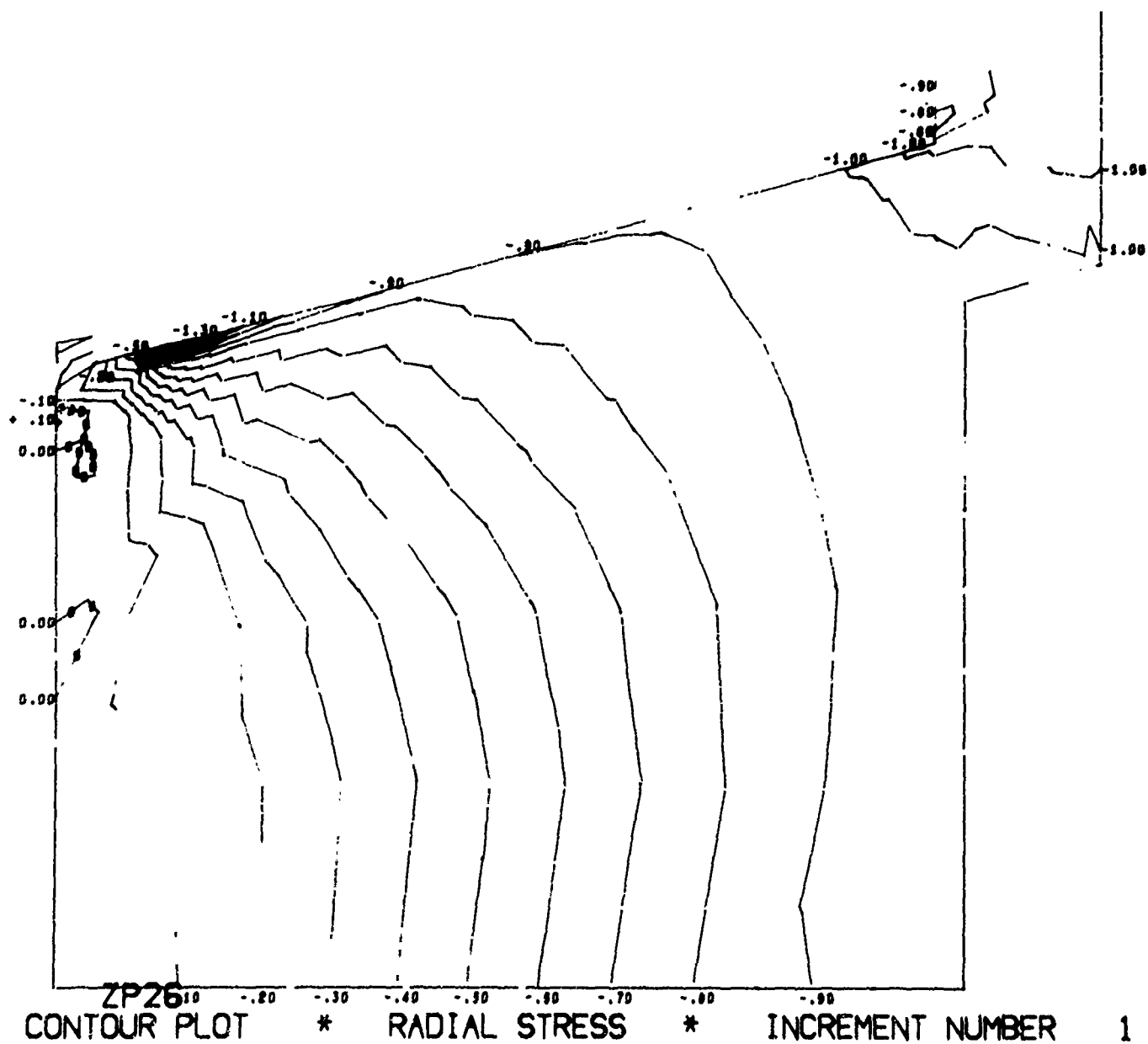
Figure B.9. Magnitude and distribution of stress in window-flange assembly Configuration B utilizing an aluminum flange, fiber-reinforced-epoxy gasket, and glass ceramic window (problem 203). (sheet 4 of 8)
