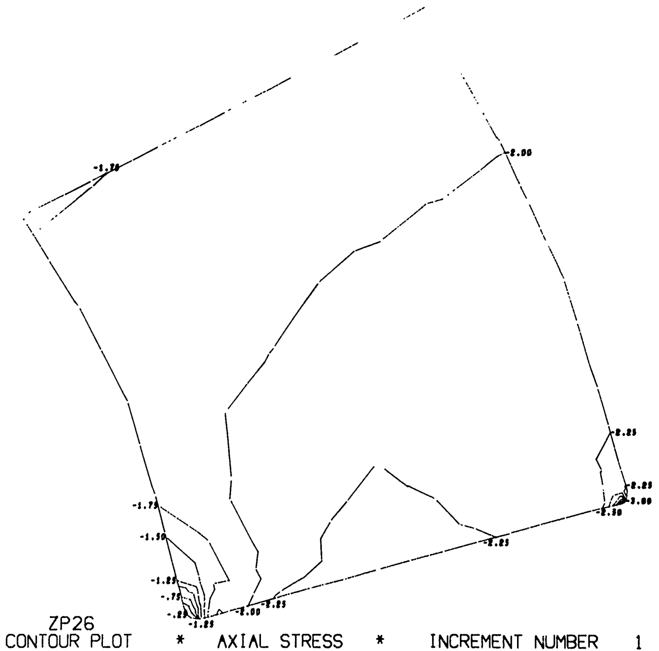
Figure E.6. Calculated axial stresses in Cer-Vit C-101 window and Monel K-500 flange. (sheet 2 of 2)
