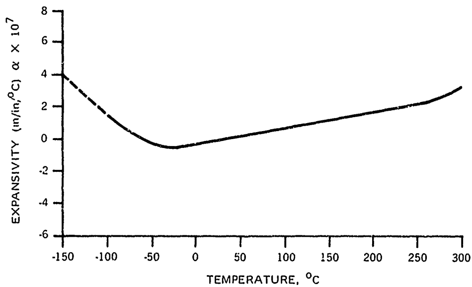
Figure C.13. Thermal expansion coefficient ( \alpha ) for Cer-Vit C-101.
