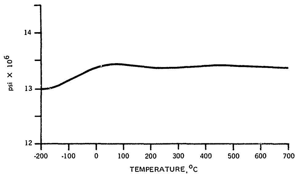
Figure C.6. Young's modulus for Cer-Vit C-101.
