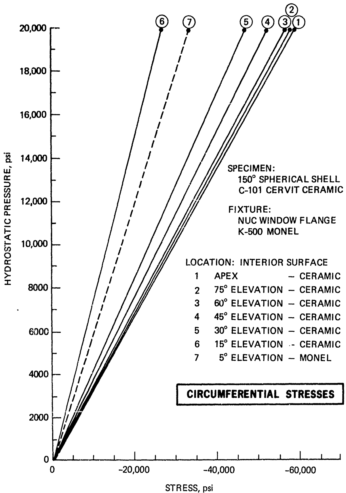
Figure E.3. Experimentally generated stresses in Cer-Vit C-101 window and Monel K-500 flange.
