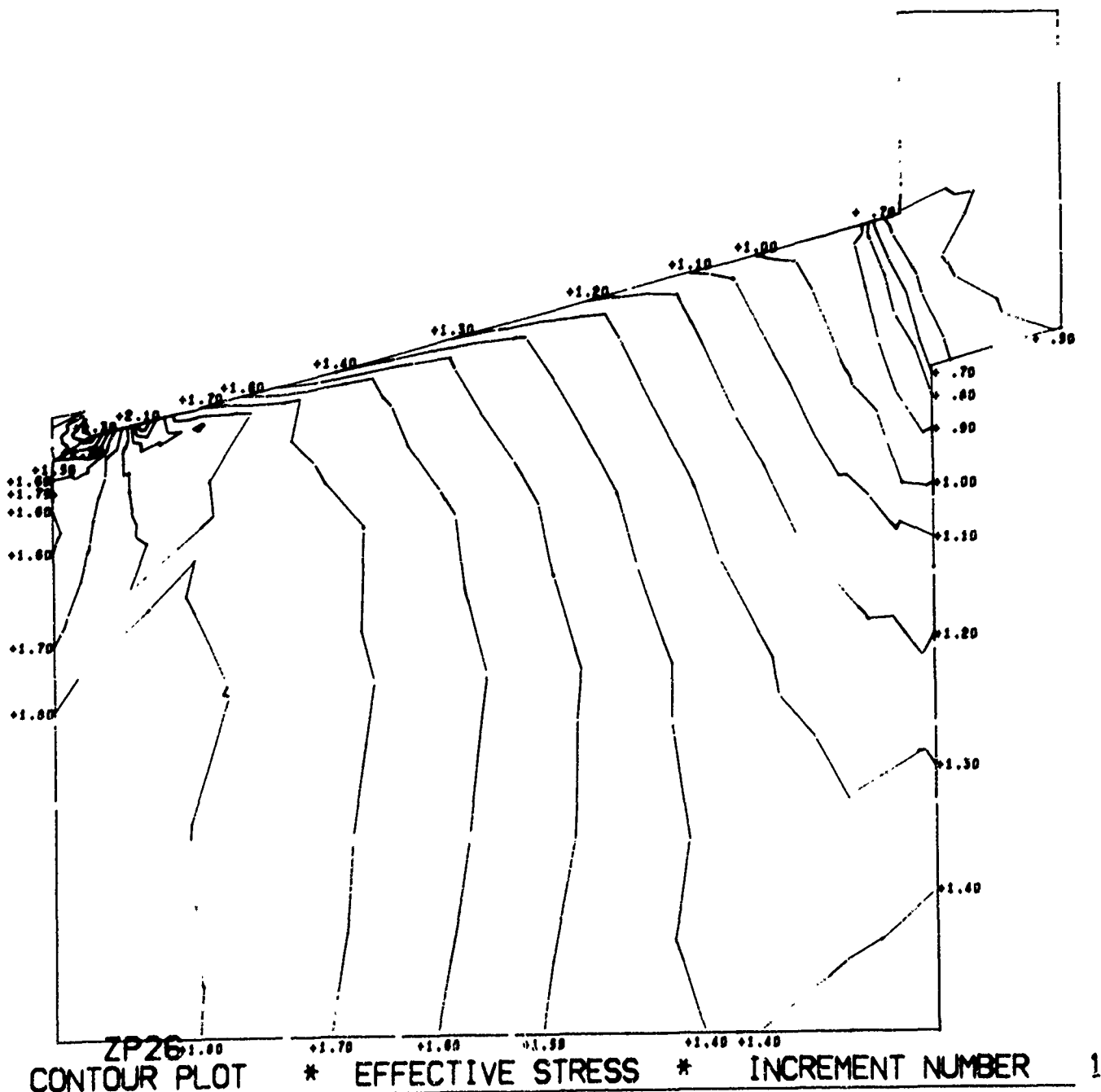
Figure B.9. Magnitude and distribution of stress in window-flange assembly Configuration B utilizing an aluminum flange, fiber-reinforced-epoxy gasket, and glass ceramic window (problem 203). (sheet 8 of 8)
