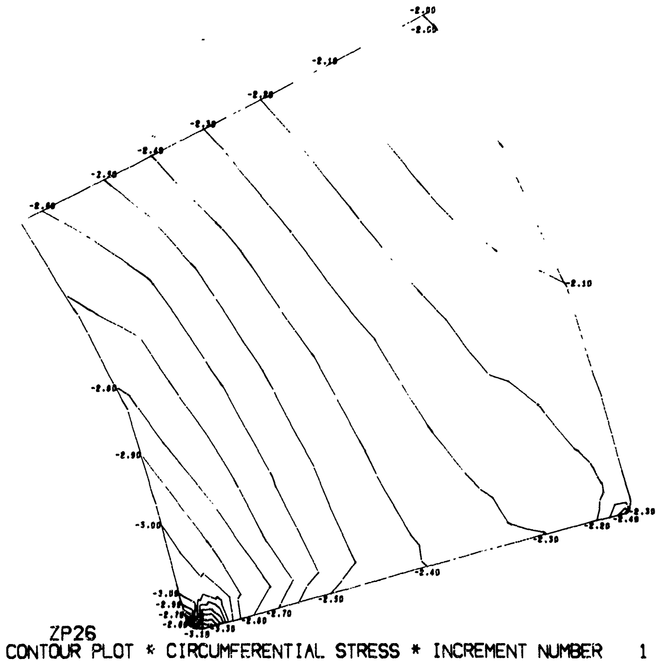
Figure B.8. Magnitude and distribution of stresses in window-flange assembly Configuration B, utilizing a glass-reinforced-plastic flange and glass ceramic window (problem 204). (sheet 4 of 8)
