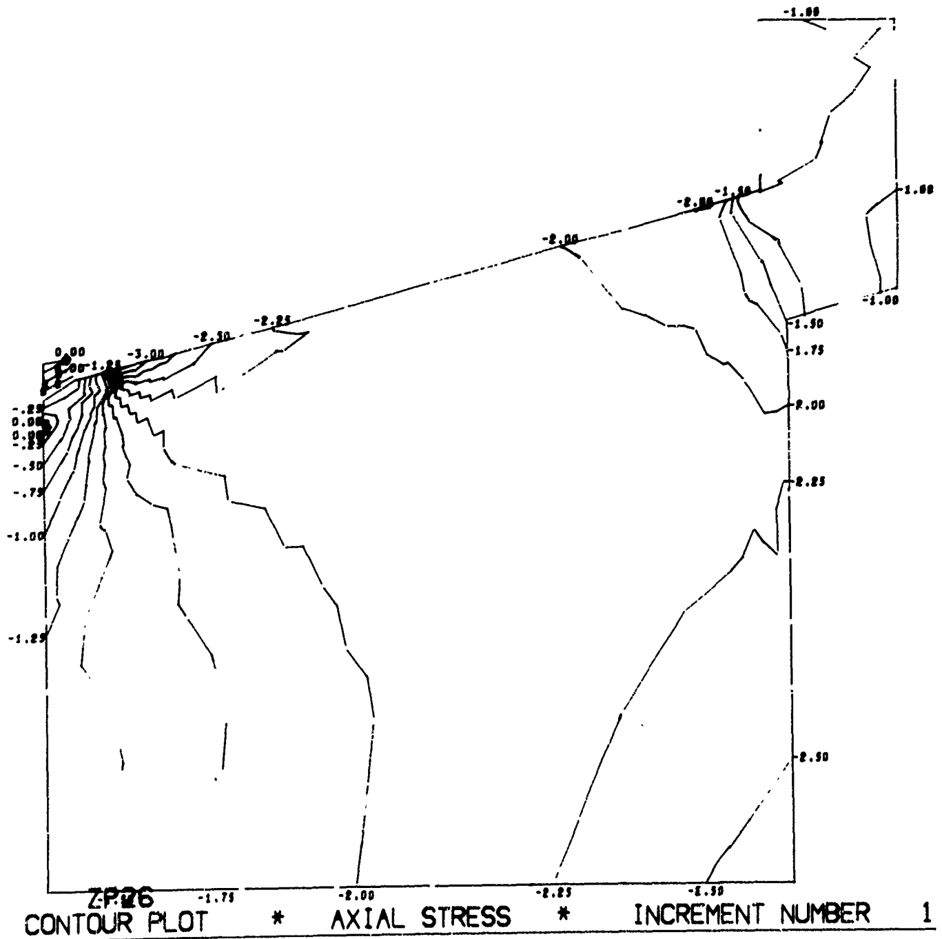
Figure B.9. Magnitude and distribution of stress in window-flange assembly Configuration B utilizing an aluminum flange, fiber-reinforced-epoxy gasket, and glass ceramic window (problem 203). (sheet 2 of 8)
