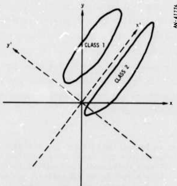
Figure 4.1. Illustration of Potential Rejection of Important Classification Information Following Principal Components Analysis
