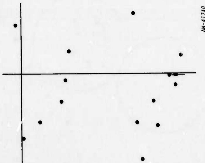
Figure 4.4. Samples Remaining After the Samples Initially Assigned to the First Mode are Removed (The arrow again indicates the point of maximum probability.)
