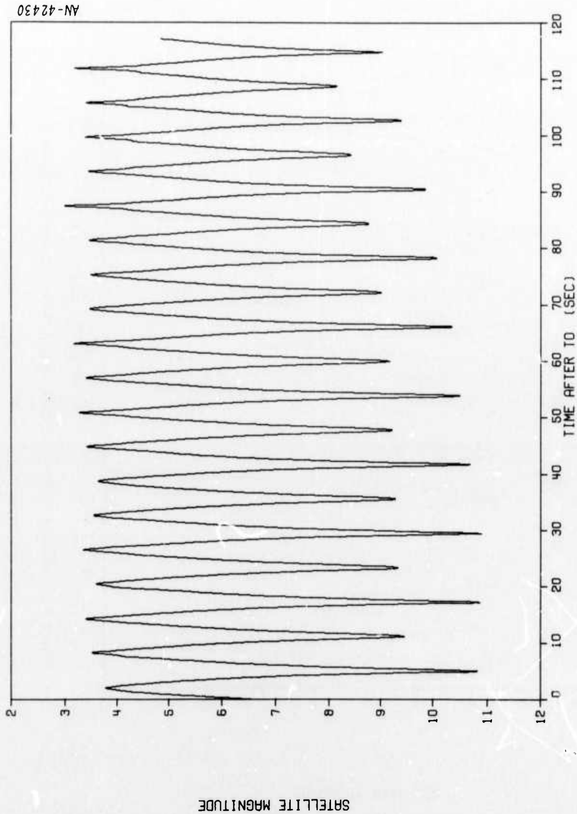
Figure 6.10. Simulated Passive Photometric Data for Tumbling Agena 3
