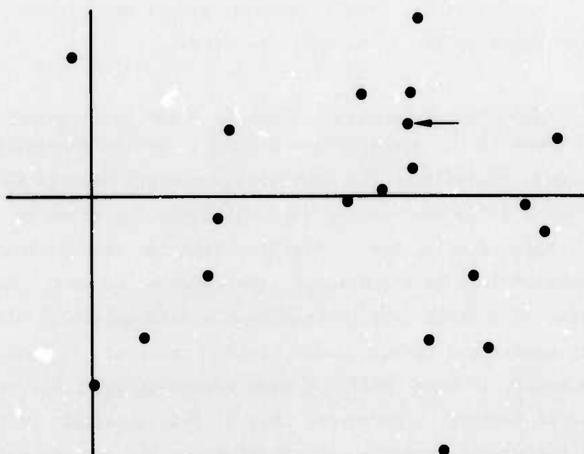
Figure 4.2. A Typical Set of Twenty Random Samples (arrow indicates point at which p(\vec{x}) is maximum on the first iteration) in a Two-Dimensional Sample Space
