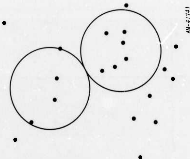
Figure 4.5. The Two Circles Found by Iteration Over the Samples
