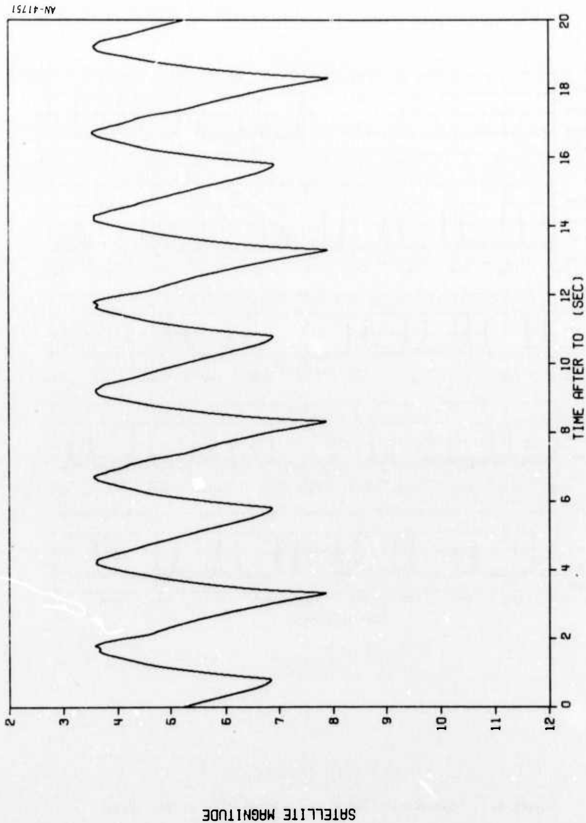
Figure 6.8. Simulated Passive Photometric Data for Tumbling Agena 1
