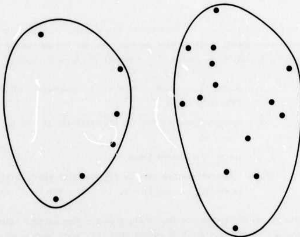
Figure 4.6. Clustering of the Samples of Fig. 4.1
