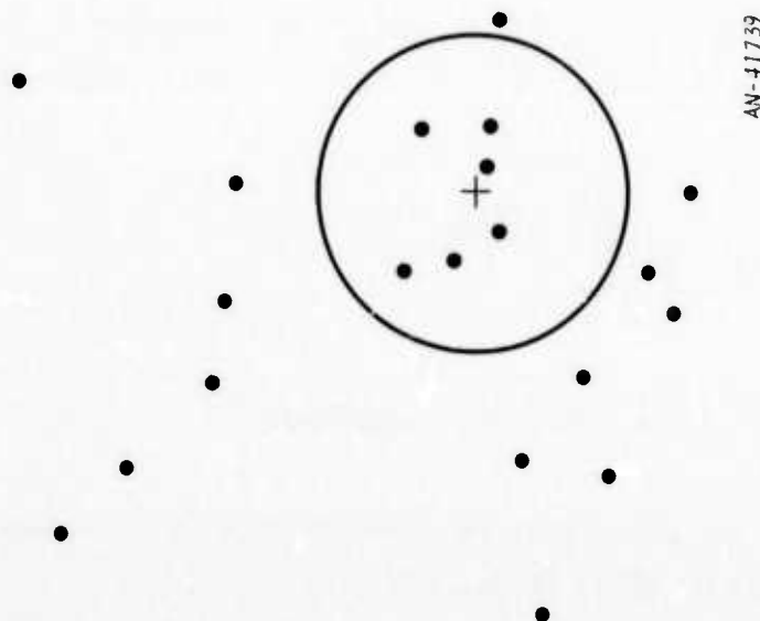
Figure 4.3. The Circle (hypersphere) Found Around the Point of Maximum Probability with Radius 1.5\rho_0 (The center is denoted by +.)
