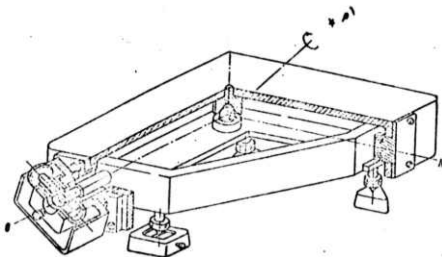
Fig. 23. Equatorial platform for the AFU-75 camera.
