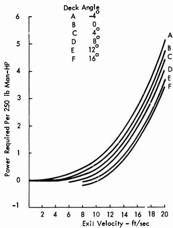
FIGURE D-3. POWER REQUIREMENTS AS A FUNCTION OF EXIT VELOCITY ACCELERATION DISTANCE = 6 FEET
