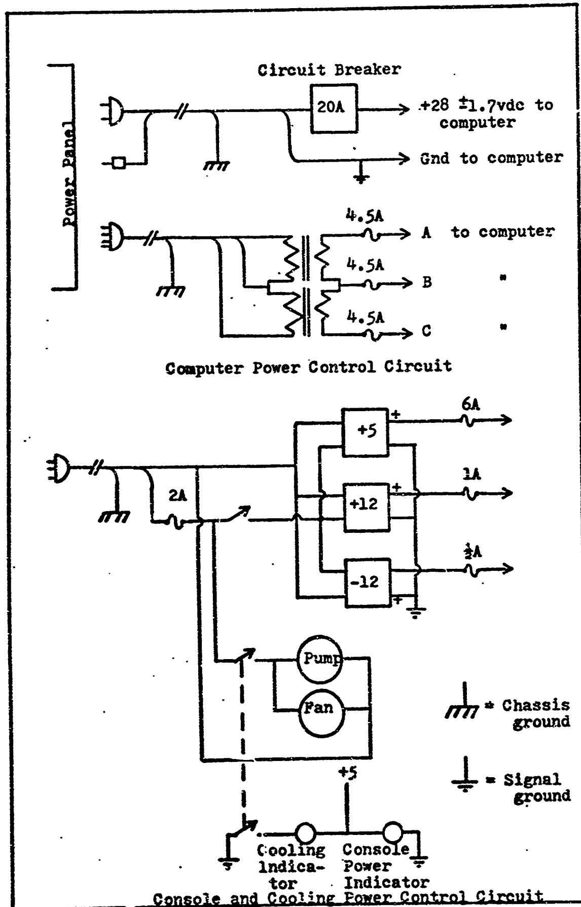
Figure 41. PDU Circuits.
