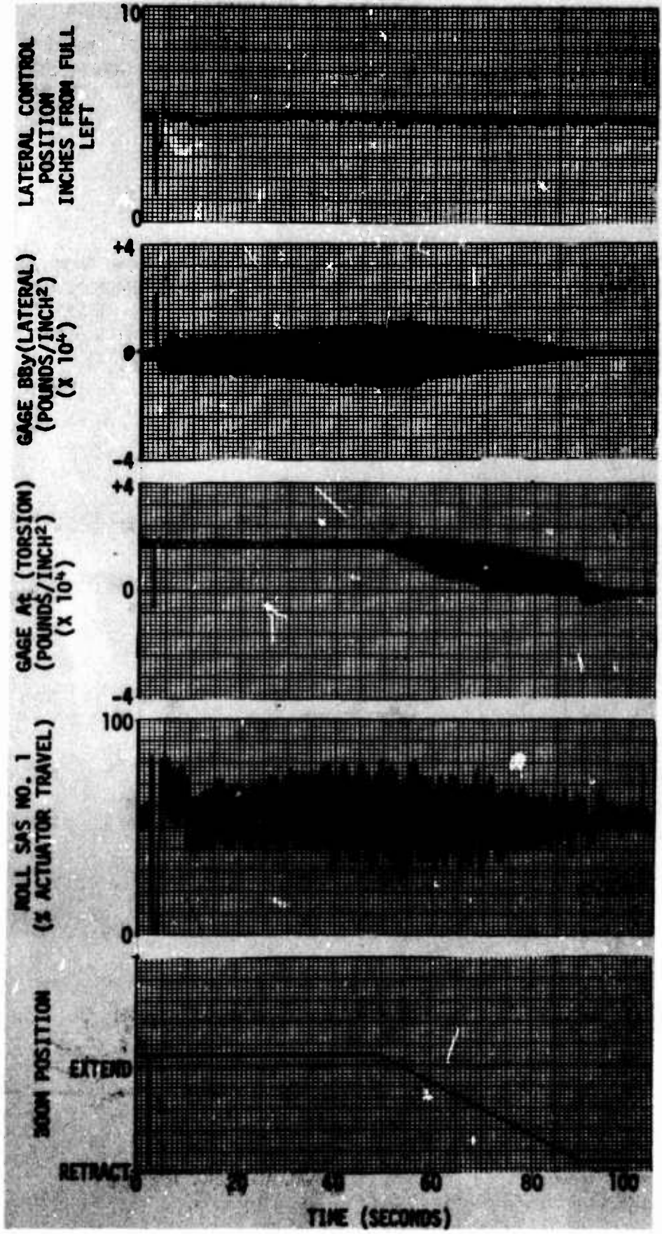
FIGURE C SHORT BOOM DIVERGENCE CH-47C S/N 15814
