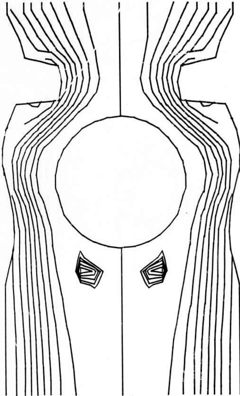
Figure 64 Computer Display of the Contour Plot of the Stream Function for No-Slip Boundary Solution of Blood Flow About a Starr-Edwards Ball Type Valve
