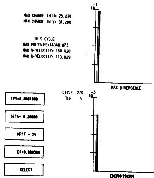
Figure 33 Computer Display of Current State of ABMAC Computation as Produced by Spy Program
