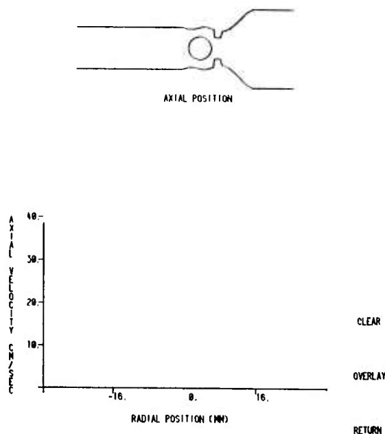
Figure 36 Computer Display of Basic Plot For Velocity Vector Display
