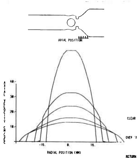
Figure 38 Computer Display of a Series of Velocity Profiles
