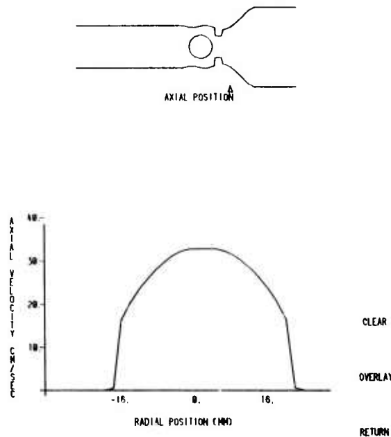
Figure 37 Computer Display of a Typical Velocity Profile
