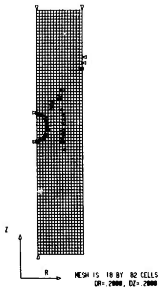
Figure 26 Computer Display of Computational Mesh Showing Points Input to Describe the Curved Boundary
