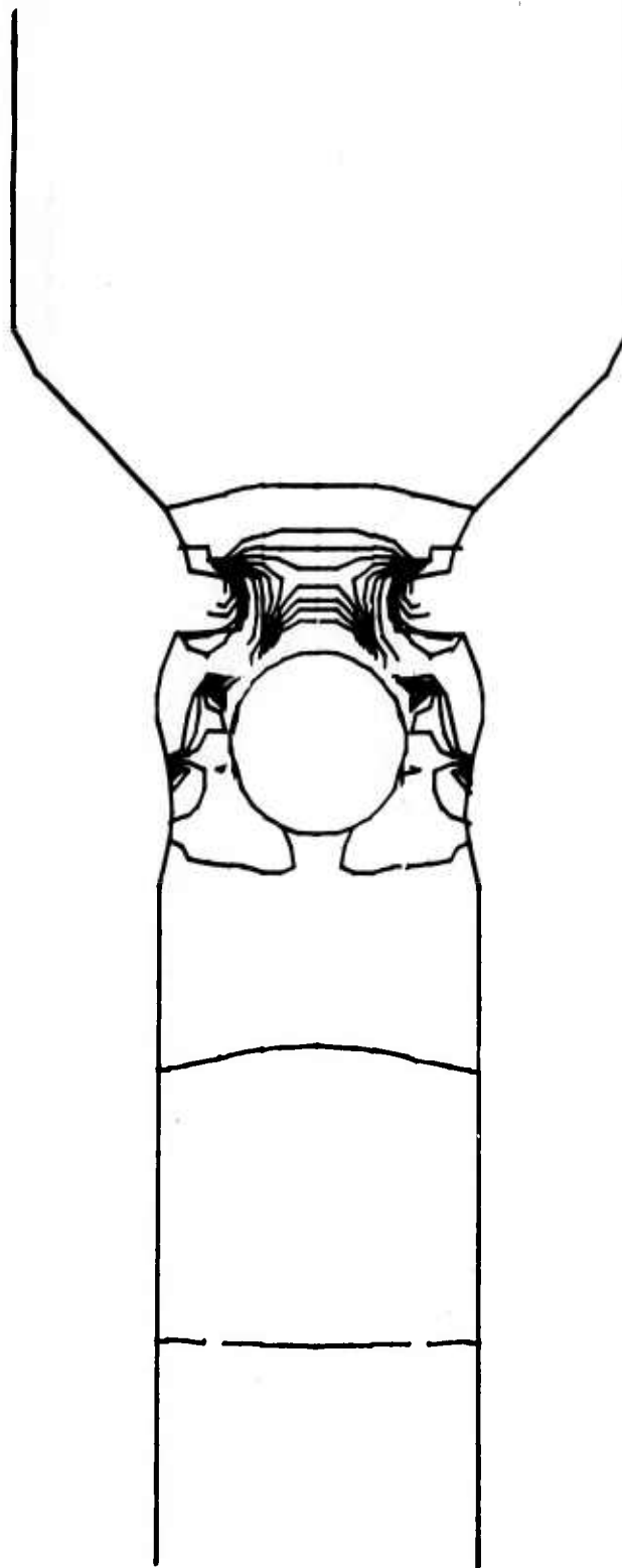
Figure 67 Computer Display of the Contour Plot of the Pressure Field for No-Slip Boundary Solution of Blood Flow About a Starr-Edwards Ball-Type Valve
