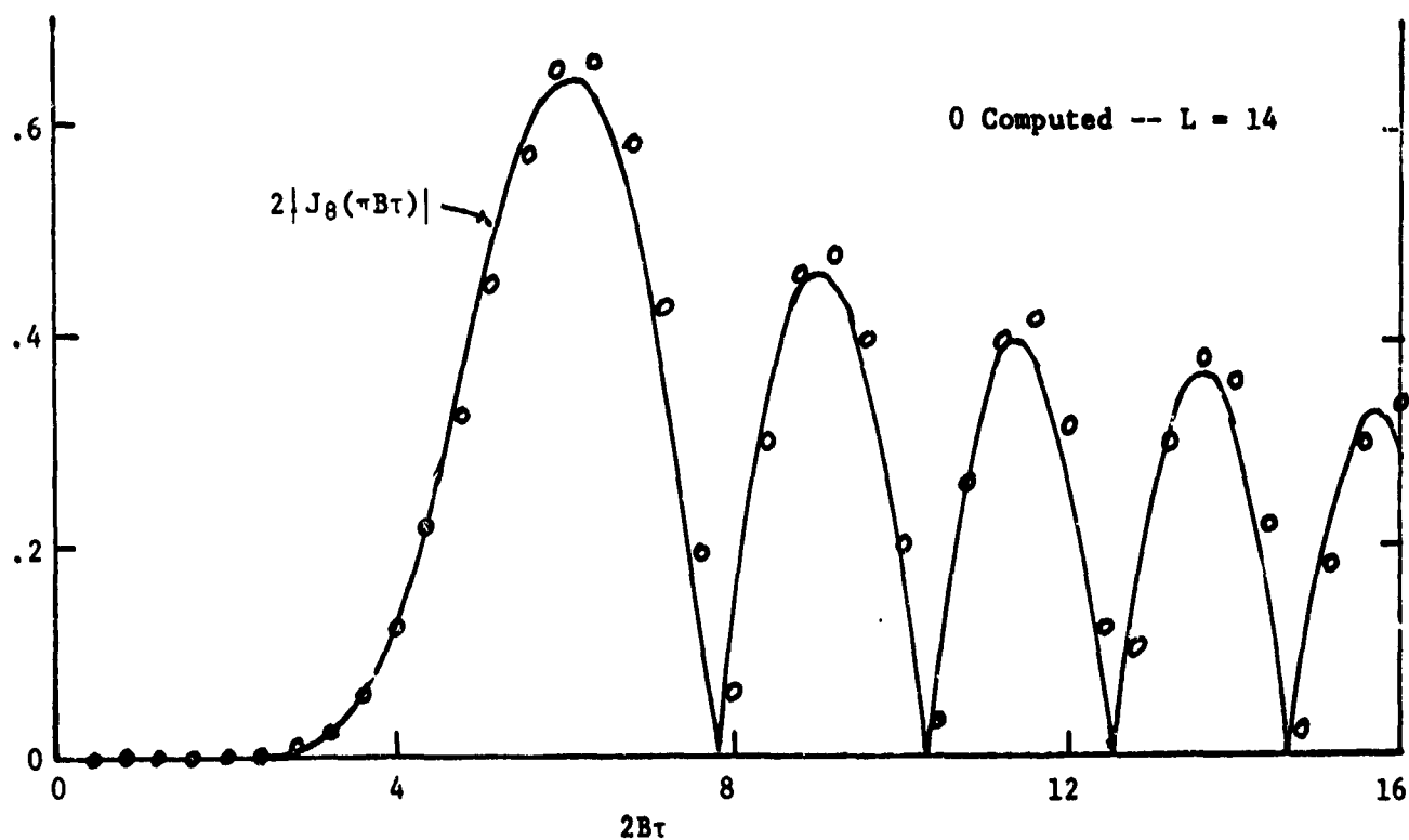
Figure 25. N = 8 Range Law for Ten and Fourteen Section Approximation to Sine Wave Modulation
