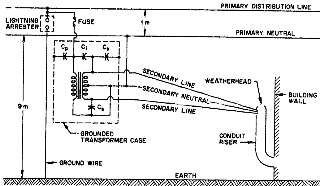
(a) SINGLE PHASE TRANSFORMER AND ASSOCIATED EQUIPMENT
