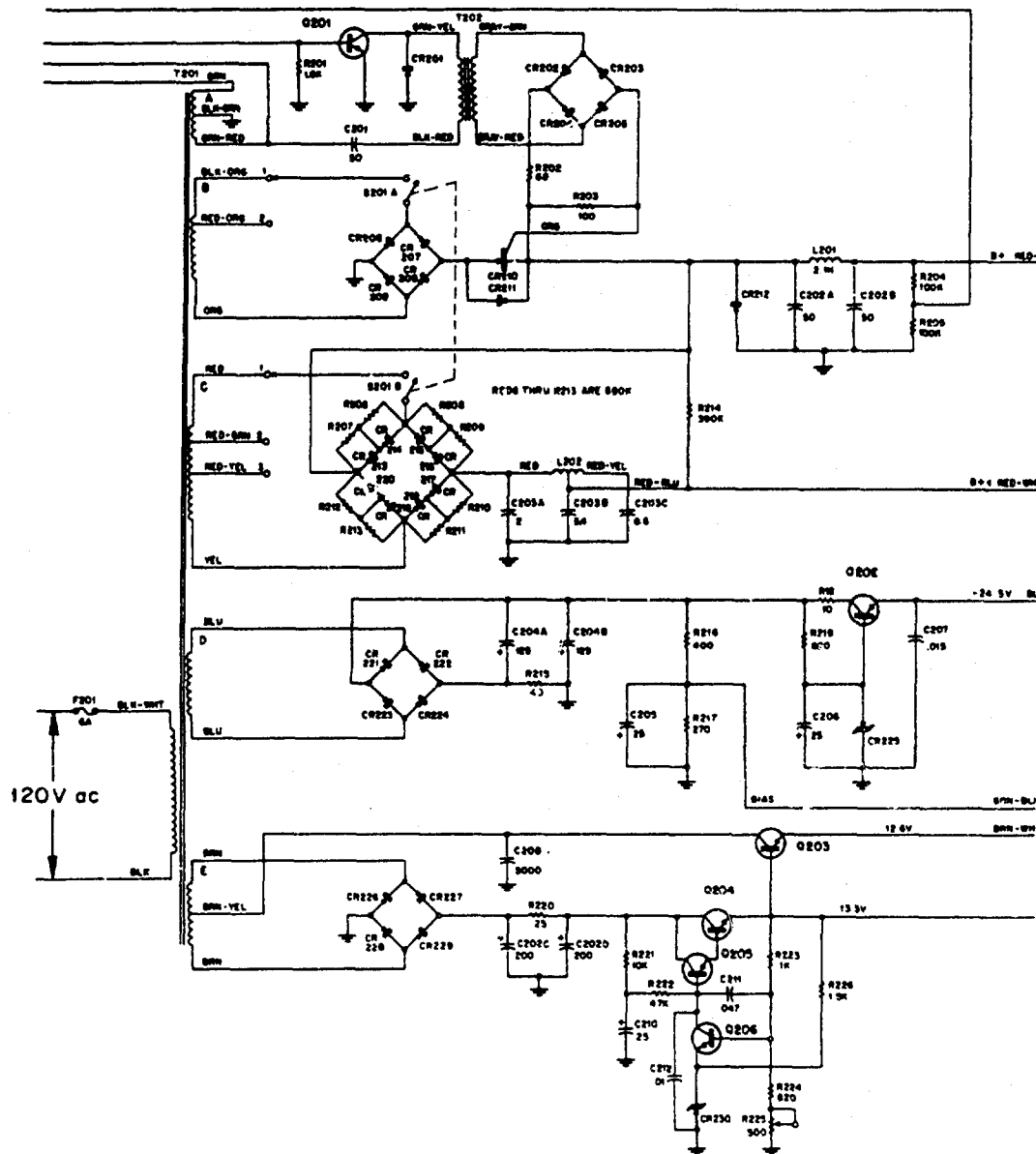
Fig. 3.4 Power Supply Schematic Diagram.
