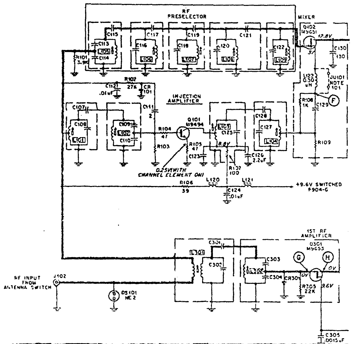
Fig. A-2. Motorola Micor VHF Low Band Receiver Front End Schematic.
