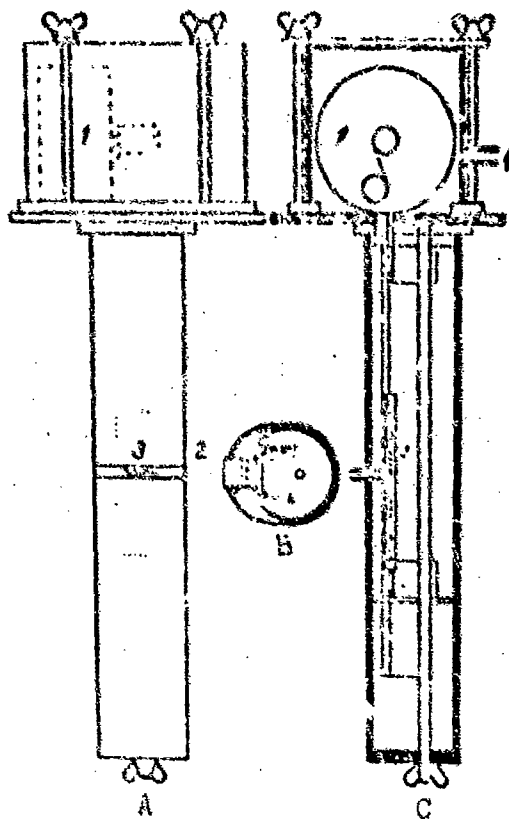
Fig. 4. Hirst trap (diagram). A - front view (upwind side); B - cross section to the intake slot; C - side view (longitudinal section). 1 - clockwork mechanism which moves the plate; 2 - intake slot, turn to face the wind, behind which the holder containing plate (3) moves upward; 4 - to the vacuum pump. (Weathervane unit and cap for protection of the inlet opening from rain are not shown).
