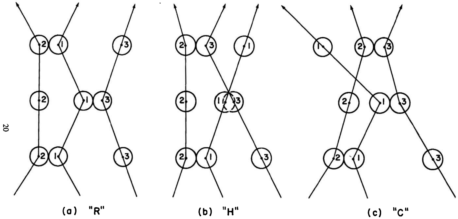
Figure 4. Sequences of three successive collisions among three molecules.
