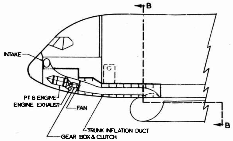
INFLATION SYSTEM
