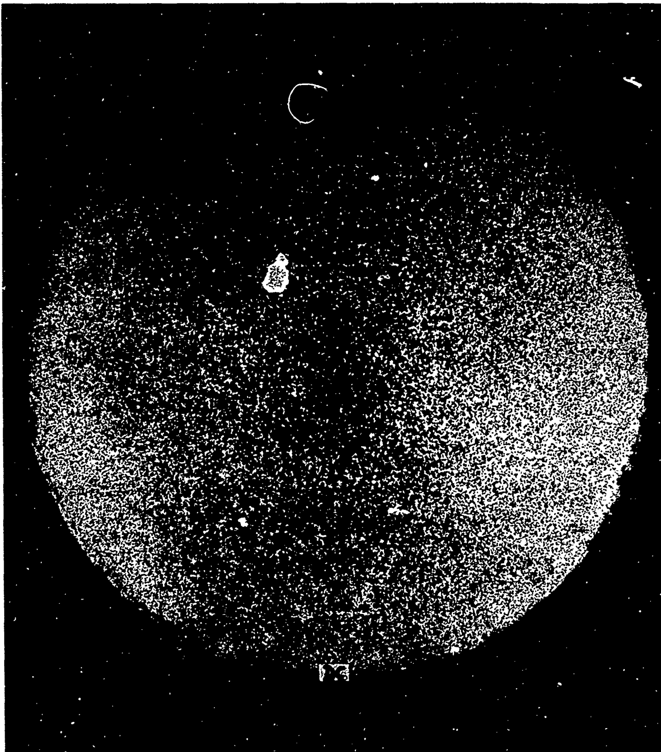
FIGURE 3 7050 INGOT-15" DIAMETER
