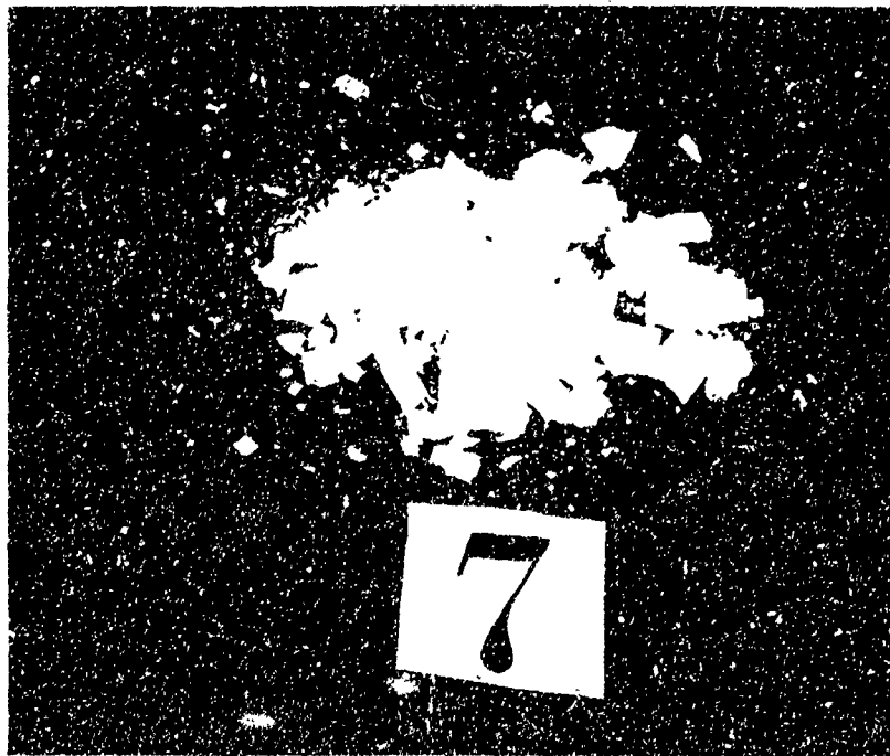
Figure 9a. Fractured tube, path 7, Lot 6A, test T1871.
