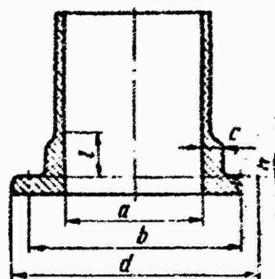
Fig. 66. Monolithic attached flange
