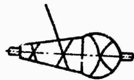
Fig. 78. Combination winding
