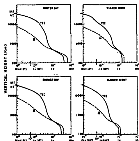
Figure 2-2. Polarization Twist ( Q , in Radians) and Total Electron Content (TEC, in \text{el}/\text{m}^2 ) Along the Slant Path From a Geostationary Satellite to a Mid-Latitude Station
