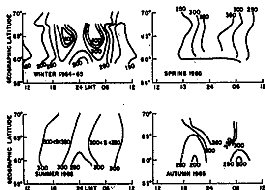
Figure 7-14. Contours of Equivalent Slab Thickness Over Northern Europe - 1965 (after Lyszka, 1967)
