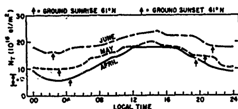
Figure 8-3. Total Electron Content From ATS-3, Thule, Greenland, 1971. Monthly medians
