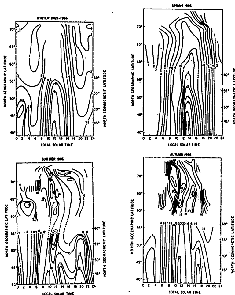
Figure 7-13. Iso-Contours of Seasonal Median Total Electron Content Taken Over Northern Europe in 1966 (After Amayenc et al, Annales de Geophysique , 1971)
