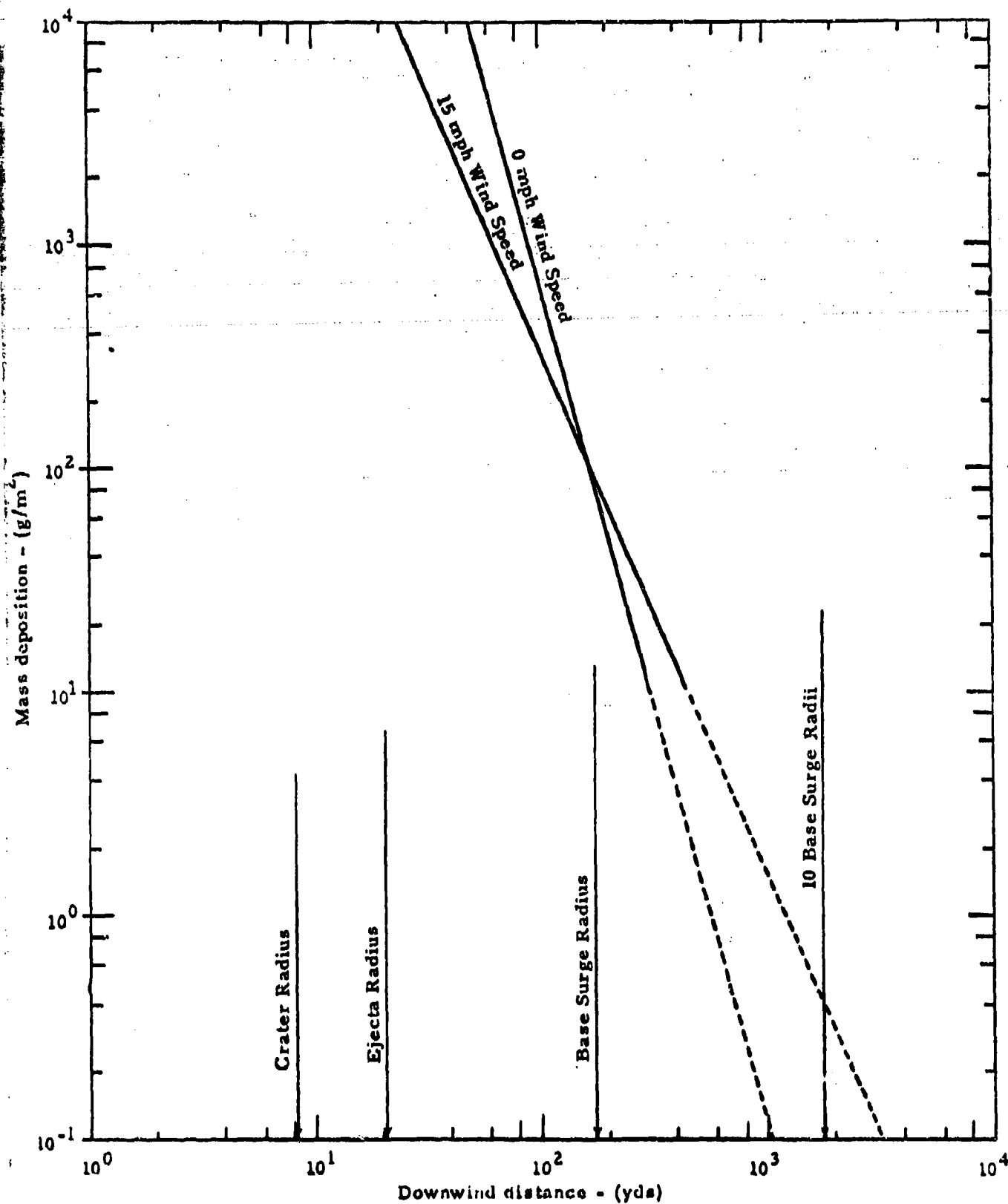
Figure 9. Predicted mass deposition versus downwind range for Trinity.
