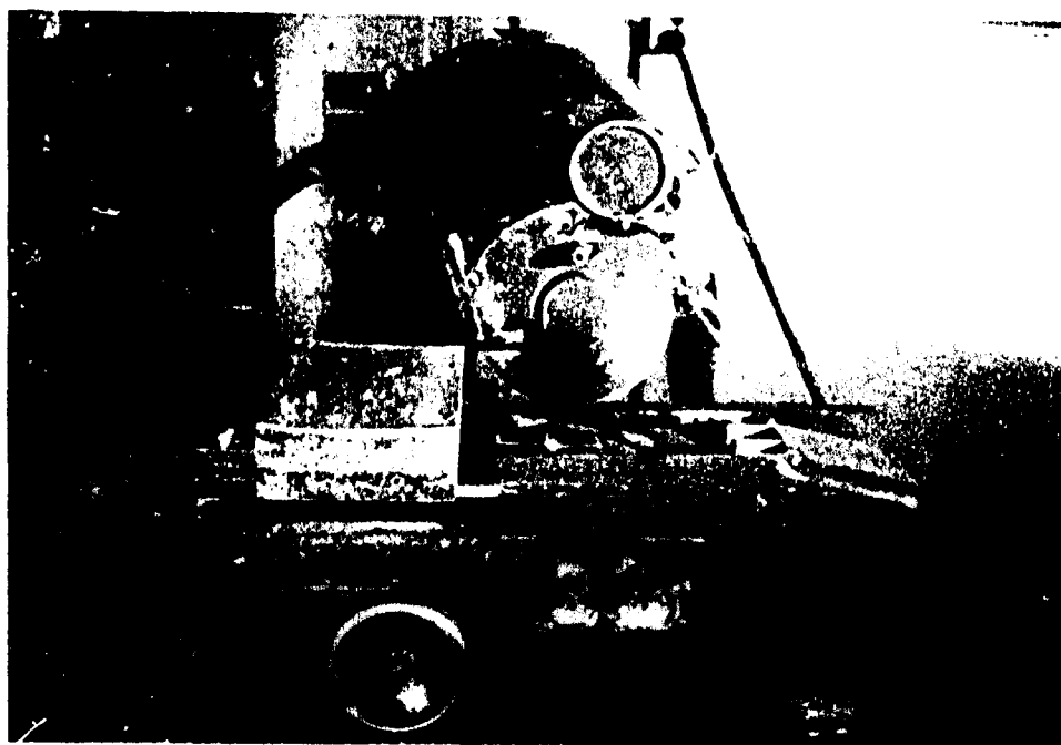
Figure 4. Diamond-bladed saw used to cut joint blocks.
