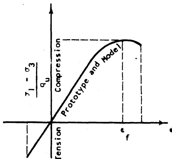
Figure A8. Dimensionless prototype and model stress-strain curve.
