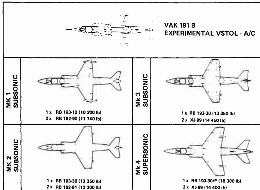
FIG. 29 VAK 191 B, GROWTH POTENTIAL VARIANTS
