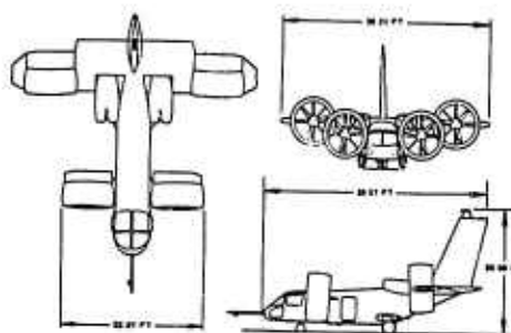
FIGURE 4. X-22 THREE - VIEW
