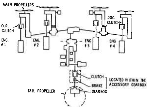
FIGURE 5. XC-142 DRIVE SYSTEM
