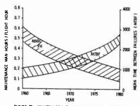
FIGURE 23. MAINTAINABILITY AND RELIABILITY TRENDS DIRECTIONS
