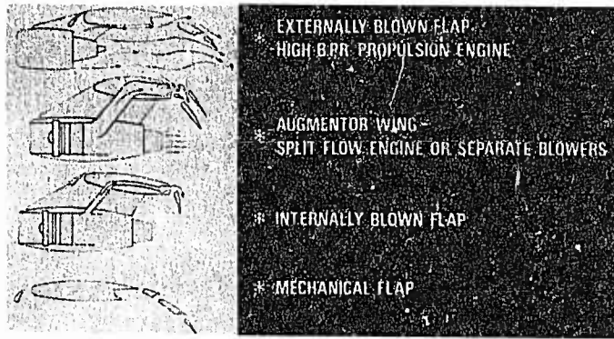
Fig. 15. Lift Systems.
