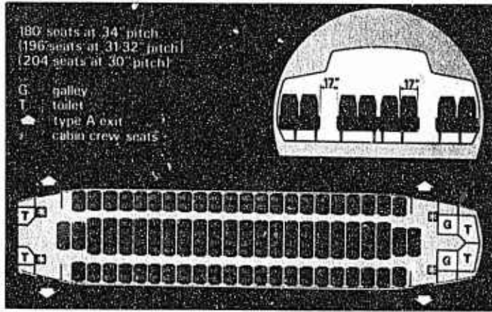
Fig. 4 Accommodation Layout.
