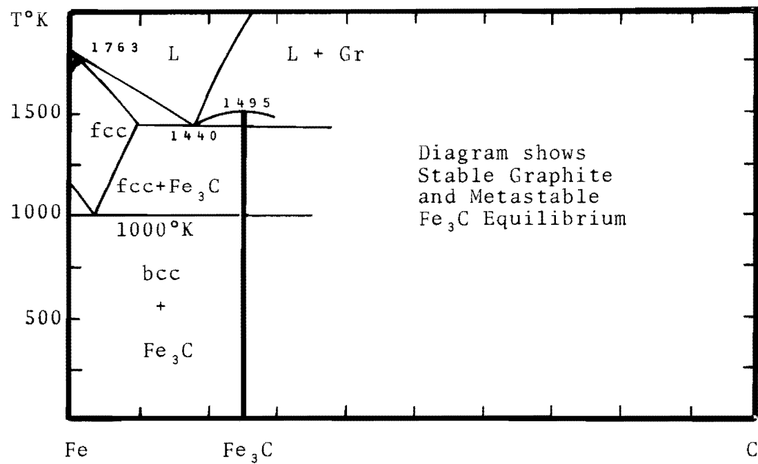
Figure 38 Calculated Phase Diagram for the Fe-C System.
