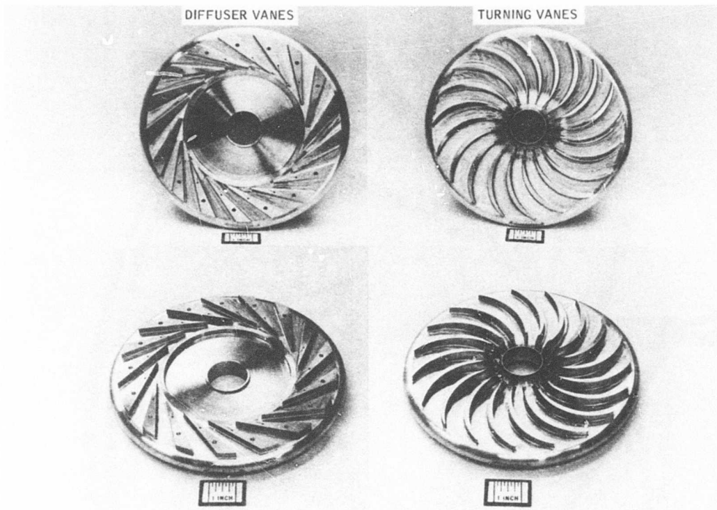
Figure 13. Interstage Crossover Assembly.
