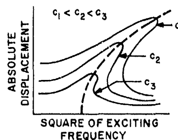
Fig. 3-5. Nonlinear characteristics.
