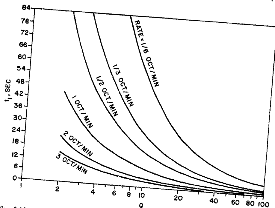
Fig. 3-12. Time spent in passing through a resonance using a logarithmic sweep rate [59].
