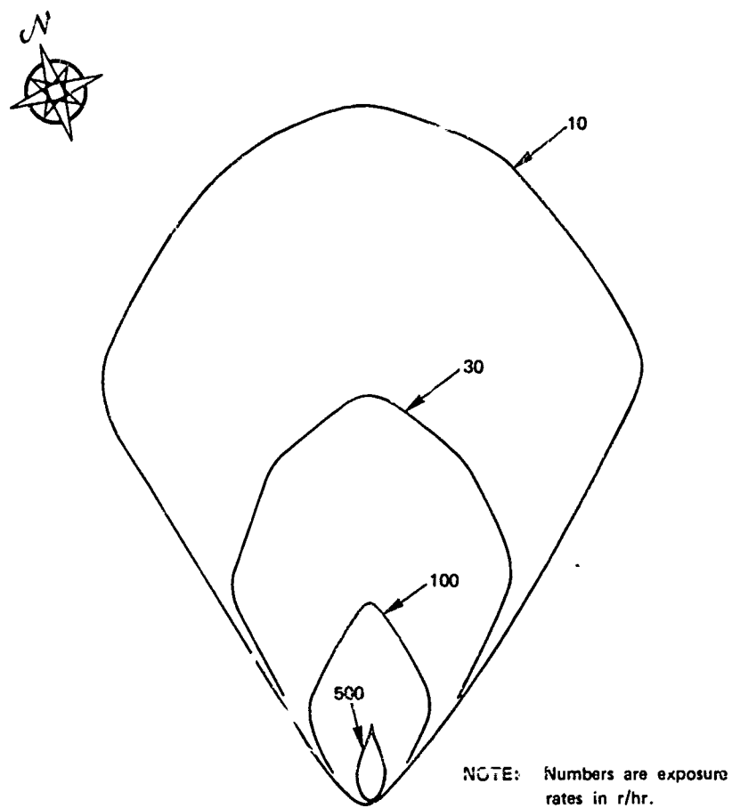
FIGURE 6 SEER FALLOUT PATTERN WITH MOCK WIND — 2 MT
