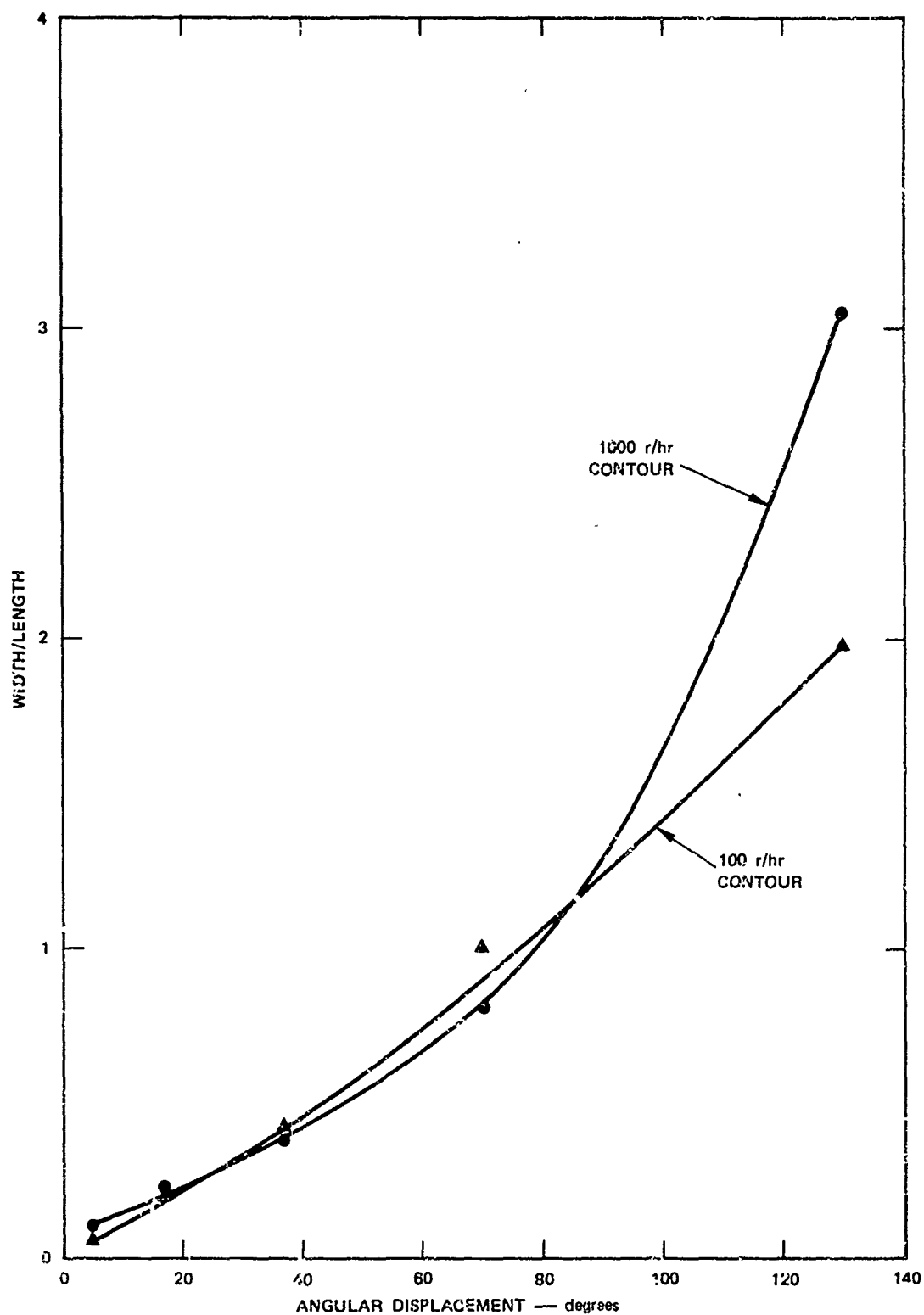
FIGURE 30 WIDTH/LENGTH RATIOS VERSUS EFFECTIVE WIND ANGULAR DISPLACEMENT
