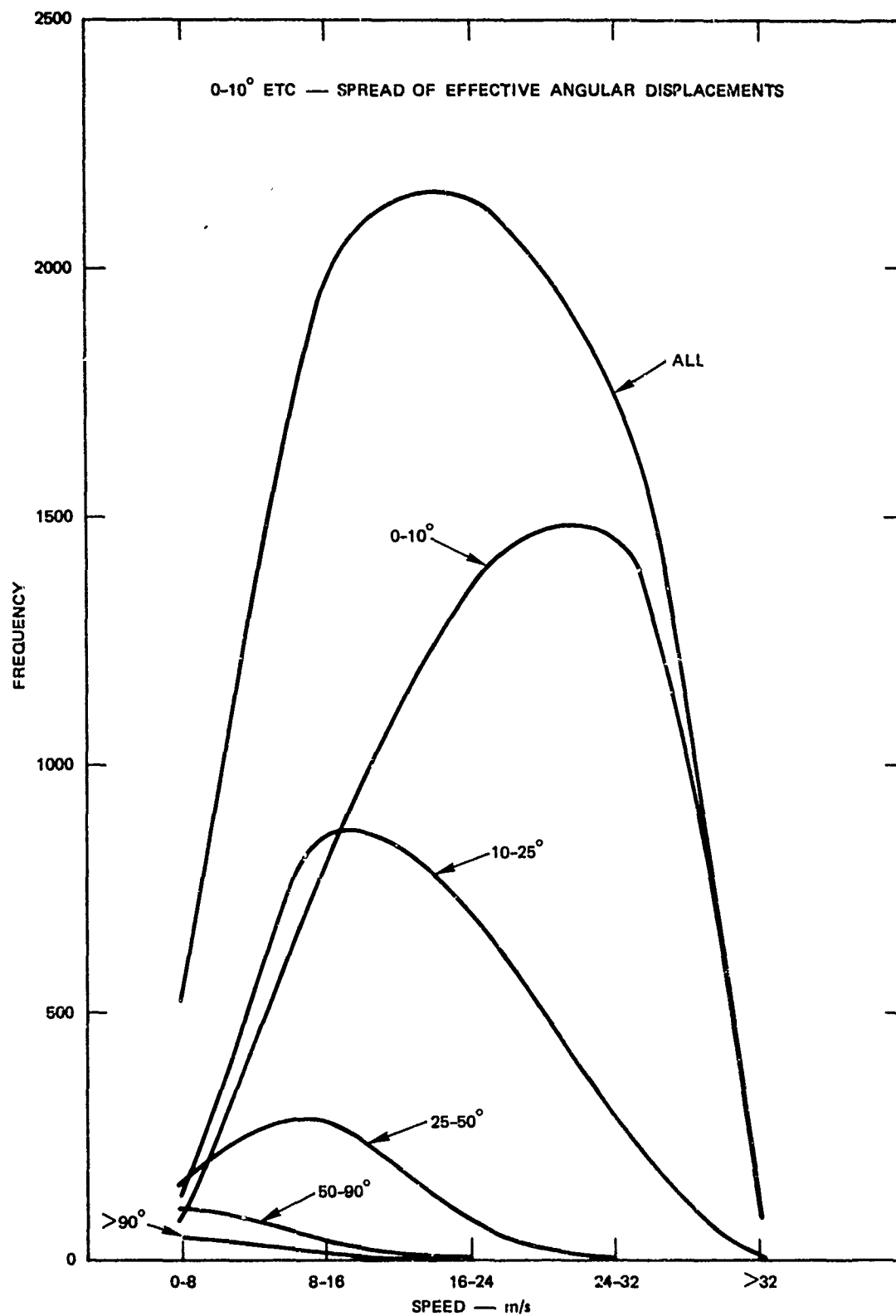
FIGURE 26 DISTRIBUTION OF WIND SPEEDS OVER PEORIA
