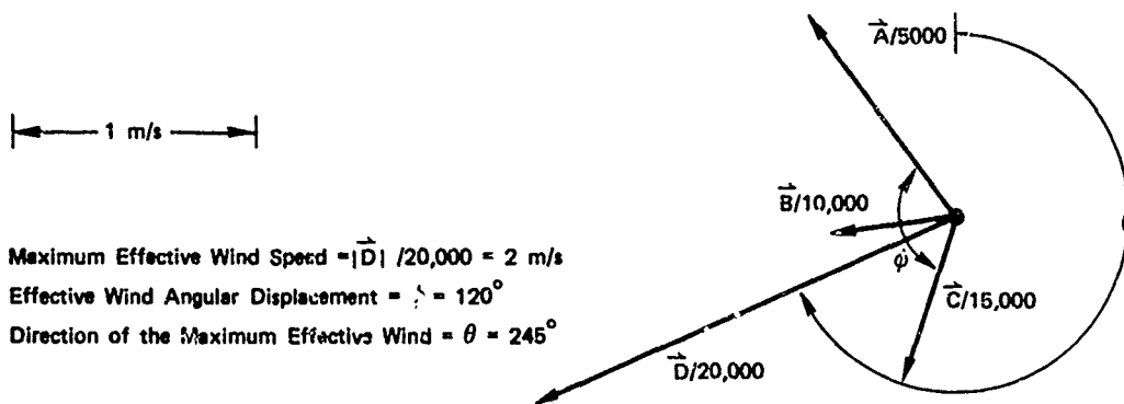
(c) AVERAGE HORIZONTAL VELOCITY VECTORS DURING FALL
