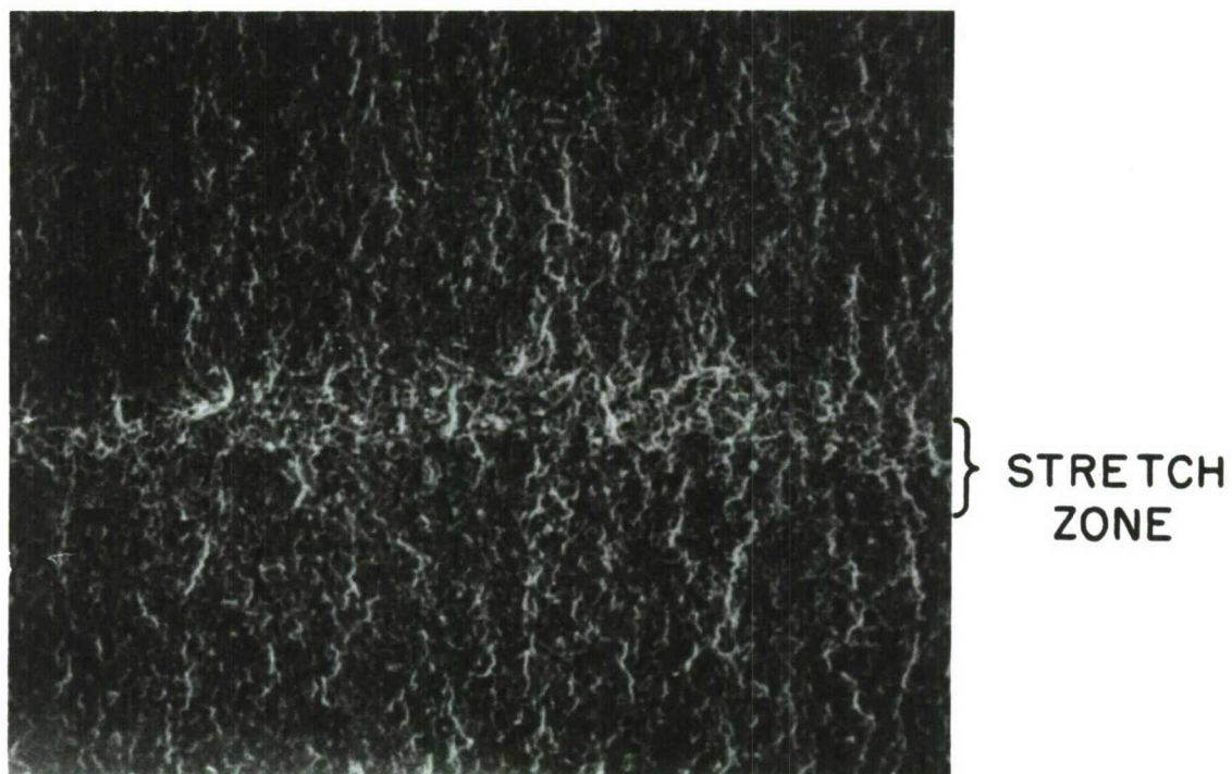
Figure 20. Overload Stretch Zones (125X) Top: 50% Overload (Specimen CG-14); Bottom: 100% Overload (Specimen CG-14)
