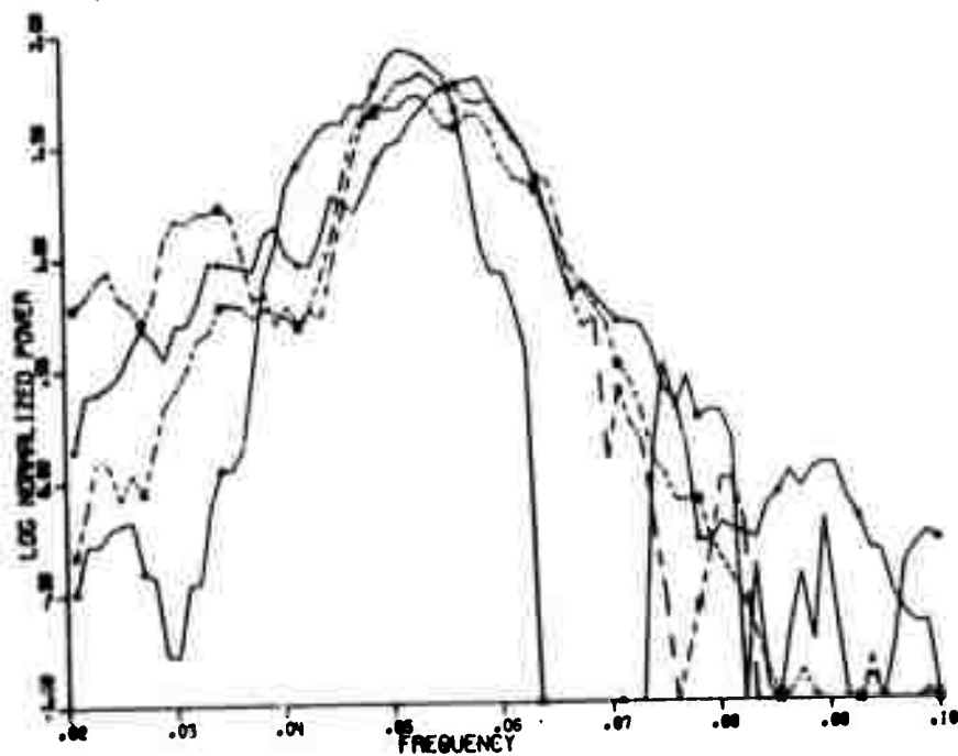
Figure 33. Rayleigh-Wave Spectra at Station TFO.
