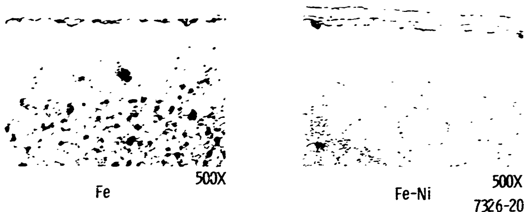
Figure 19. Vacuum diffusion zone.
