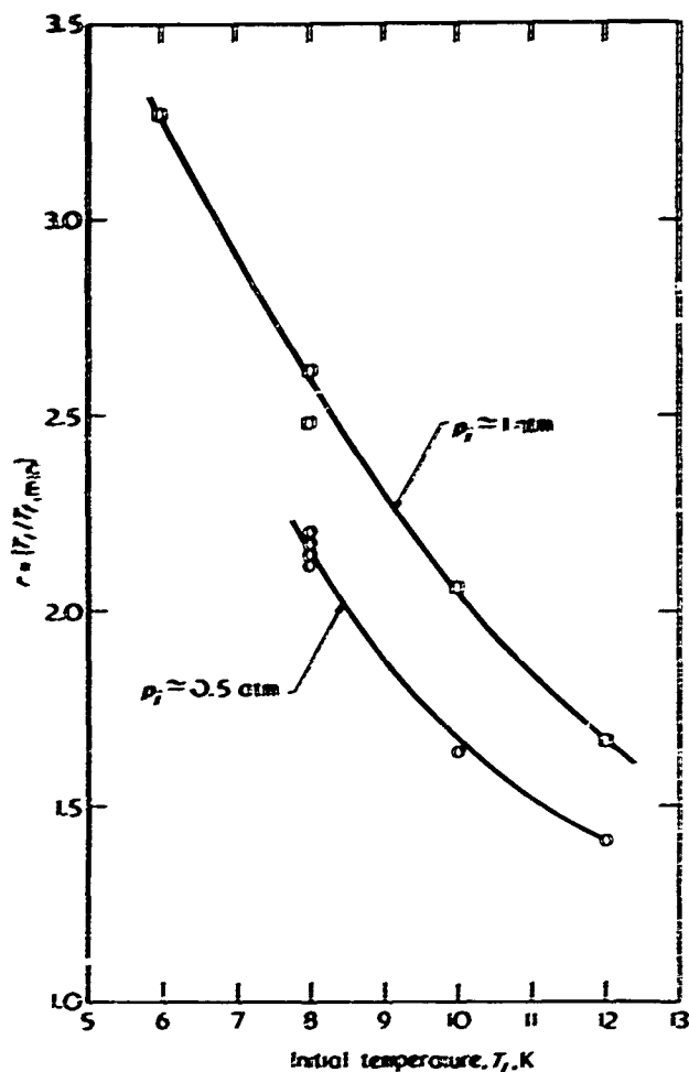
Fig. 4 Plot of the observed r values ( r = T_i/T_{f,min} ) versus initial temperature, T_i , for two initial pressures p_i = 0.5 \text{ atm} approx and p_i = 1 \text{ atm} approx. The data were taken using the mechanical pump only
