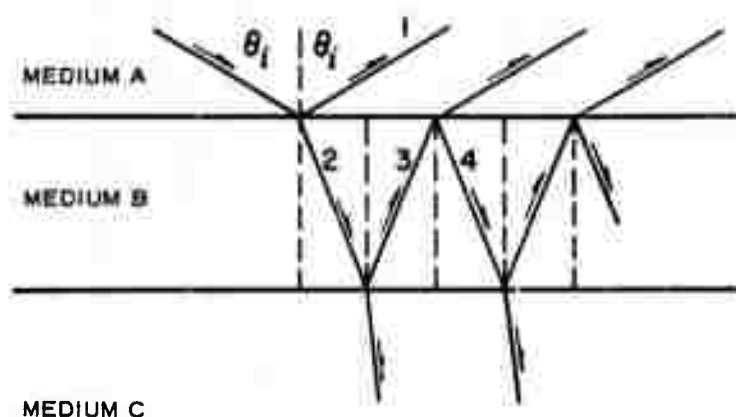
Figure 12. Schematic diagram of multiple reflections and refractions taking place in a snow layer over land or ice surfaces.
