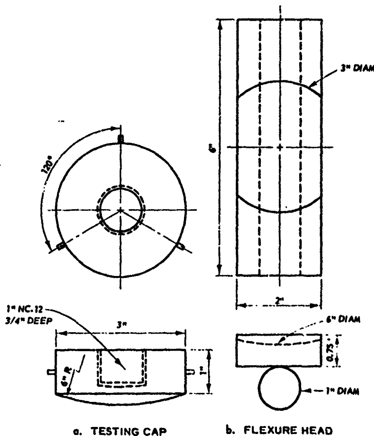
Fig. B1. Sketch of flexure head and testing cap
