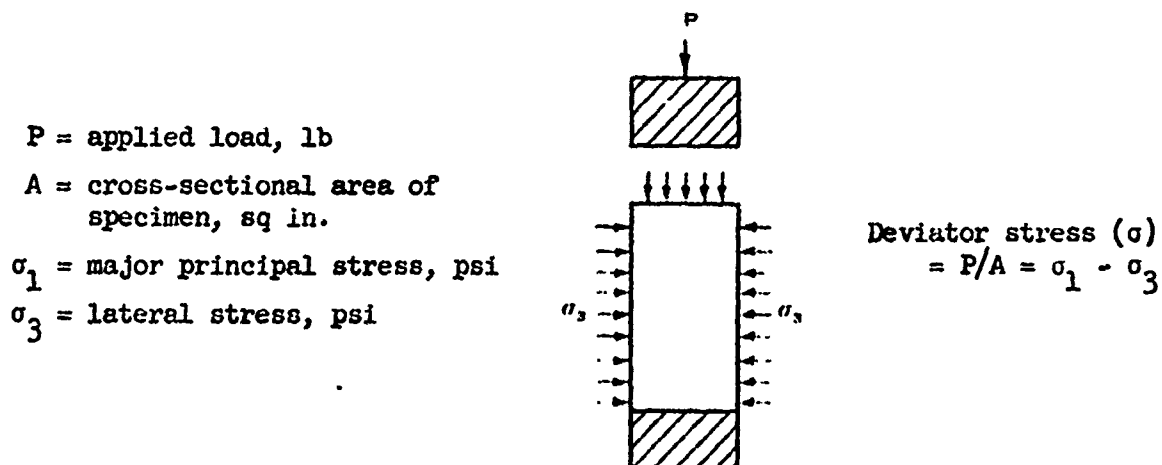
Fig. A1. Diagram of stresses during triaxial test
