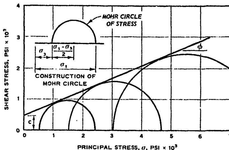
Fig. A5. Determination of shear strength parameters
