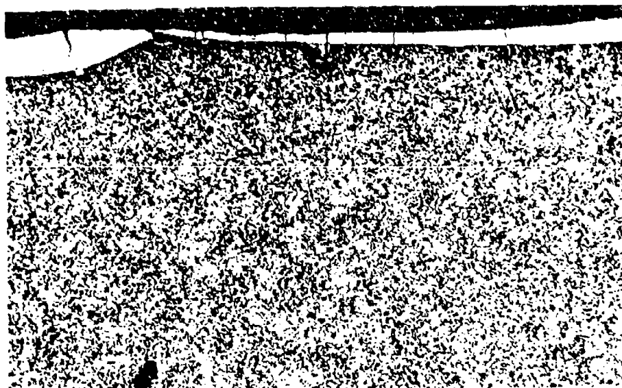
FIGURE 52 TRANSVERSE SECTION AT 10 INCHES FROM THE CHAMBER OF A STANDARD CHROME-PLATED GUN BARREL AFTER FIRING 11,283 ROUNDS AND BEING DECLARED UNSERVICEABLE.
