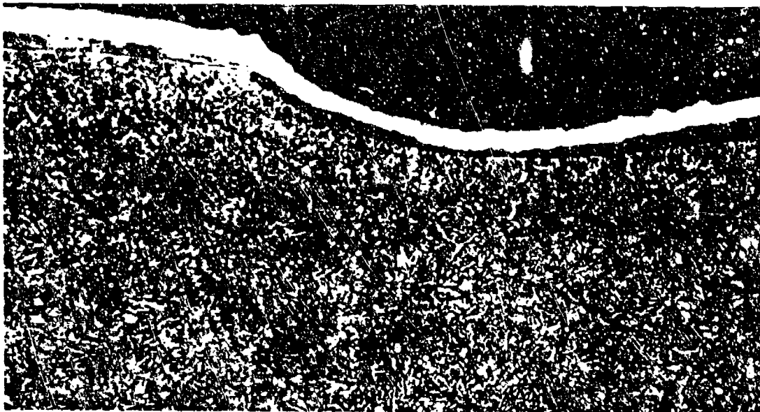
FIGURE 8 PHOTOMICROGRAPH REVEALING THE TRANSVERSE STRUCTURE ALONG THE BORE SURFACE OF AN UNPLATED RIFLED INSERT AFTER 5 VENTED BOMB SHOTS WITH WC846 PROPELLANT.
