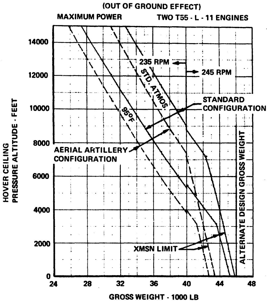
Figure 39. CH-47C Helicopter Hover Ceiling Versus Gross Weight
