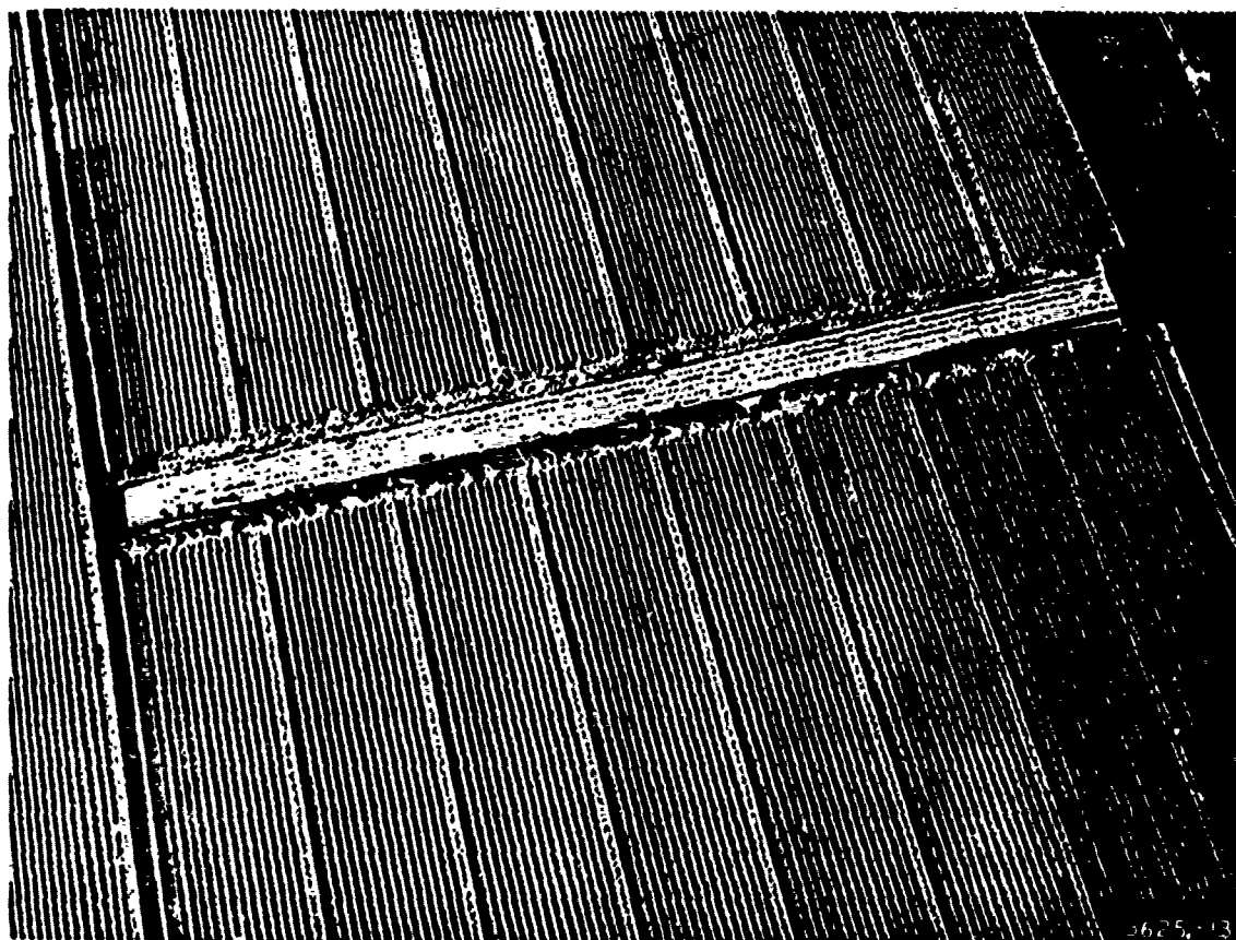
Fig. 10. Cracks at end joint and overlapping corner break in item 1 after 20 coverages of traffic
