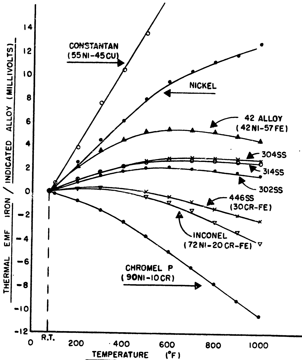
FIGURE 1. THERMAL E.M.F. OF IRON VS VARIOUS ALLOYS REFERENCED TO ROOM TEMPERATURE
