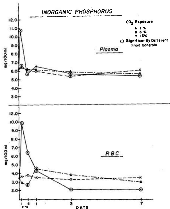
Fig. 8. Summary of Total Plasma and RBC Inorganic Phosphorus of Guinea Pigs Exposed to 1%, 3%, and 15% \text{CO}_2 . Statistical Significance at the 5% Level or Better
