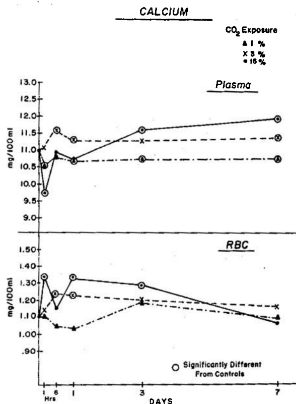
Fig. 7. Summary of Total Plasma and RBC Calcium of Guinea Pigs Exposed to 1%, 3%, and 15% \text{CO}_2 . Statistical Significance at the 5% Level or Better
