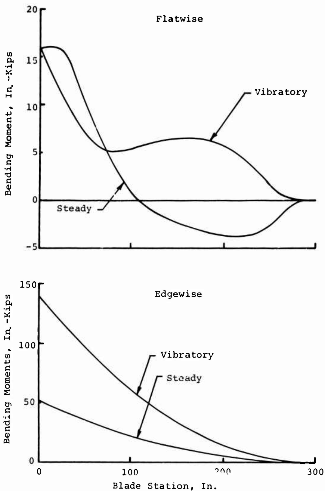
Figure 23 Flatwise and Edgewise Flight Loading for Configuration II Blade.
