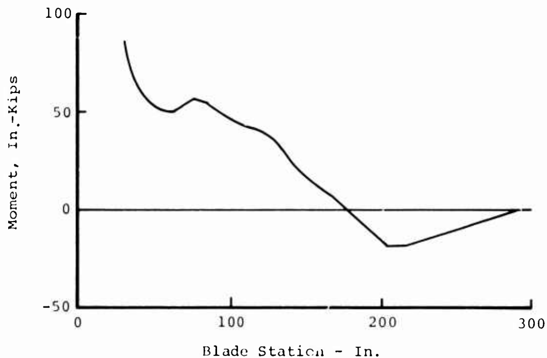
(b) Steady Edgewise Moment Due to Centrifugal Force at a Rotor Speed of 315 rpm for the UH-1H Blade.
