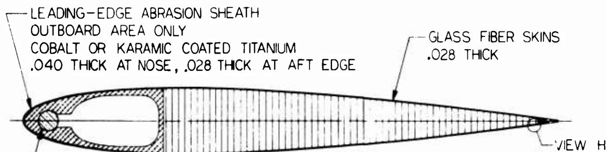
SECTION C-C TYPICAL OUTBOARD SECTION
