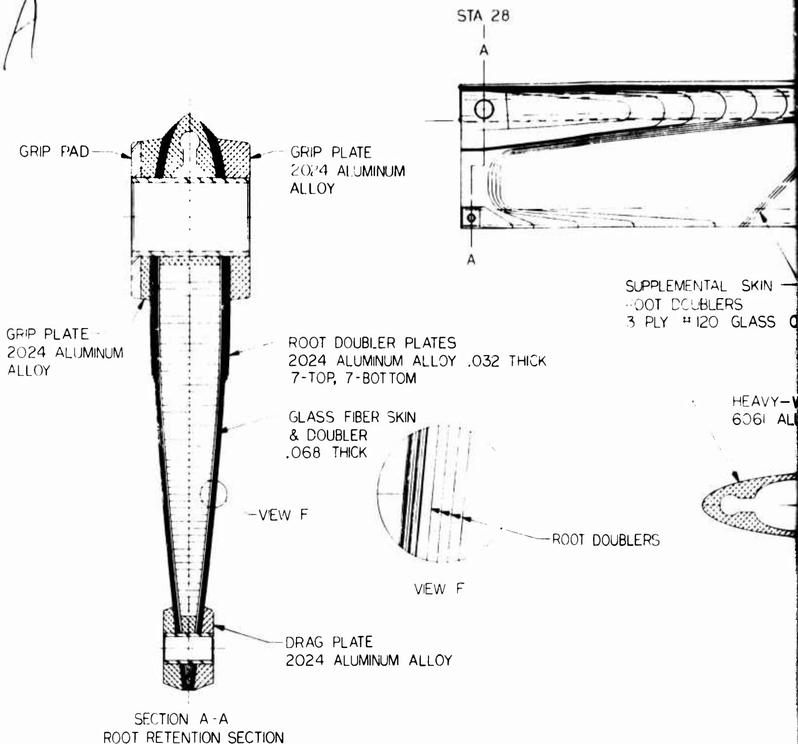
Figure 6. Configuration V, Selected Repairable Rotor Blade Design.
