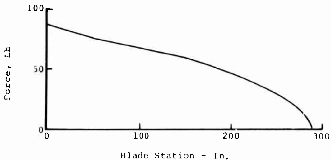
(a) Centrifugal Force at a Rotor Speed of 315 rpm for the UH-1H Blade.
