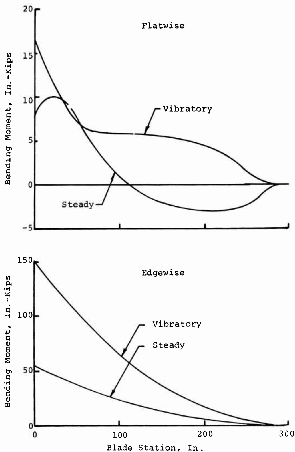
Figure 25. Flatwise and Edgewise Flight Loading for Configuration IV Blade.
