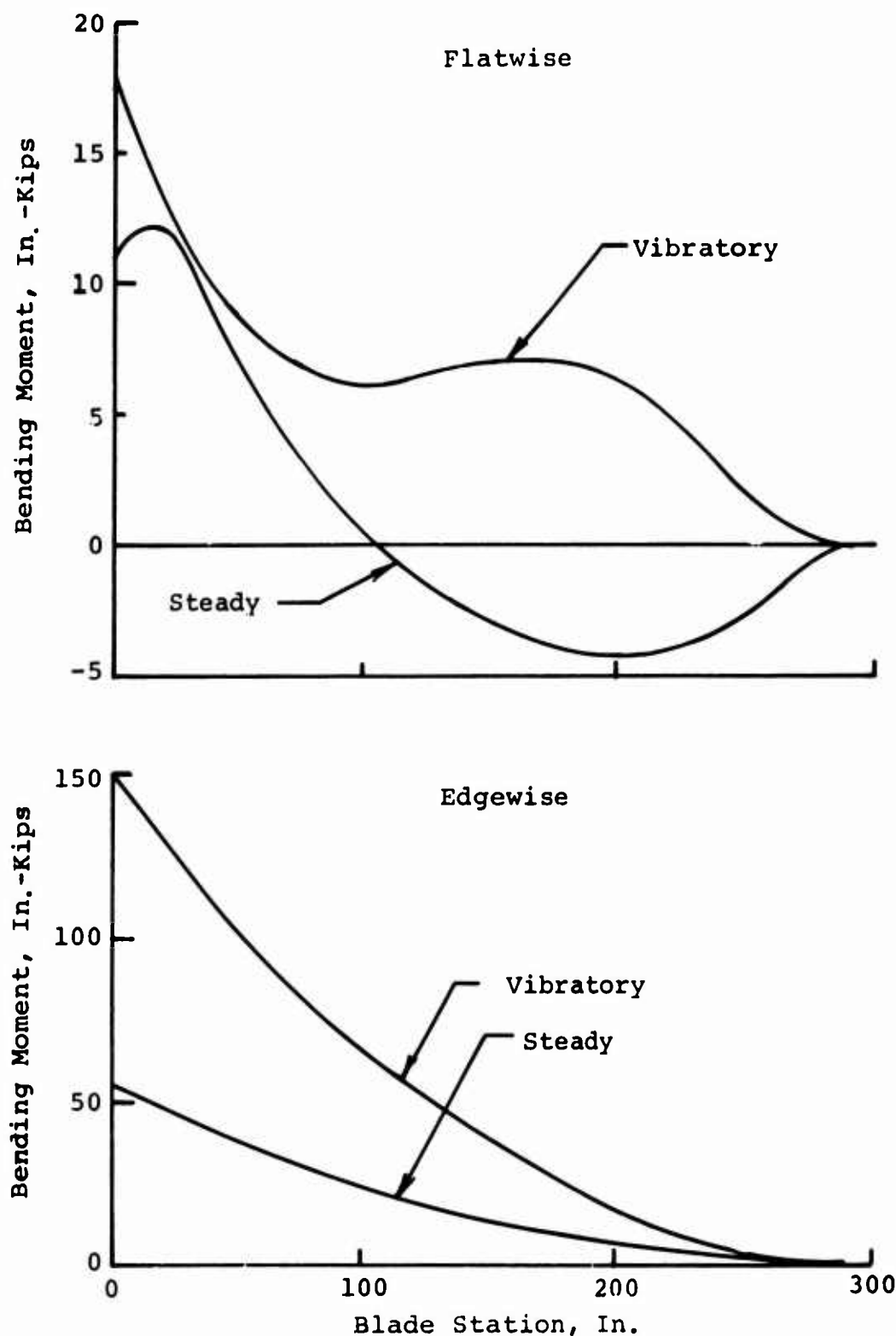
Figure 21. Flatwise and Edgewise Flight Loading for the Current UH-1H Blade.
