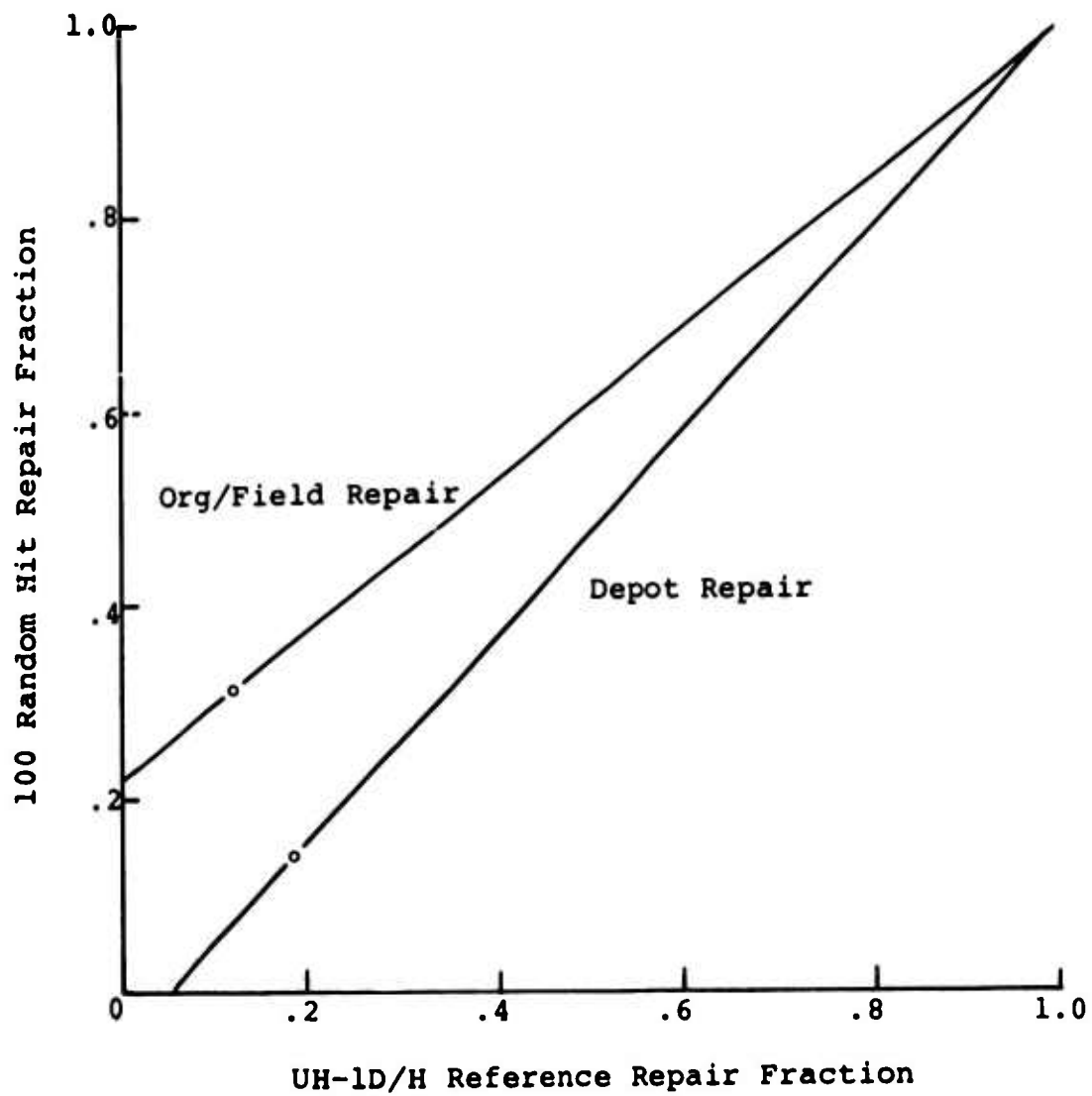
Figure 13. Blade Repair Analysis Adjustment.
