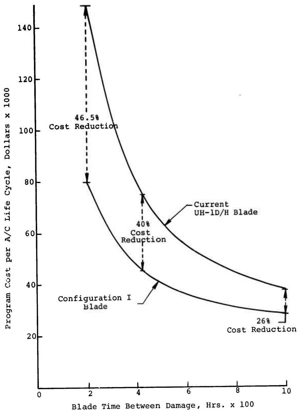
Figure 14. Program Cost With Varying Blade Time Between Damage.
