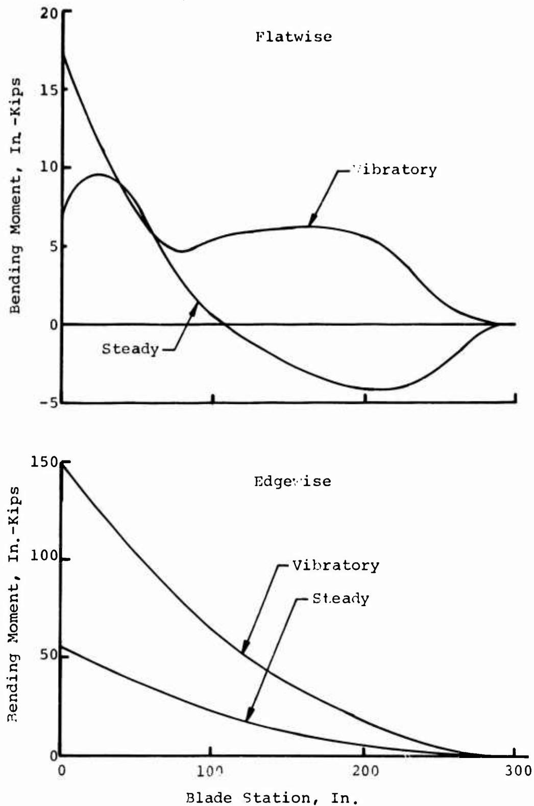
Figure 24. Flatwise and Edgewise Flight Loading for Configuration III Blade.
