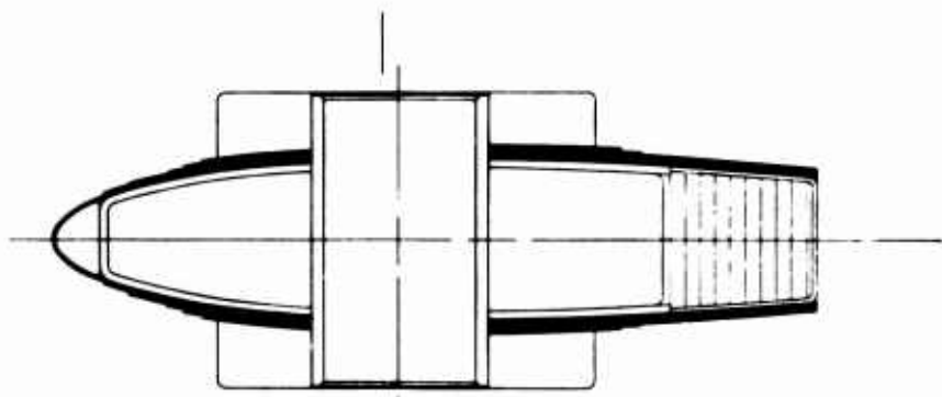
SECTION A MAIN RETENTION PIN AREA
