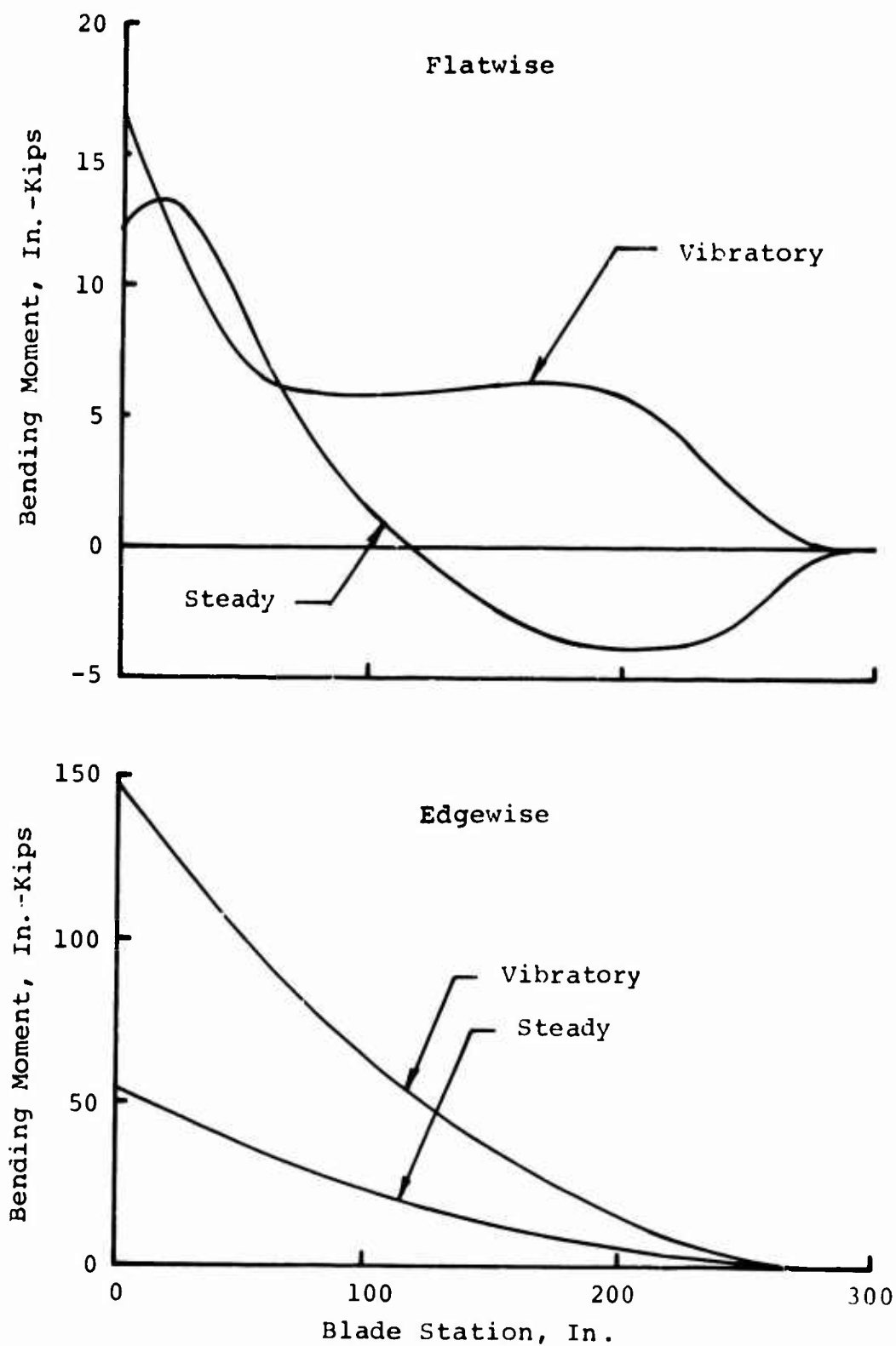
Figure 22. Flatwise and Edgewise Flight Loading for the Configuration I Blade.
