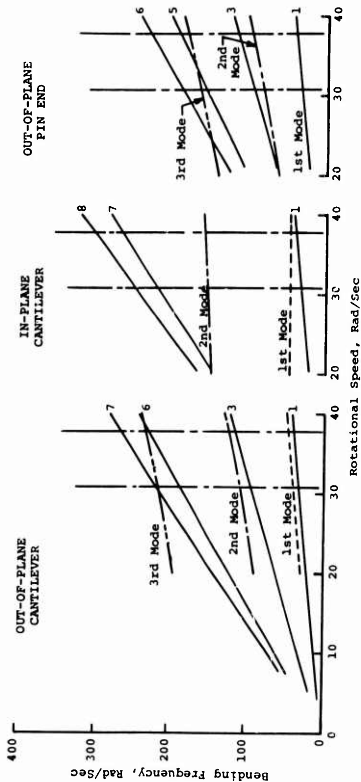
Figure 16. Natural Frequencies of Current UH-1H Blade.
