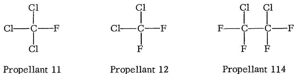
Figure 1. CHEMICAL STRUCTURES OF THREE FLUOROCARBON PROPELLANTS.
