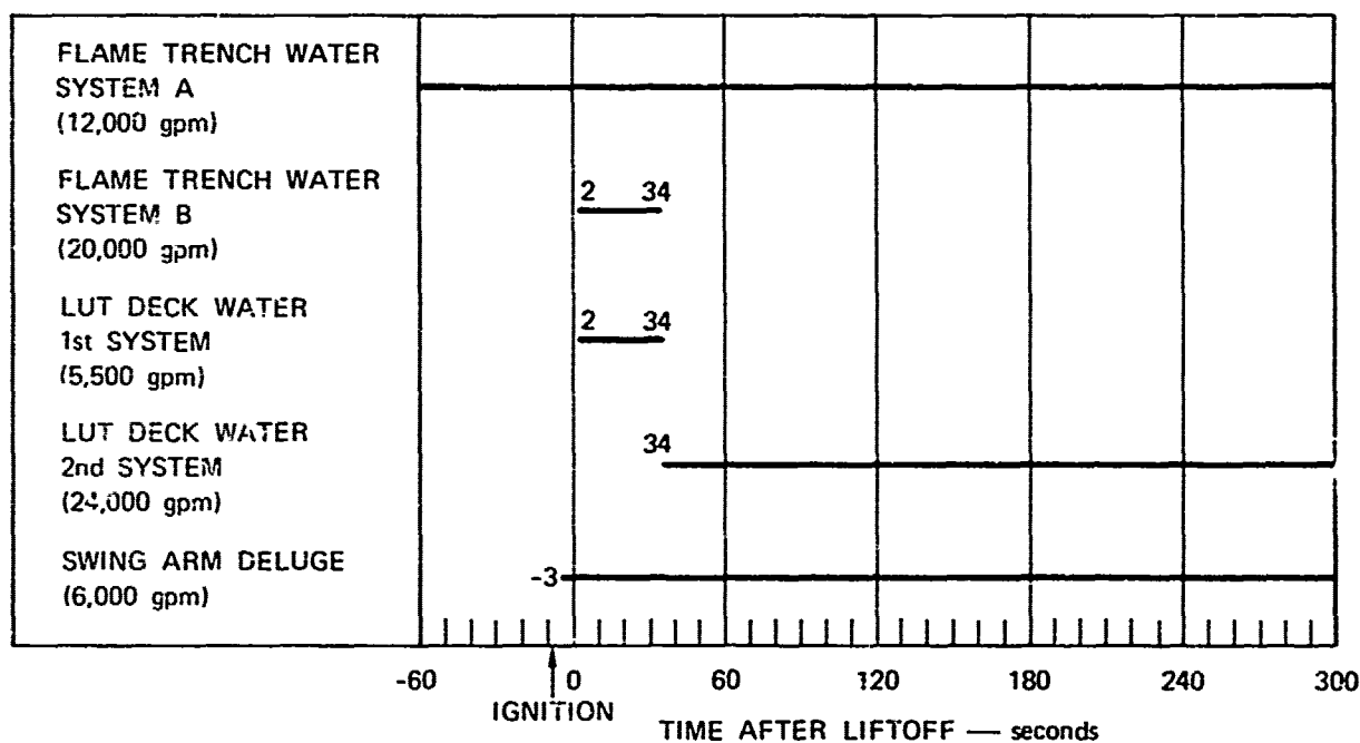
FIGURE 25 ACTIVITY OF PAD WATER-DELUGE SYSTEM DURING APOLLO LAUNCH
