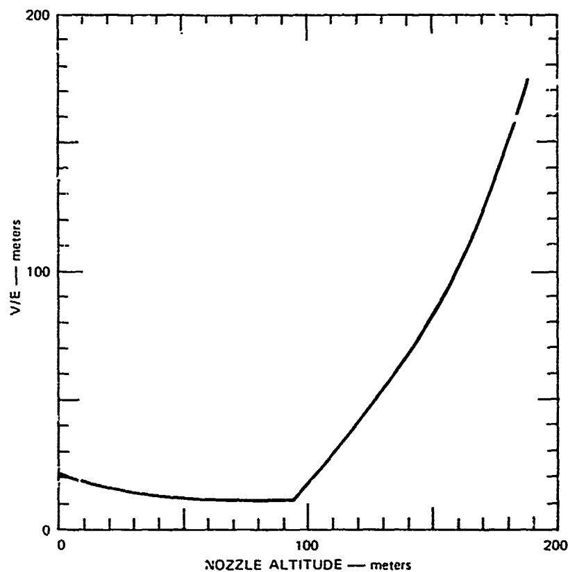
FIGURE 15 RELATIONSHIP BETWEEN ROCKET POTENTIAL AND LUT-FACE FIELD AT FIELD-METER POSITION
