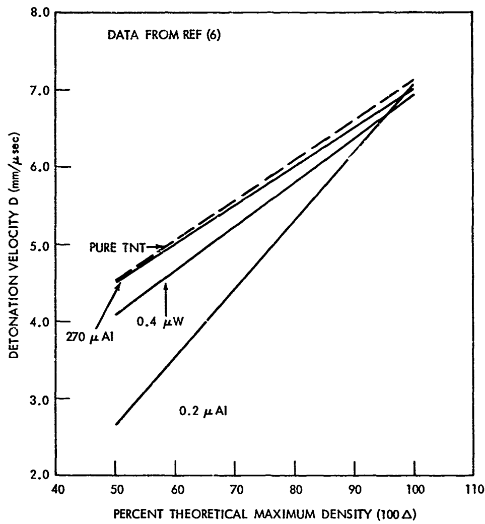
FIG. 3 EFFECT OF 15% DILUENT ON DETONATION VELOCITY OF TNT
