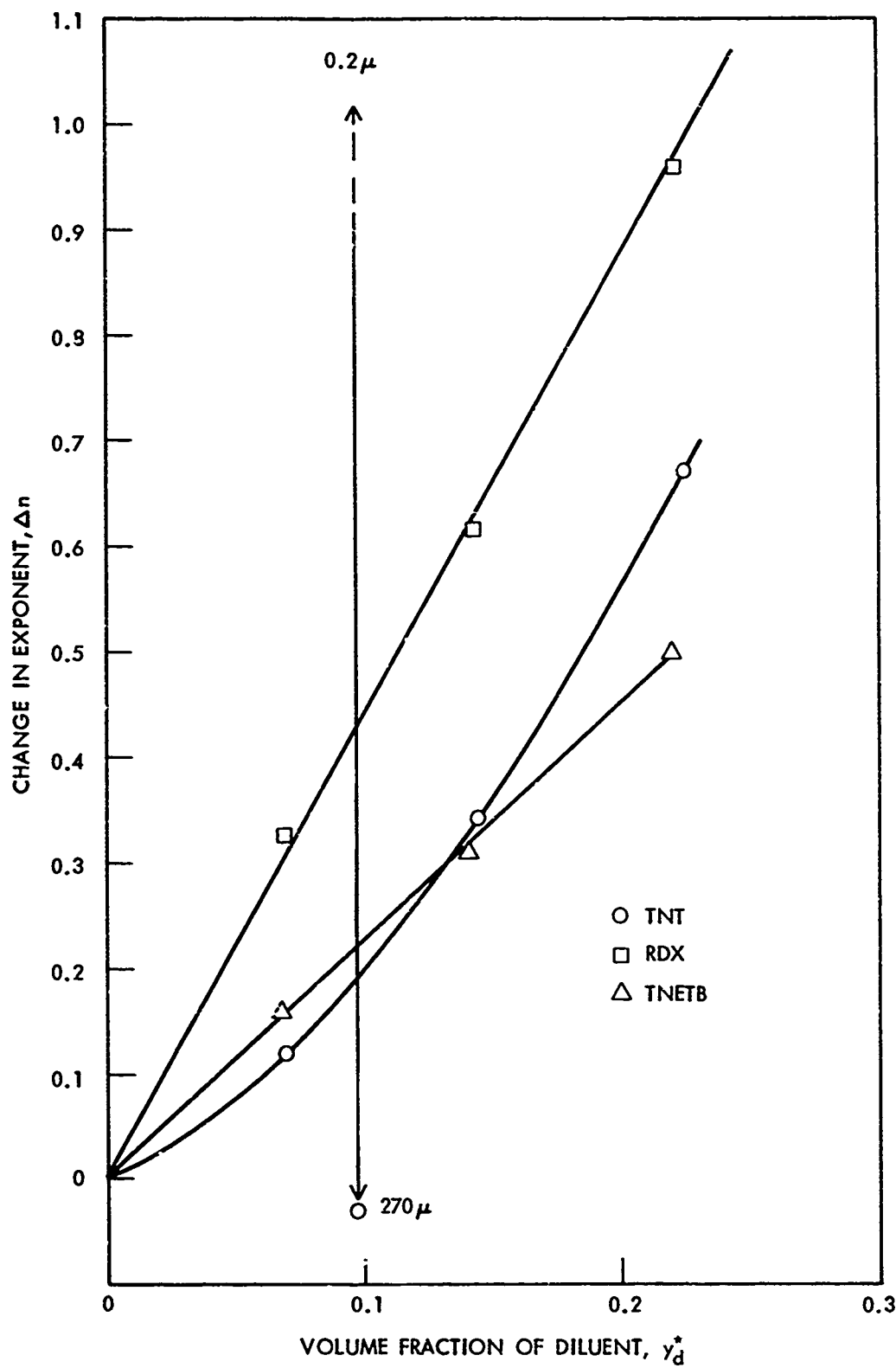
FIG. 7 CHANGE IN EXPONENT \Delta n EFFECTED BY DIFFERENT MATRICES IN HE/Al MIXTURES
