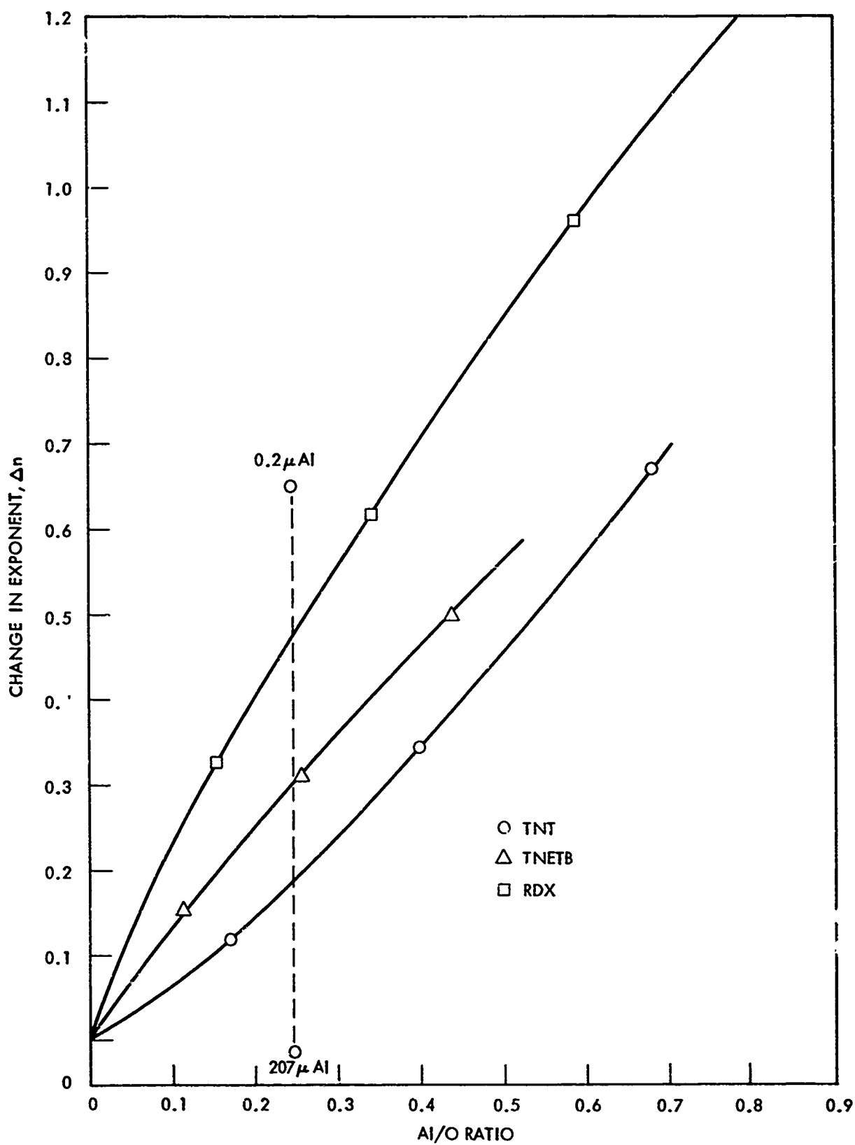
FIG. 8 CHANGE IN EXPONENT \Delta n AS FUNCTION OF Al/O RATIO OF VARIOUS HE/Al MIXTURES
