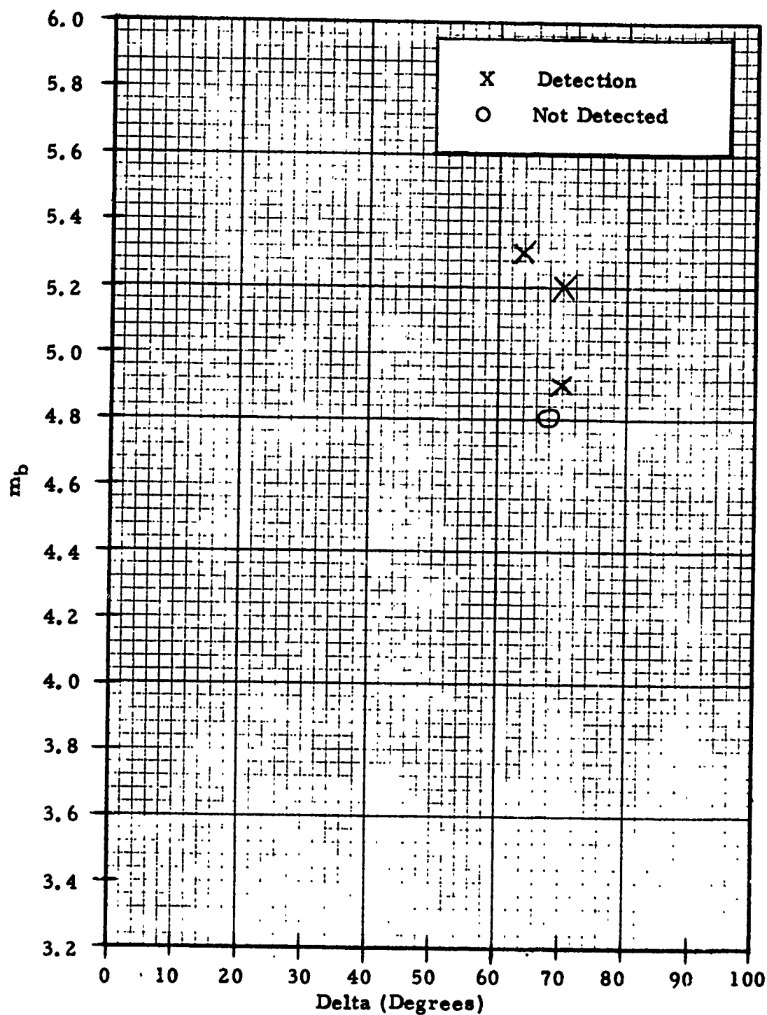
FIGURE IV-1 AUSTRALIA EVENT DETECTION vs. DELTA
