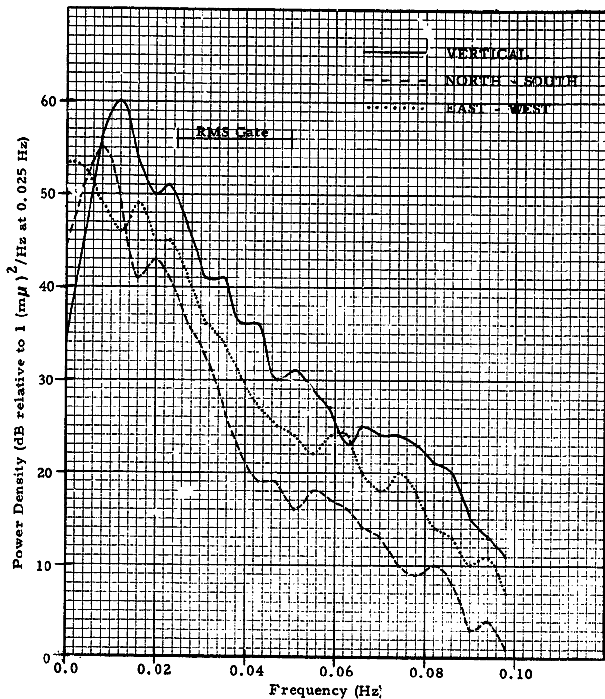
FIGURE III-4 ALASKA (HIGH 20-40 sec RMS LEVEL) NOISE POWER DENSITY SPECTRA 10/31/71 (DAY 304) 12:00:00
