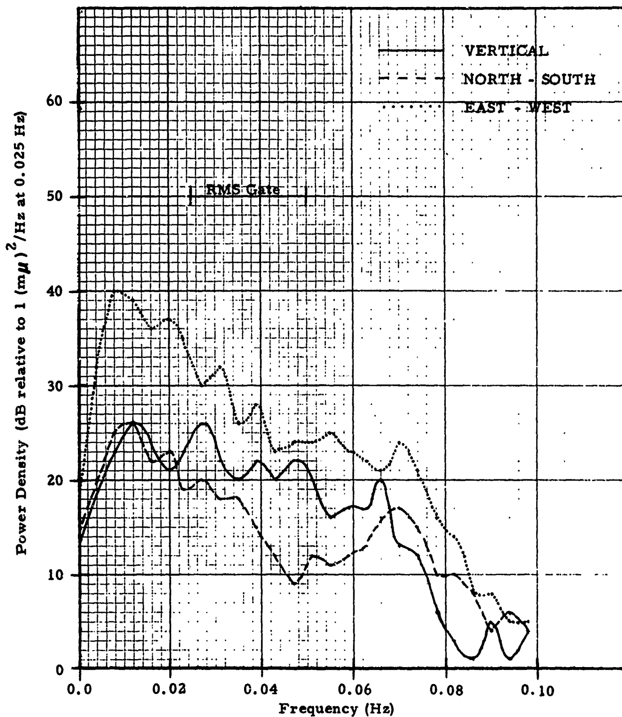
FIGURE III-6 ISRAEL NOISE POWER DENSITY SPECTRA 5/23/71 23:30:00
