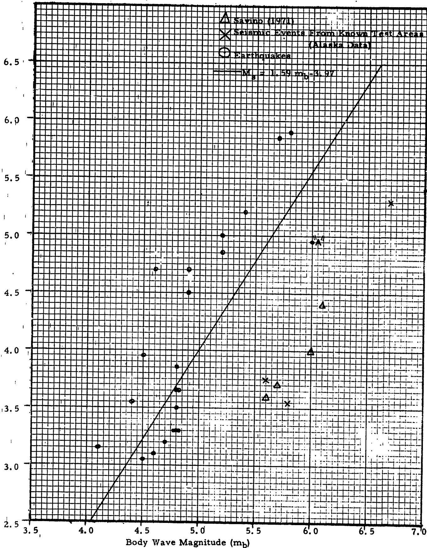
FIGURE IV-13 ISRAEL M_s - m_b
