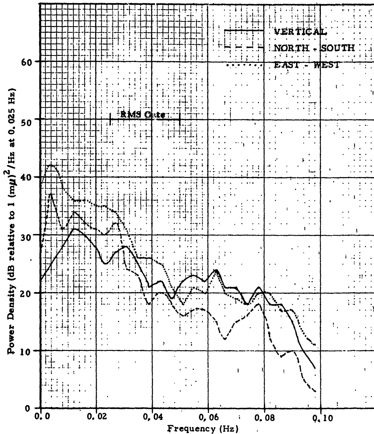
FIGURE III-7. NORWAY NOISE POWER DENSITY SPECTRA 09/20/71 01:00:00
