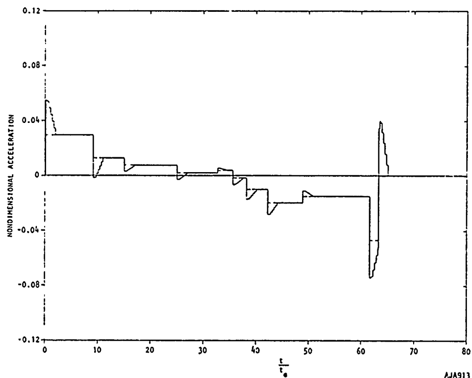
(c) FREE-SURFACE RADIAL ACCELERATION AT 0^\circ
