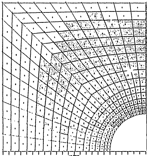
(g) LAST STEP OF GROUND SHOCK LOADING-- FOURTH ATTACK
