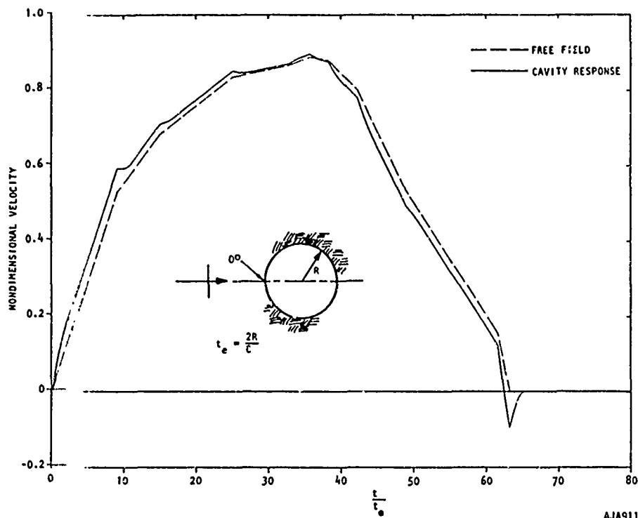
(a) FREE-SURFACE RADIAL VELOCITY AT 0^\circ
