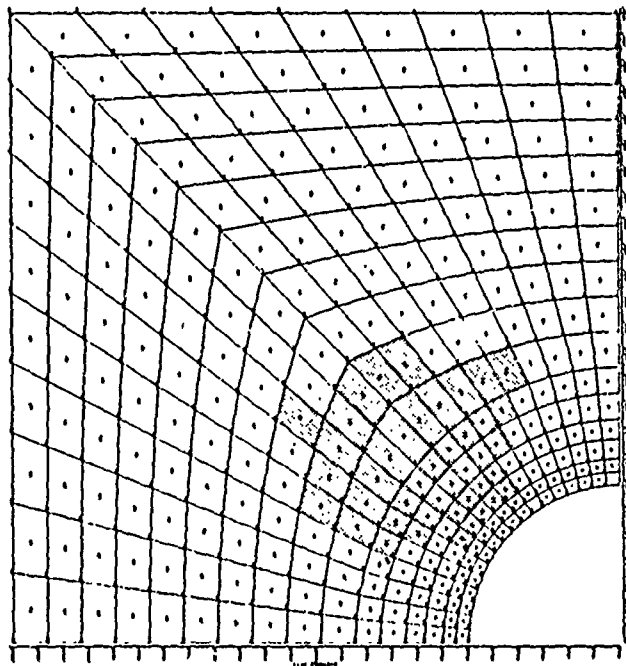
(b) FIRST STEP OF GROUND SHOCK LOADING-- FIRST ATTACK
