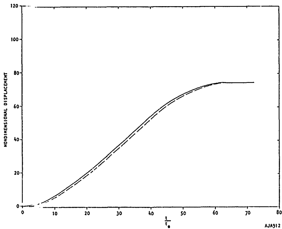
(b) FREE-SURFACE RADIAL DISPLACEMENT AT 0^\circ
