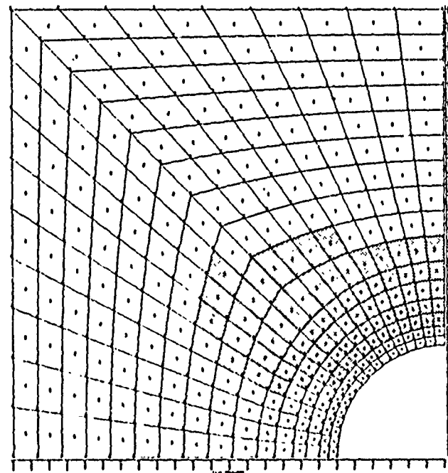
(a) LAST STEP OF OVERBURDEN LOADING
