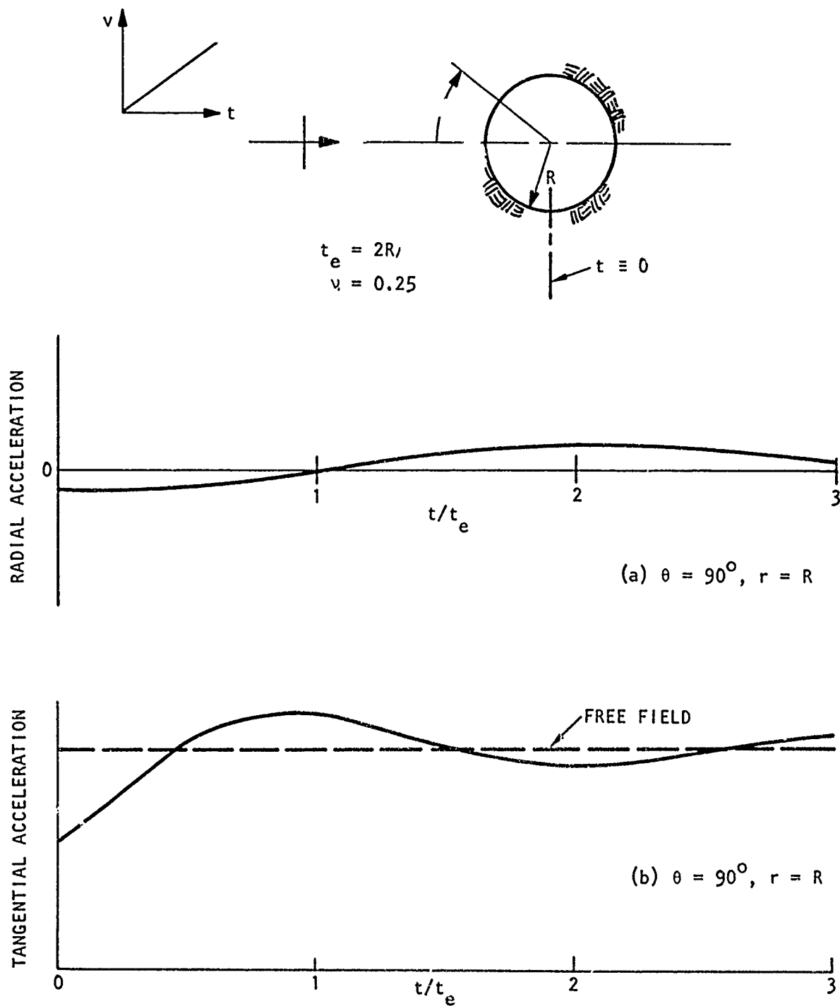
FIGURE 2-5. TRANSIENT ACCELERATION RESPONSE ON SHADOW SIDE OF UNLINED CAVITY
