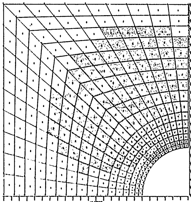
(e) LAST STEP OF GROUND SHOCK LOADING-- SECOND ATTACK
