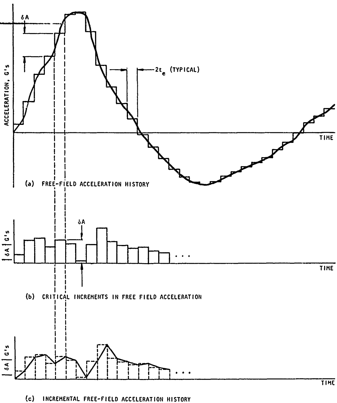
FIGURE 2-8. CONSTRUCTION OF INCREMENTAL FREE FIELD ACCELERATION HISTORY
