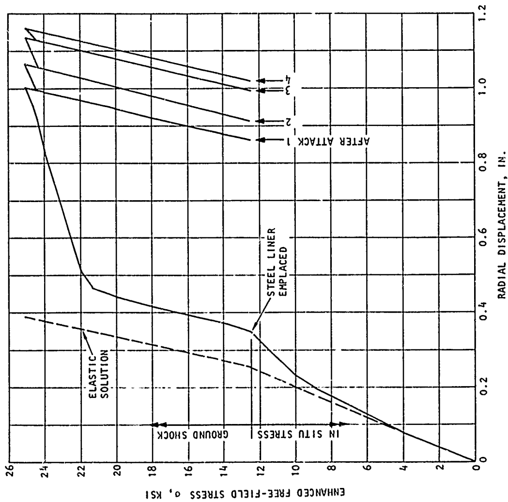
FIGURE 3-8. RADIAL DISPLACEMENT OF PENETRATION CROWN
