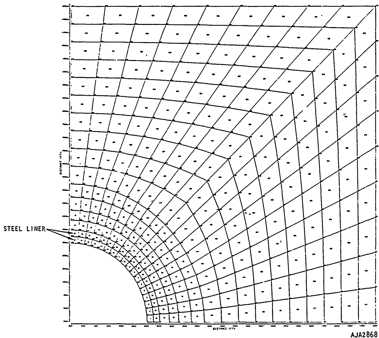
FIGURE 3-6. FINITE ELEMENT MESH OF PENETRATION (SEE FIGURE 3-1) (b))
