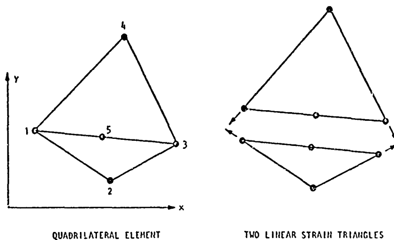
FIGURE C-1. LINEAR STRAIN QUADRILATERAL ELEMENT (WILSON, REFERENCE C-1)
