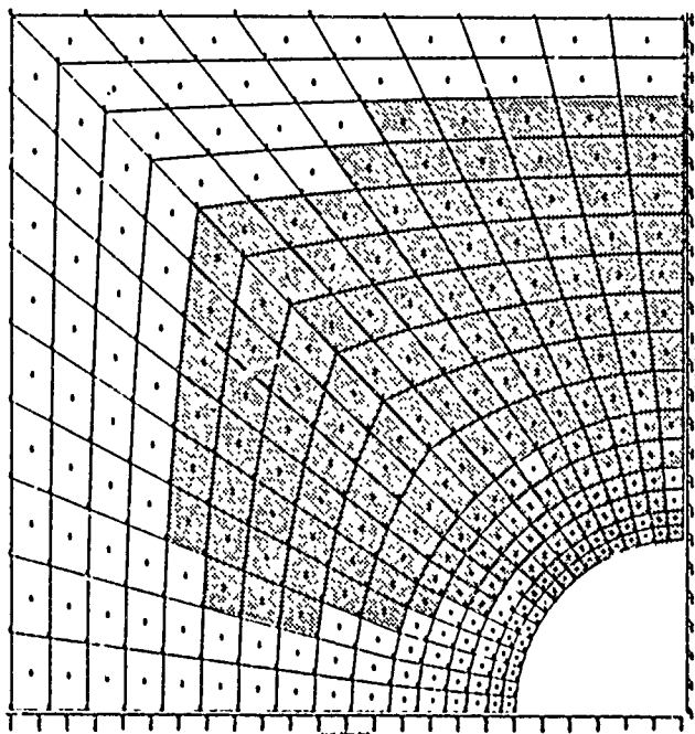
(f) LAST STEP OF GROUND SHOCK LOADING-- THIRD ATTACK
