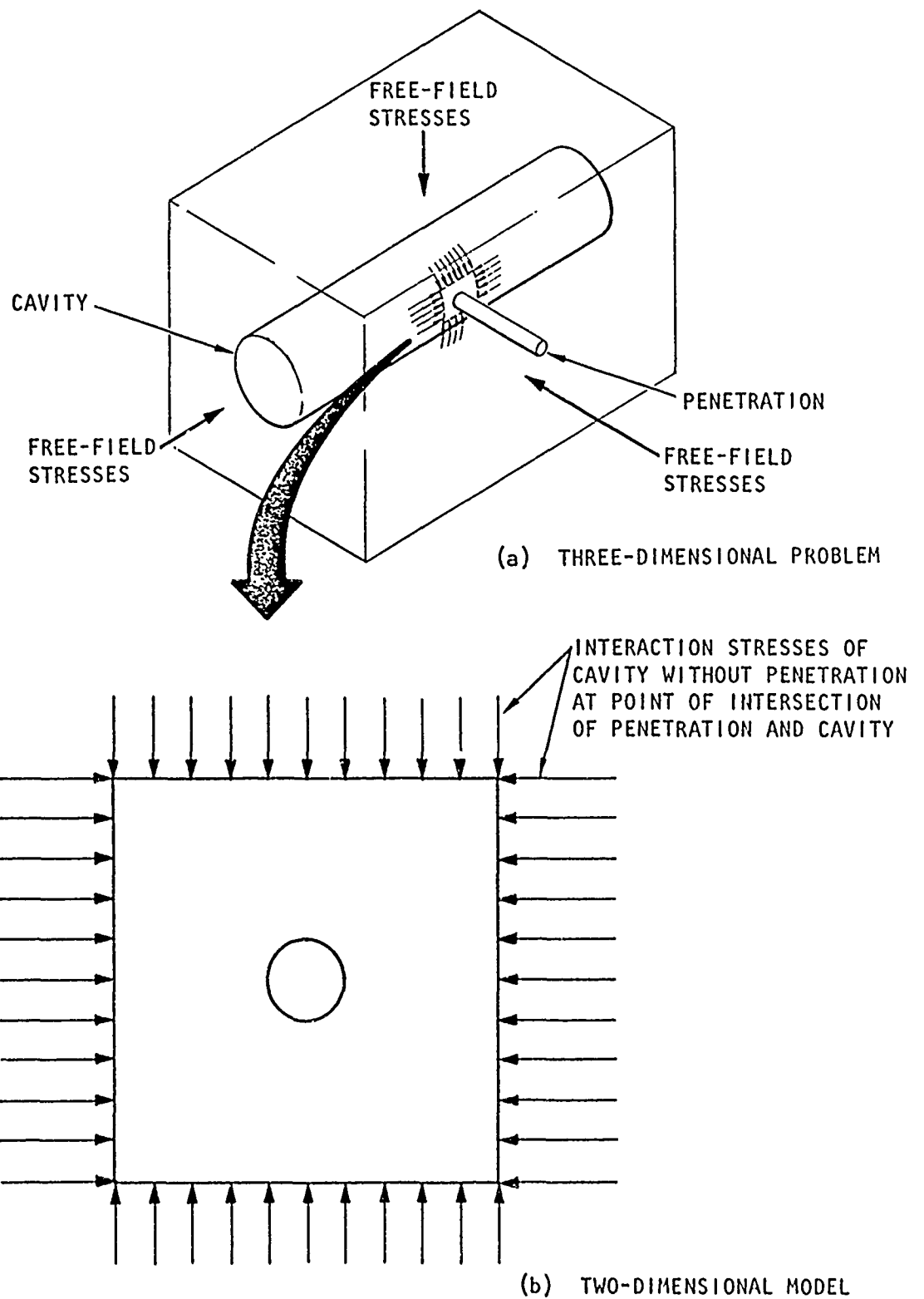
FIGURE 3-1. IDEALIZATION OF PENETRATION PROBLEM
