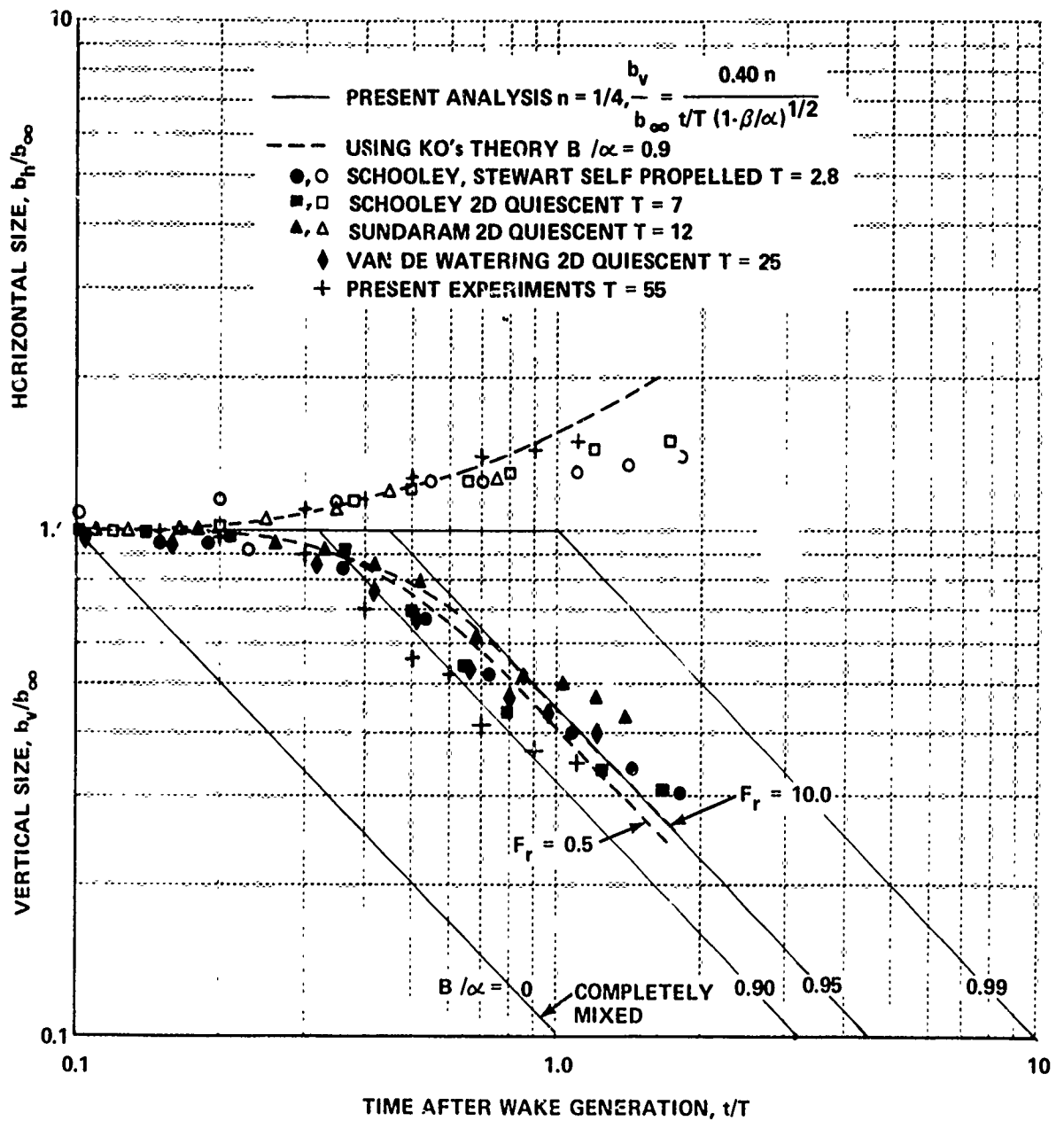
Figure 10 CORRELATION OF WAKE DIMENSIONS DURING COLLAPSE
