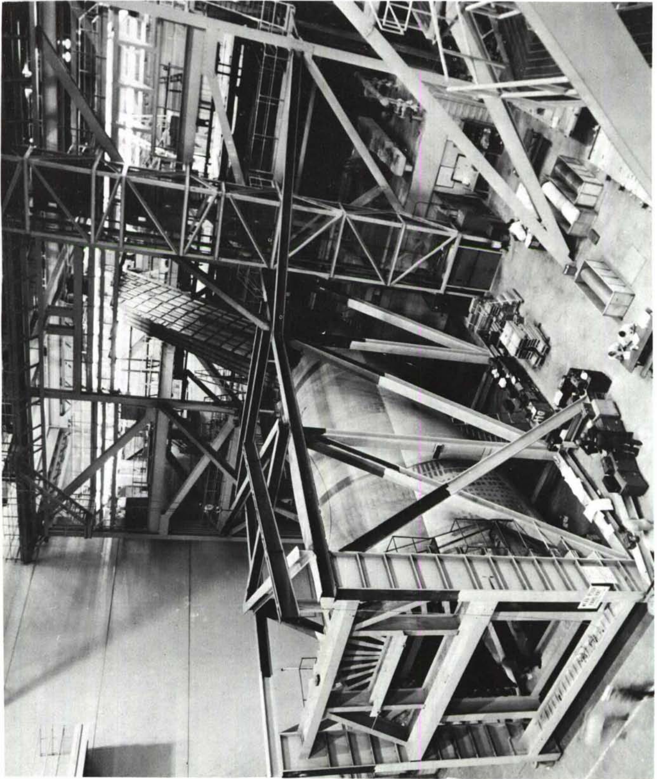
FIGURE 33. C-5A AFT FUSELAGE-EMPENNAGE IN TEST FIXTURE PRIOR TO INSTALLATION OF JACKS AND LINKAGE
