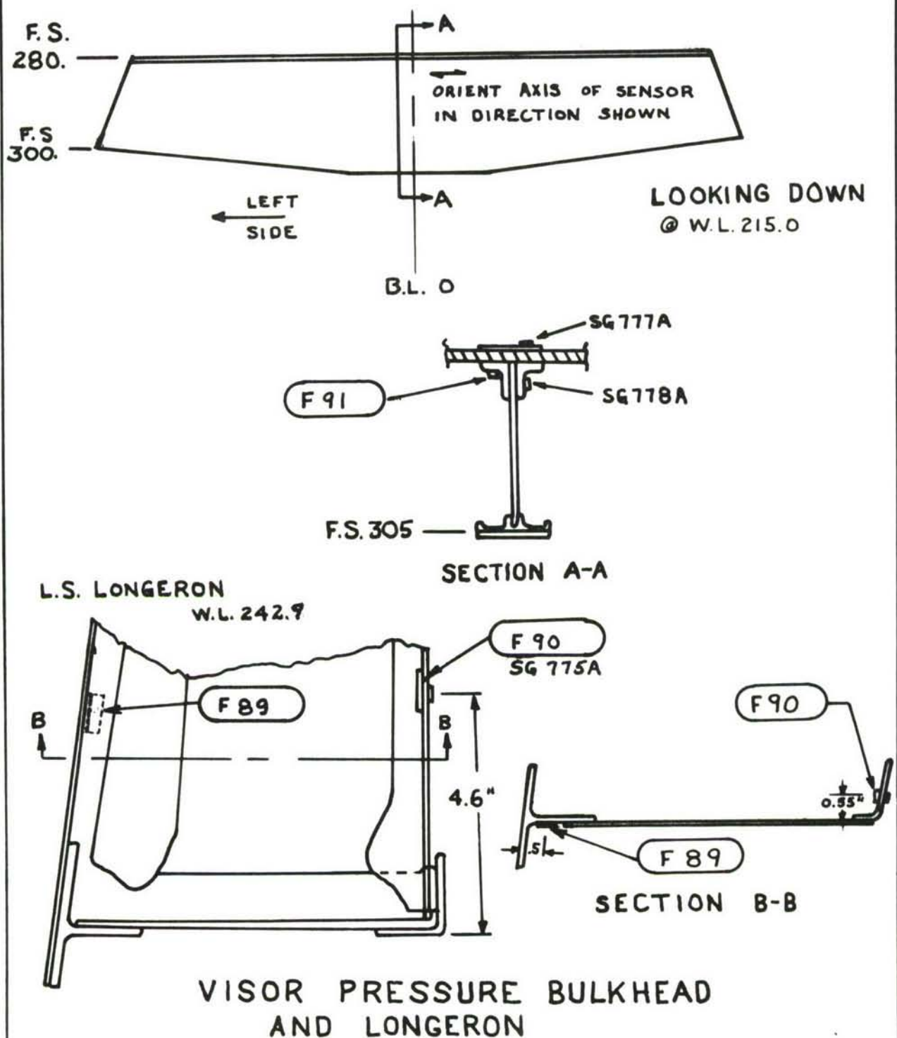
FIGURE 98. SENSOR LOCATIONS ON THE NOSE VISOR
