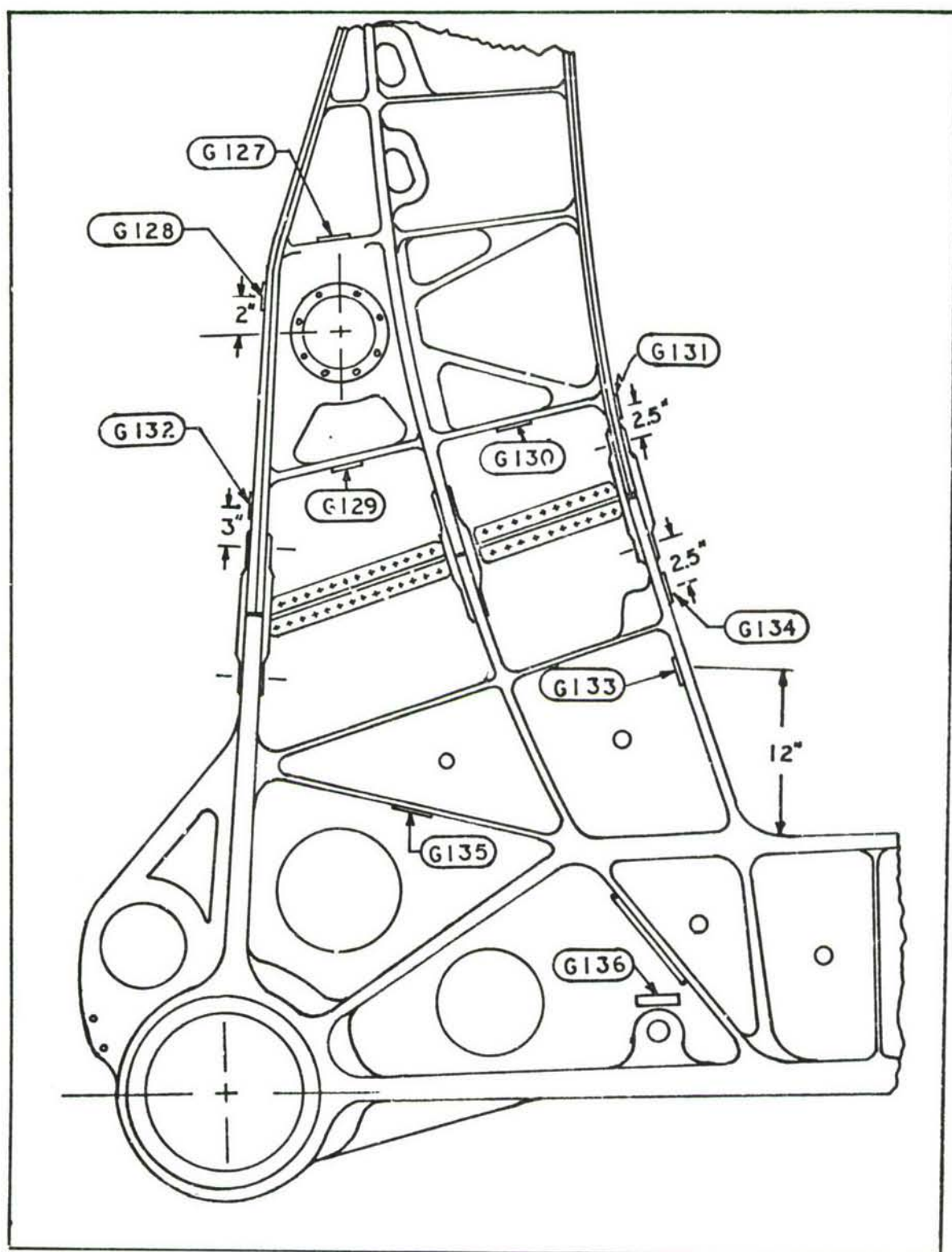
FIGURE 28. PARTIAL MAIN FRAME F.S. 1603
