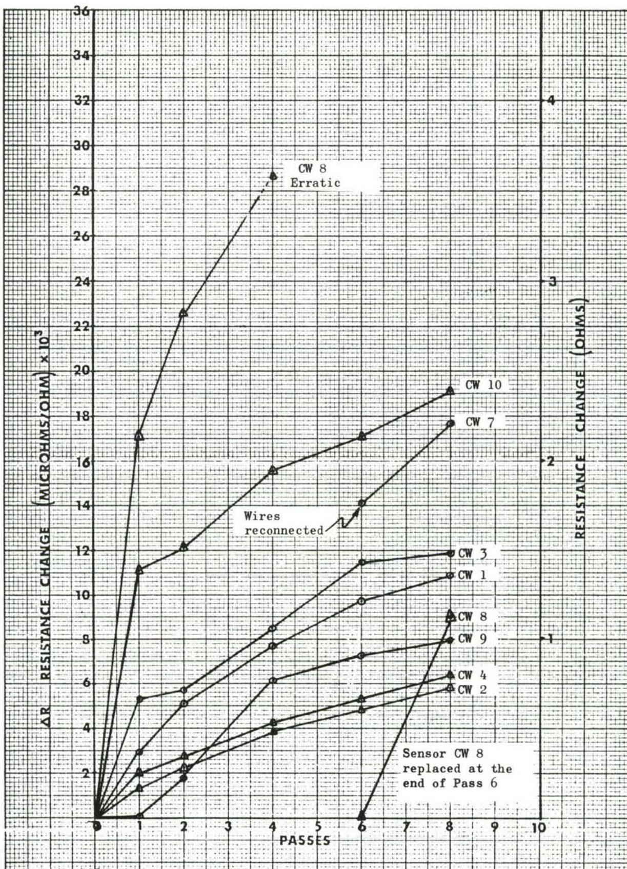
FIGURE 106. SENSOR RESPONSE ON THE CENTER WING AT B.L. 101
