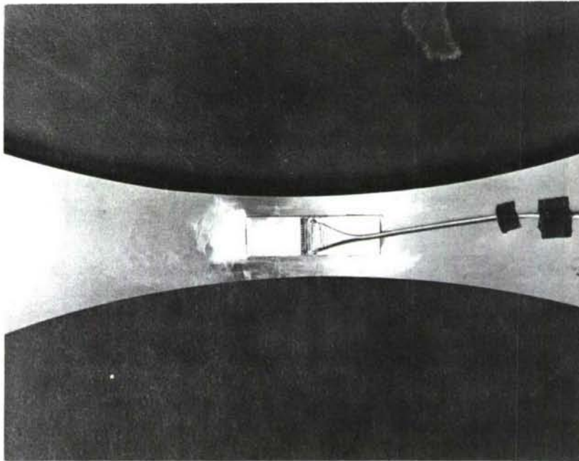
FIGURE 9. VIEW OF SAP204DA-STE SENSOR INSTALLED ON TEST COUPON
