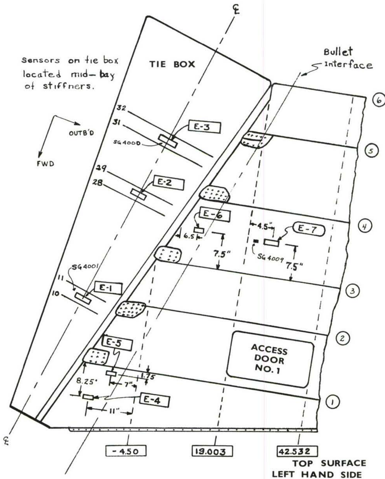
FIGURE 54. HORIZONTAL STABILIZER
