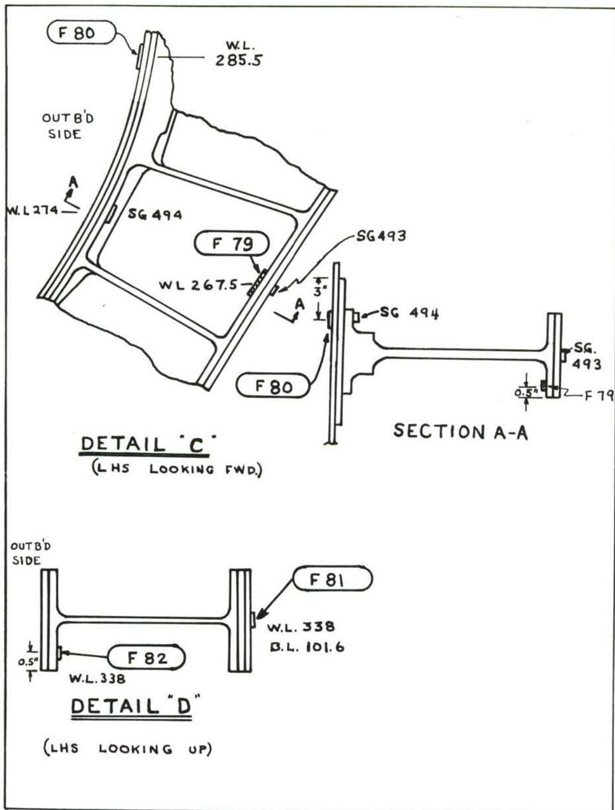
FIGURE 92. SENSOR LOCATION DETAILS ON THE FUSELAGE MAIN FRAME AT F.S. 1106
