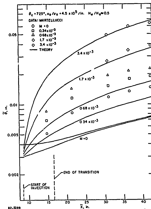
Figure 35 MOMENTUM THICKNESS DISTRIBUTIONS ON A SHARP CONE AT MACH 8
