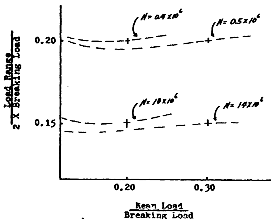
Figure 12 AXIAL FATIGUE LIFE OF \frac{1}{2} -IN. DIA., 6 x 25, IPS, WIRE ROPE AS A FUNCTION OF MEAN LOAD AND LOAD AMPLITUDE
