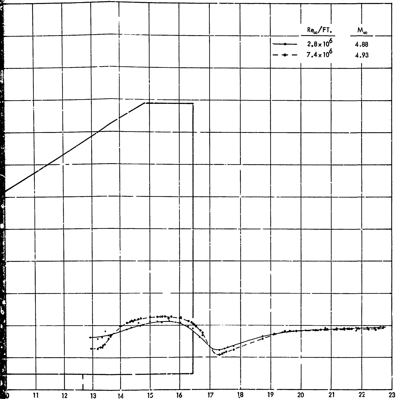
FIG. 16C 60° SWEEPED FIN WITH 0.25 INCH CLEARANCE GAP
