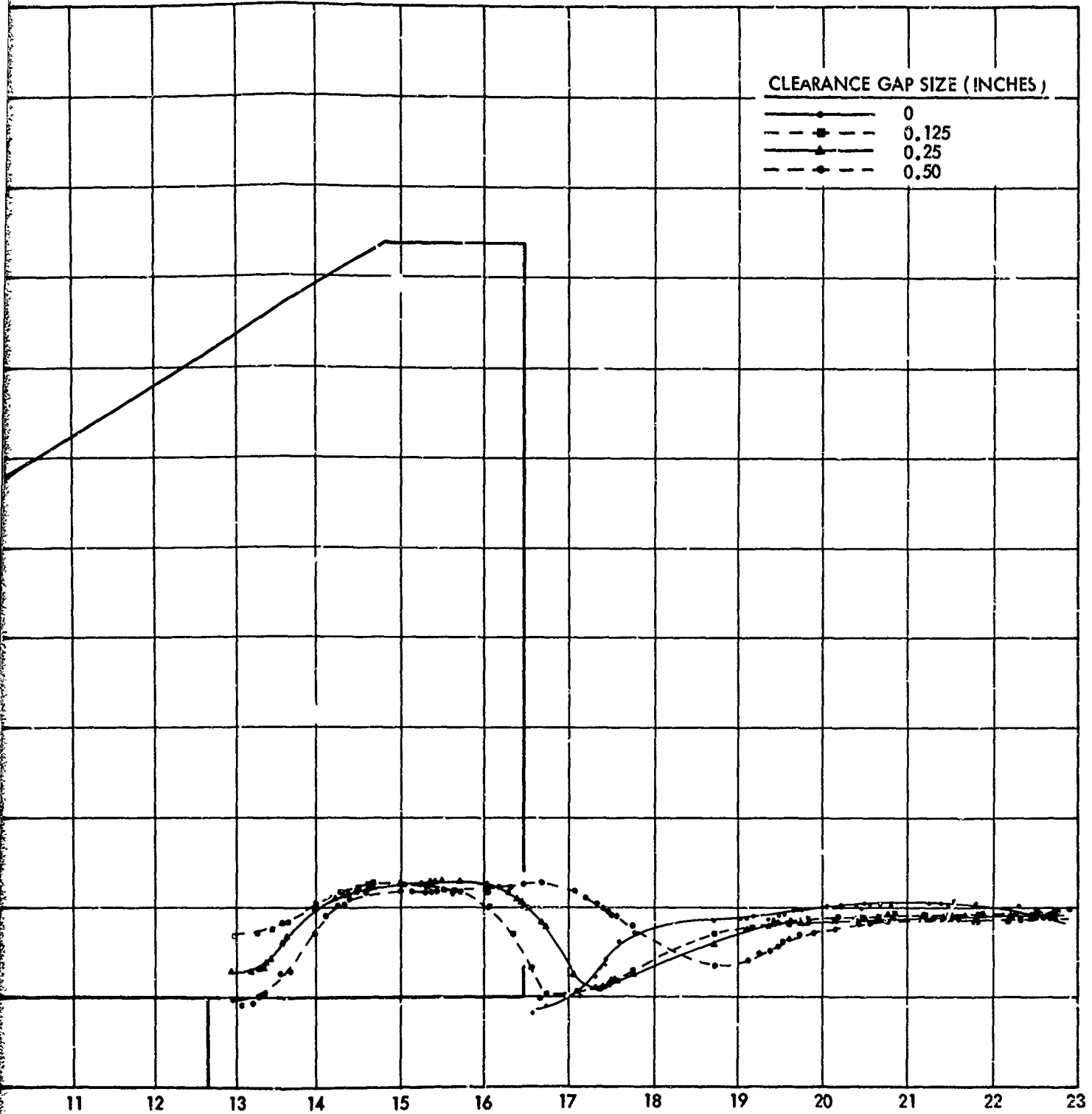
FIG. 17 FLAT PLAT PRESSURE DISTRIBUTION FOR VARYING CLEARANCE GAPS ON A 60° SWEEP FIN
