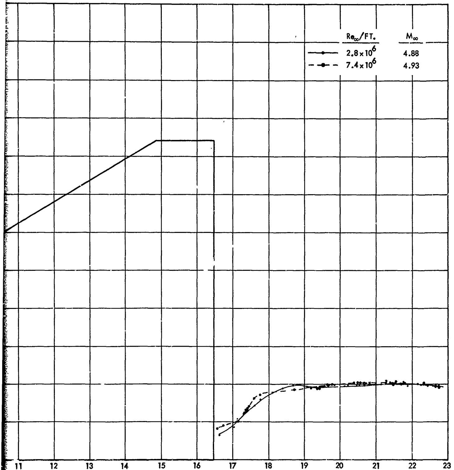
FIG. 16A FLAT PLATE PRESSURE DISTRIBUTION PRODUCED BY A 60° SWEEP FIN
