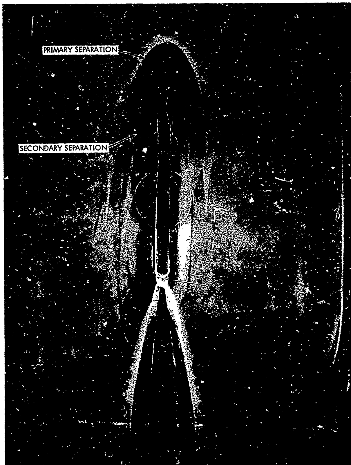
FIG. 27a OIL PATTERN ON THE FLAT PLATE FOR A 60° SWEEP FIN
