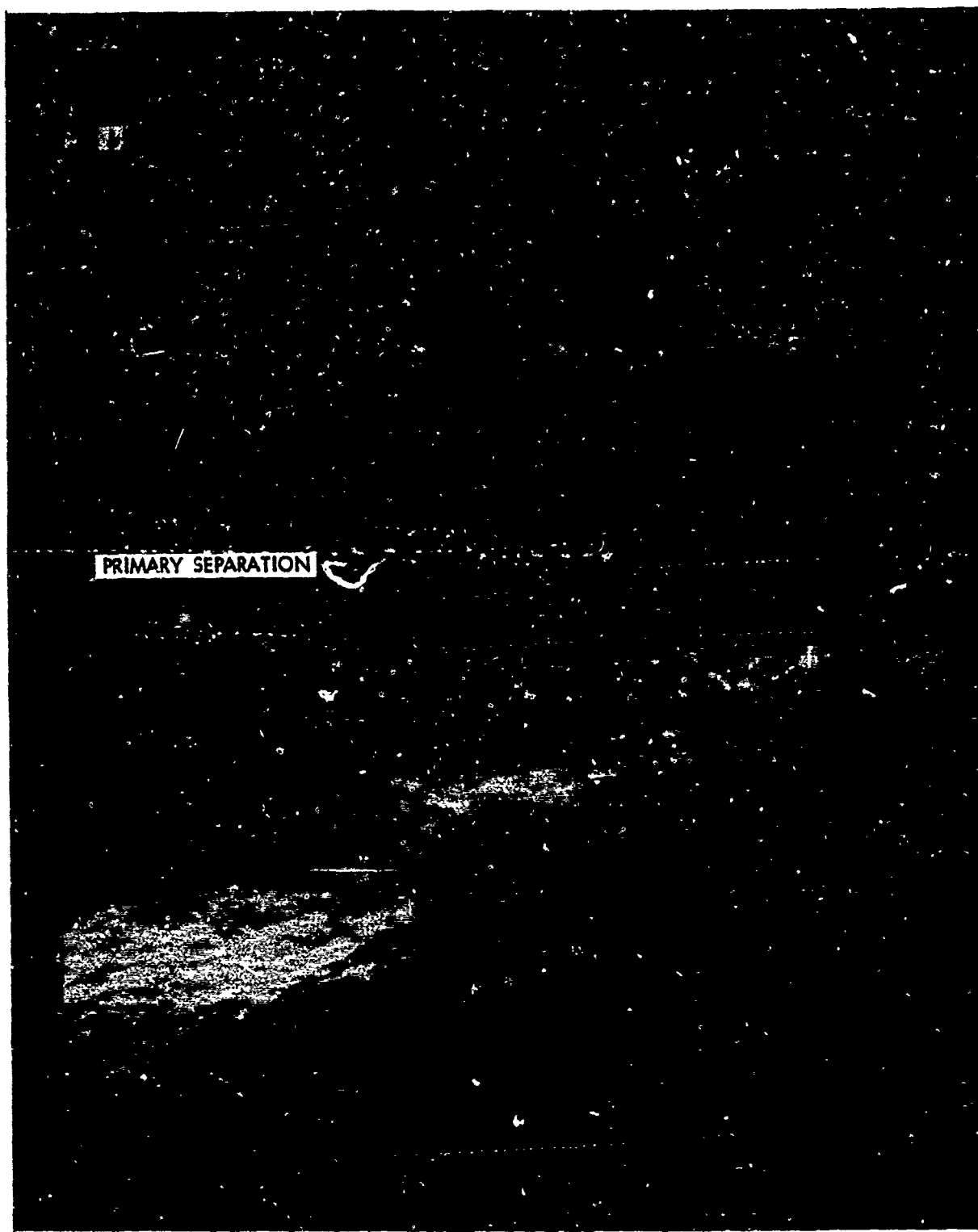
FIG. 34a SCHLIEREN PHOTOGRAPHS OF THE FLOW FIELD UPSTREAM OF A 60° SWEPT, CYLINDRICALLY BLUNT FIN
