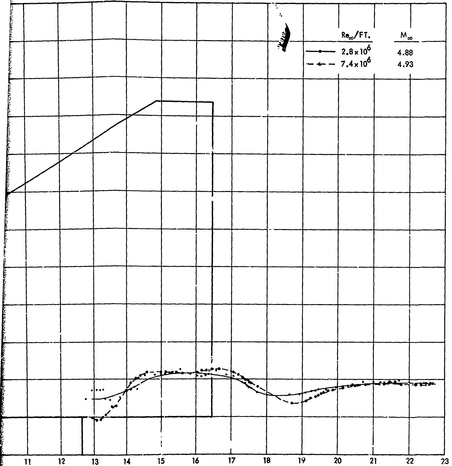
FIG. 16D 60^{\circ} SWEPT FIN WITH 0.50 INCH CLEARANCE GAP
