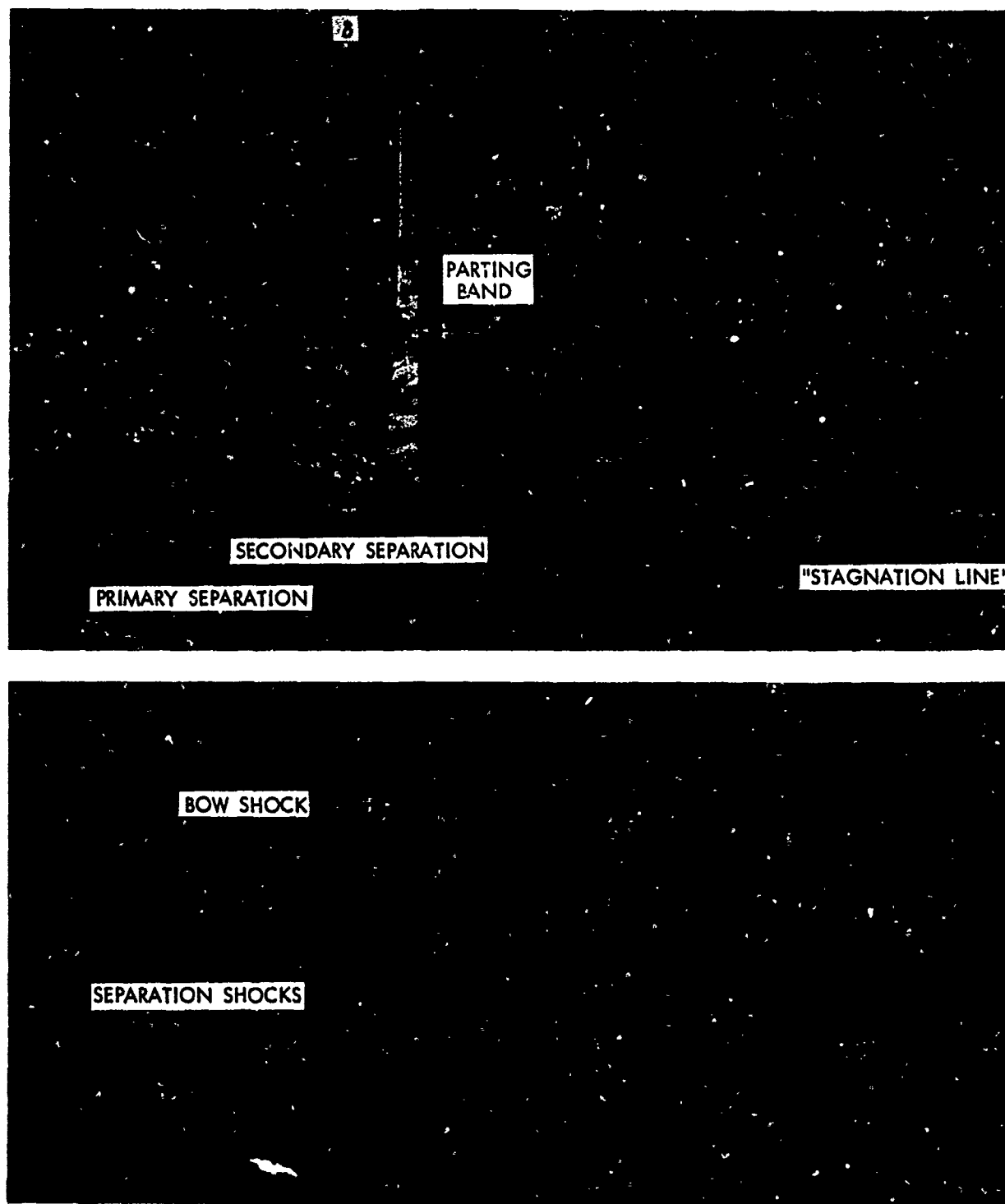
FIG. 33a SCHLIEREN PHOTOGRAPHS OF THE FLOW FIELD UPSTREAM OF AN CYLINDRICALLY BLUNT FIN ( M_\infty = 4.93 Re_\infty/FT = 7.4 \times 10^6 )
