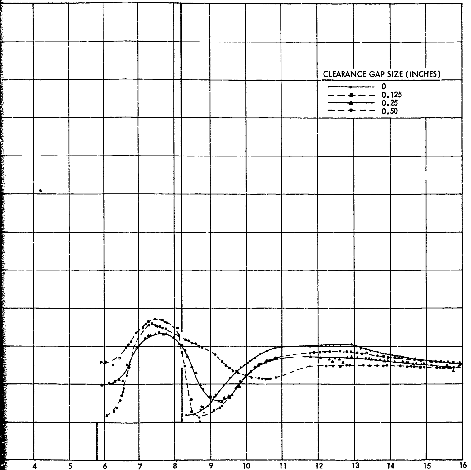
FIG. 13 FLAT PLATE PRESSURE DISTRIBUTION FOR VARYING CLEARANCE GAPS OF AN UNSWEPT FIN
