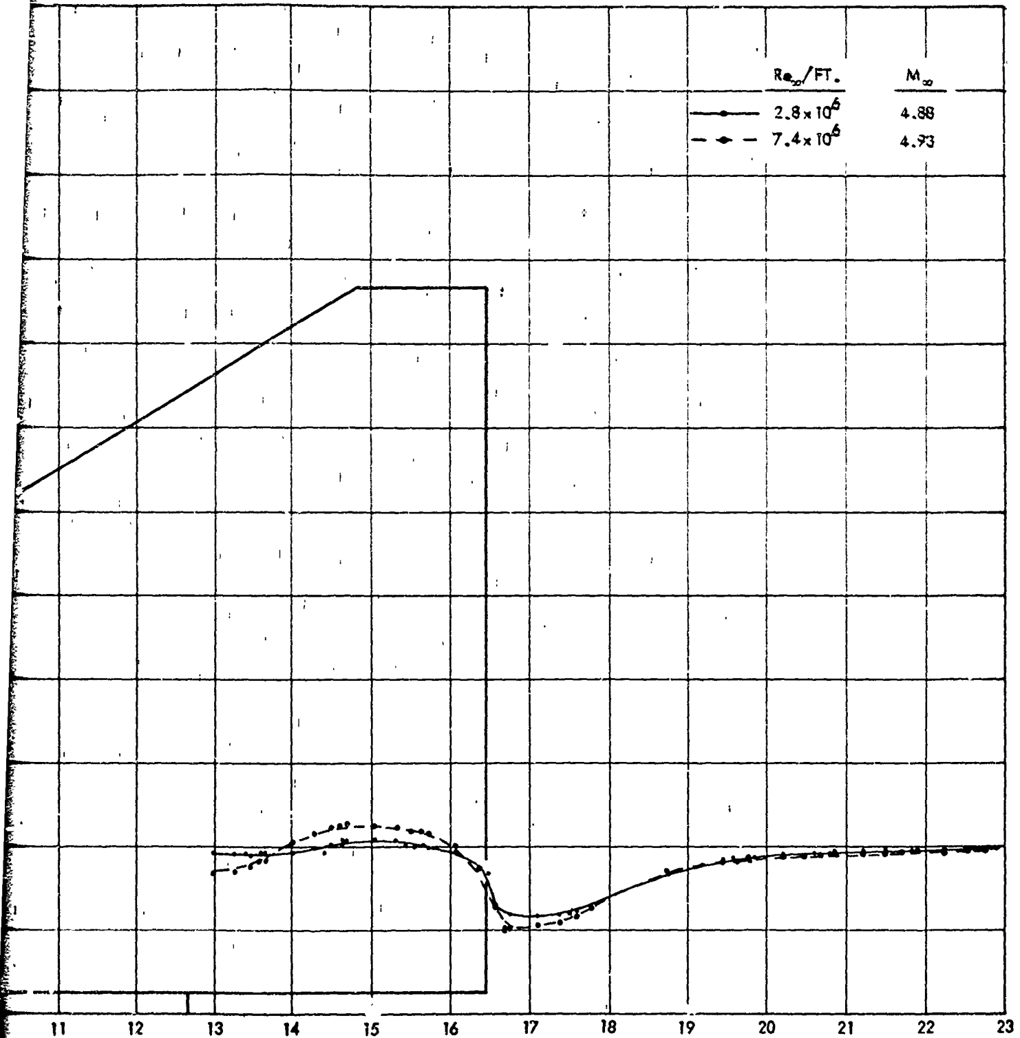
FIG. 16 B 60° SWEPT FIN WITH 0.125 INCH CLEARANCE GAP
